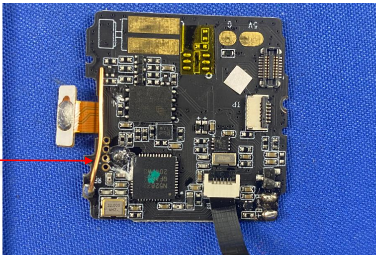
Bluetooth Antenna
