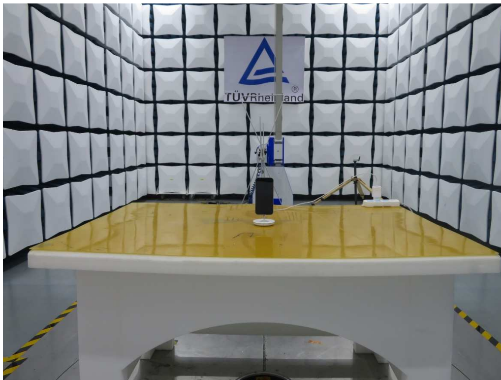
Photograph 2: Set-up photo for Radiated Spurious Emission, 30MHz - 1GHz For Apple Magsafe:
