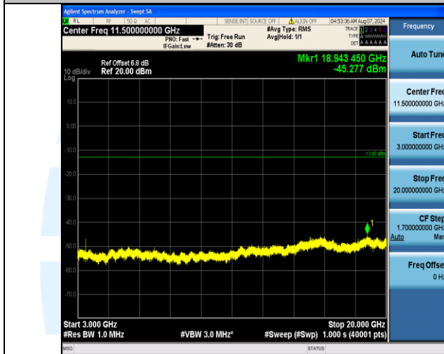
Band4_5MHz_16QAM_19975_1RB#24_3000~20000_3000~20000
