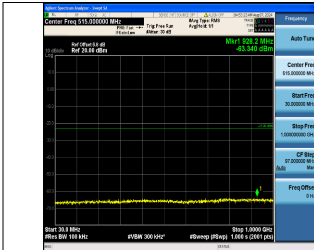
Band4_5MHz_16QAM_19975_1RB#24_30~1000_30~1000
