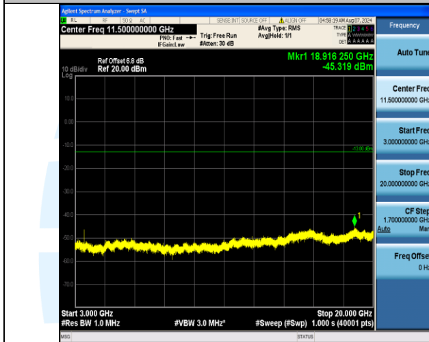
Band4_5MHz_16QAM_20375_1RB#24_3000~20000_3000~20000
