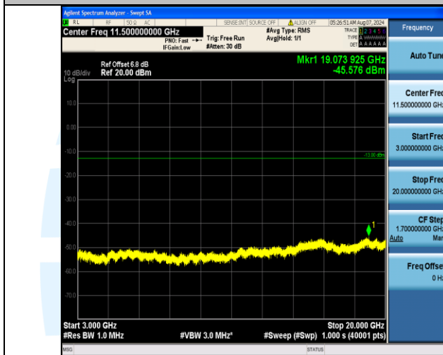
Band4_10MHz_QPSK_20000_50RB#0_3000~20000_3000~20000
