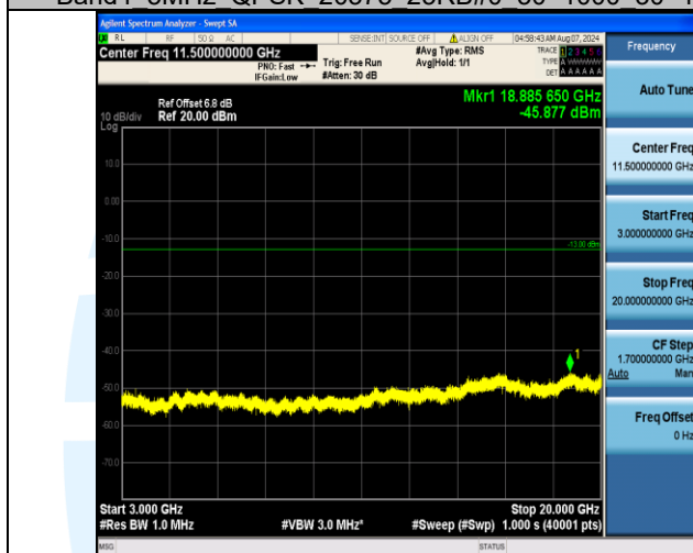
Band4_5MHz_QPSK_20375_25RB#0_3000~20000_3000~20000
