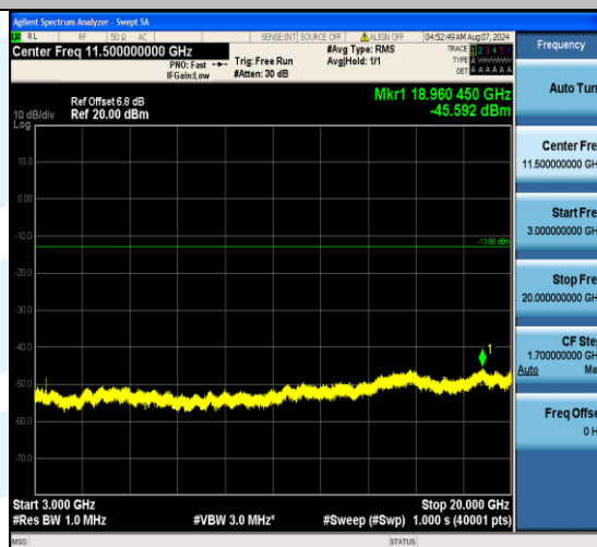
Band4_5MHz_16QAM_19975_1RB#0_3000~20000_3000~20000
