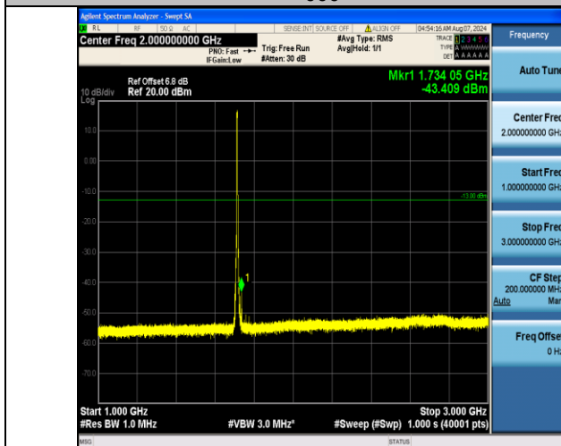
Band4_5MHz_16QAM_19975_25RB#0_1000~3000_1000~3000
