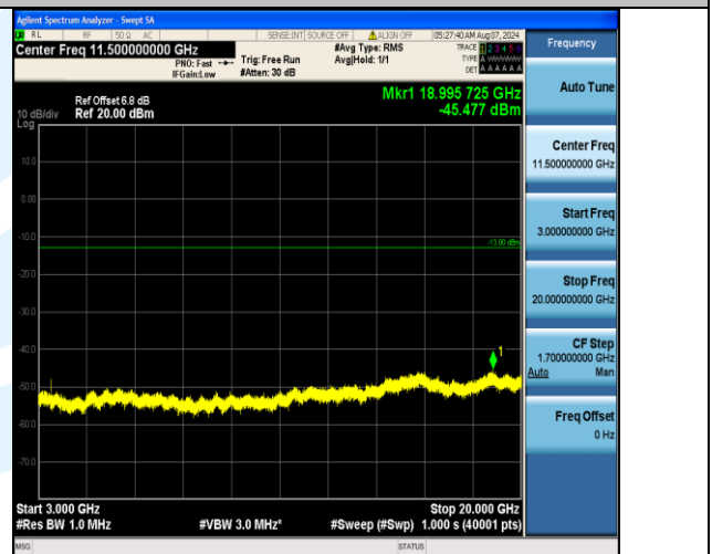
Band4_10MHz_QPSK_20175_1RB#0_3000~20000_3000~20000
