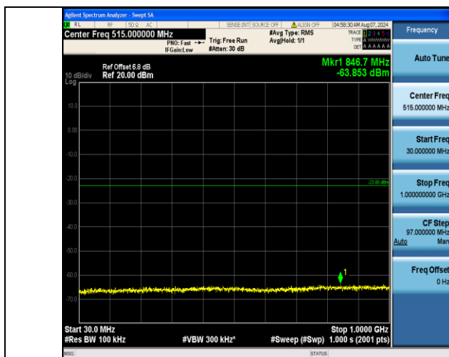
Band4 5MHz QPSK 20375 25RB#0 30~1000 30~1000
