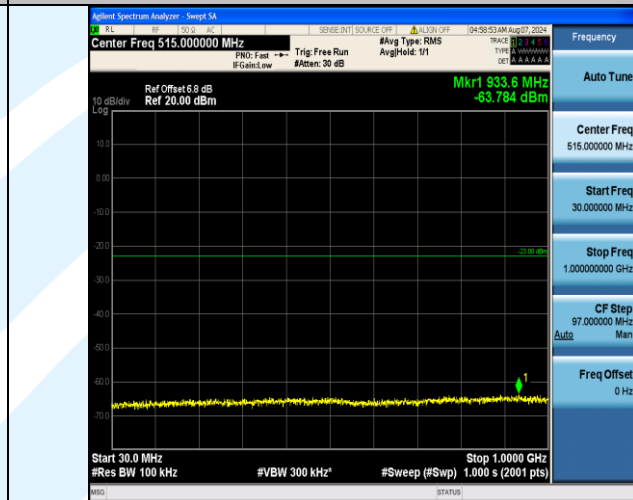
Band4_5MHz_16QAM_20375_25RB#0_30~1000_30~1000
