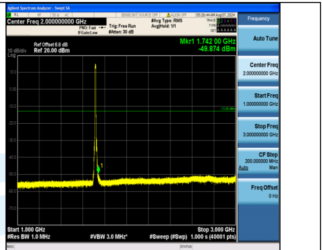
Band4_10MHz_QPSK_20000_50RB#0_1000~3000_1000~3000
