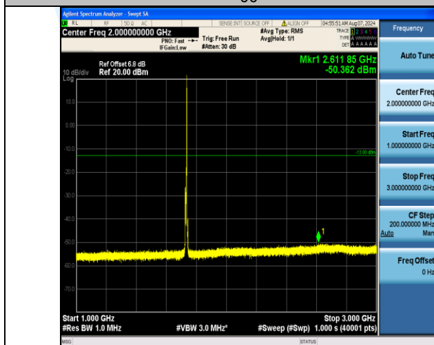
Band4_5MHz_16QAM_20175_1RB#24_1000~3000_1000~3000
