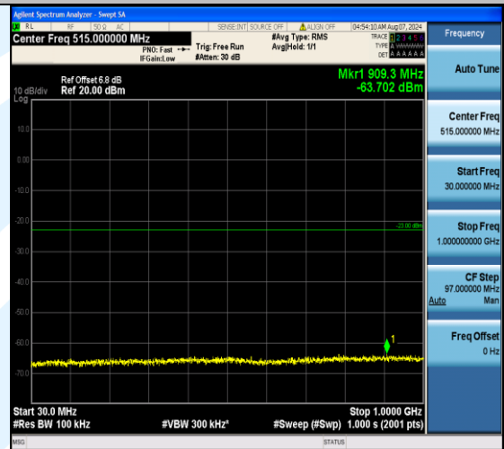
Band4_5MHz_16QAM_19975_25RB#0_30~1000_30~1000
