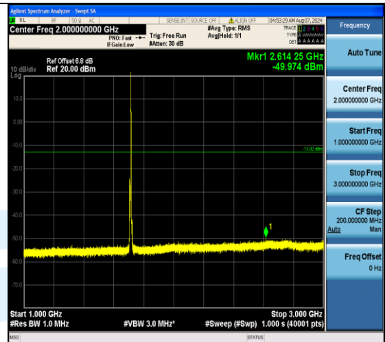
Band4_5MHz_16QAM_19975_1RB#24_1000~3000_1000~3000
