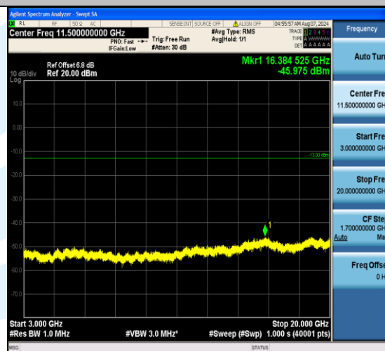
Band4_5MHz_16QAM_20175_1RB#24_3000~20000_3000~20000
