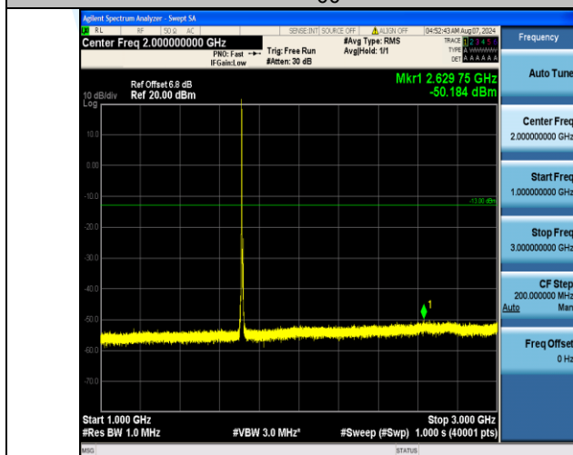
Band4_5MHz_16QAM_19975_1RB#0_1000~3000_1000~3000
