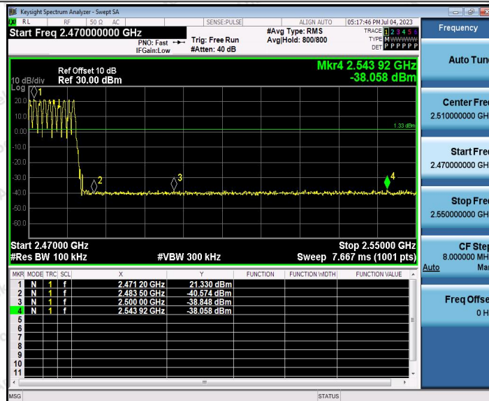
2.4G_Ant1_High_Hop_2479.4
