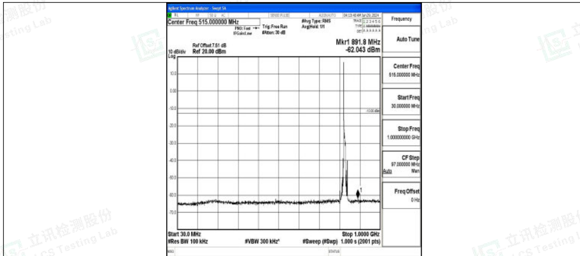
Band5_10MHz_QPSK_20450_1RB#0_30~1000_30~1000
