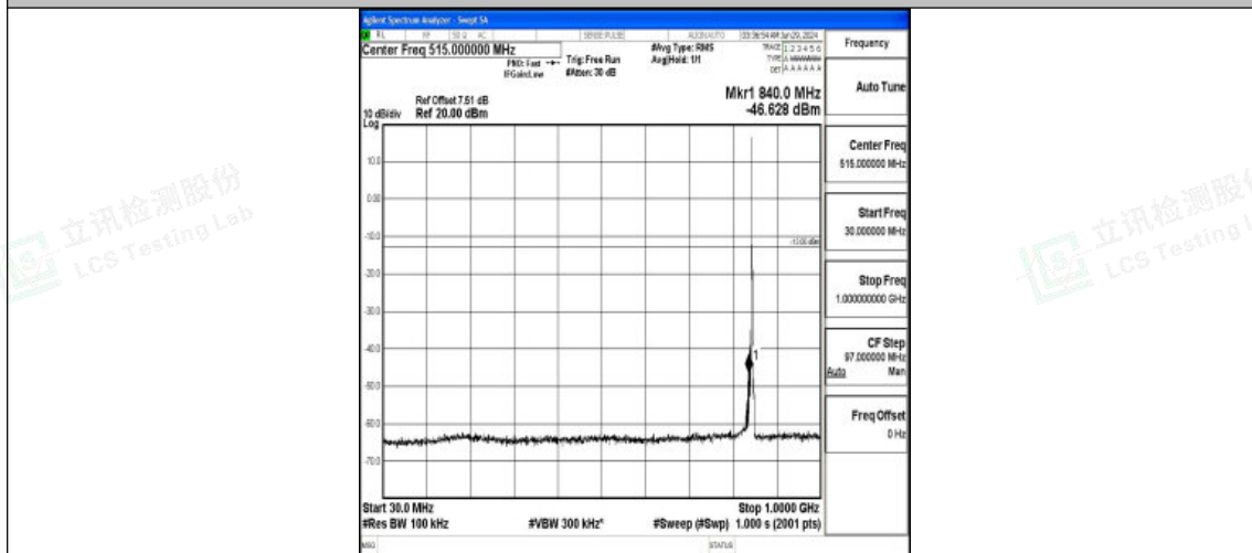
Band5_3MHz_QPSK_20635_1RB#0_30~1000_30~1000
