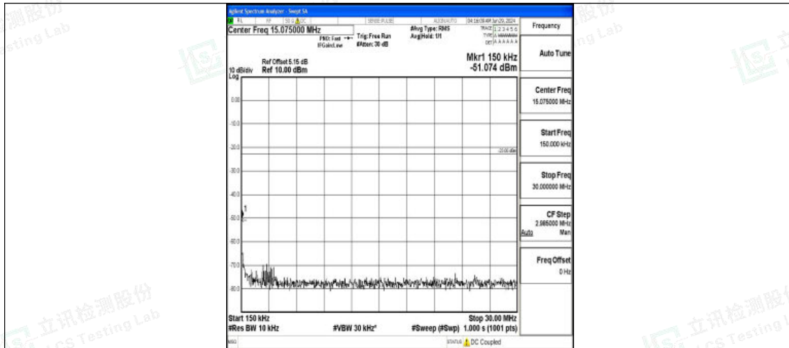
Band5_10MHz_16QAM_20600_1RB#0_0.15~30_0.15~30
