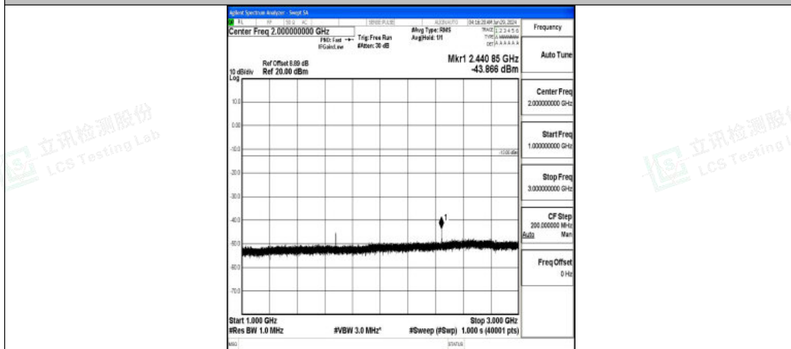
Band5_10MHz_16QAM_20600_1RB#0_1000~3000_1000~3000
