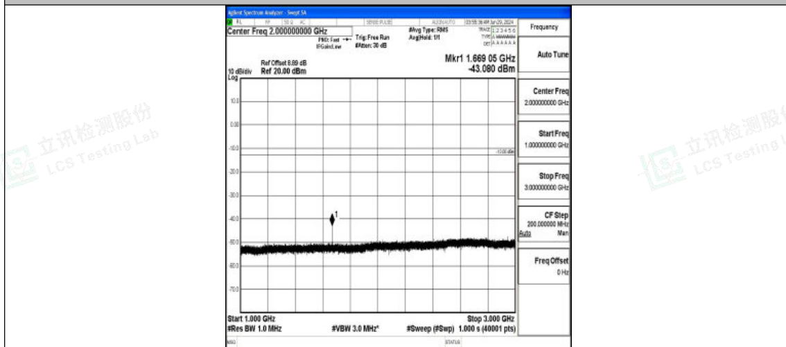
Band5_5MHz_QPSK_20525_1RB#0_1000~3000_1000~3000
