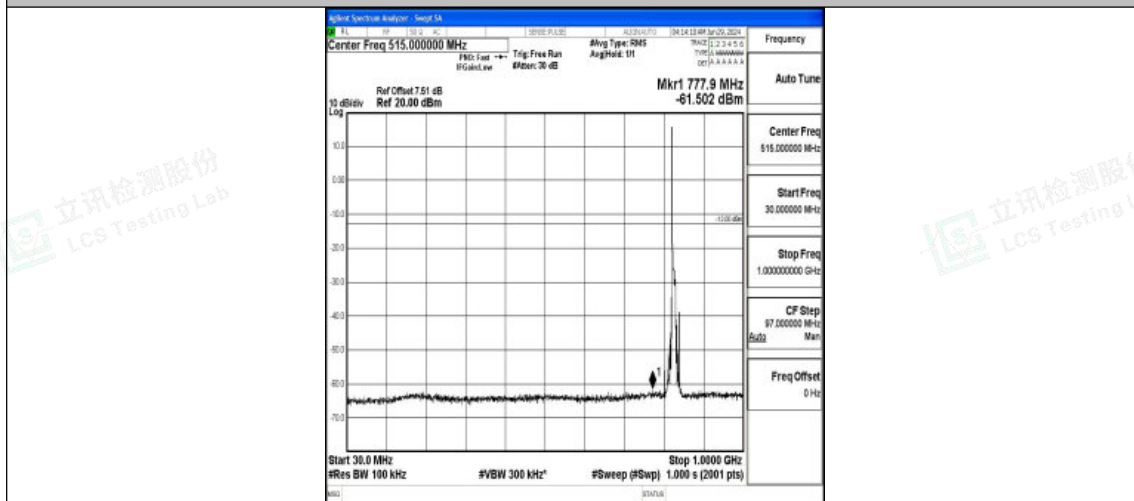
Band5_10MHz_16QAM_20450_1RB#0_30~1000_30~1000
