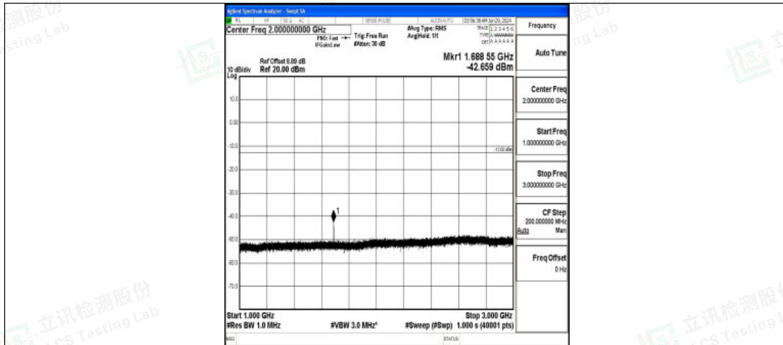
Band5_5MHz_QPSK_20625_1RB#0_1000~3000_1000~3000
