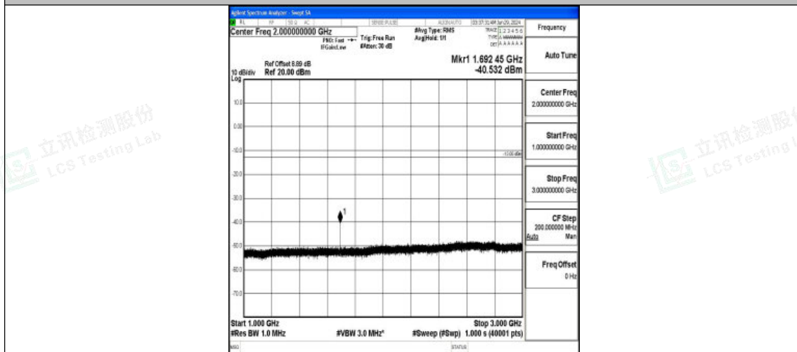
Band5_3MHz_16QAM_20635_1RB#0_1000~3000_1000~3000
