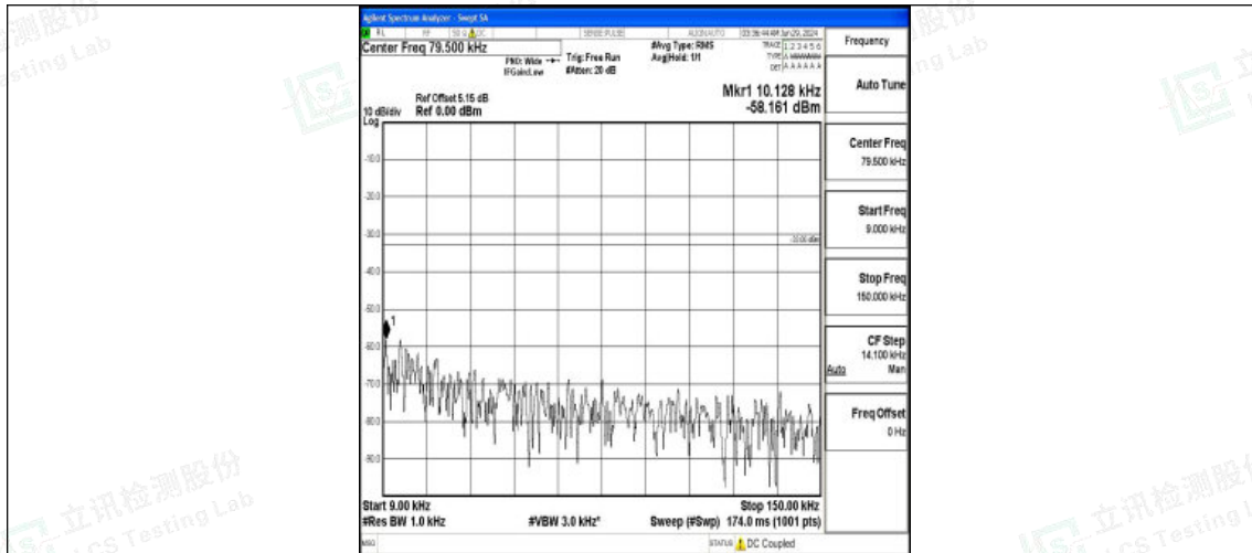
Band5_3MHz_QPSK_20635_1RB#0_0.009~0.15_0.009~0.15
