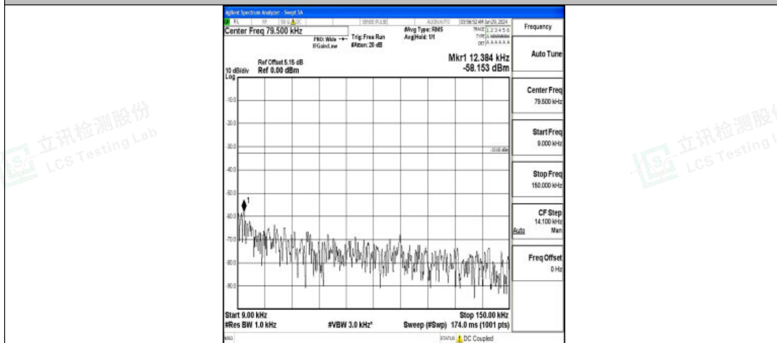
Band5_5MHz_16QAM_20625_1RB#0_0.009~0.15_0.009~0.15
