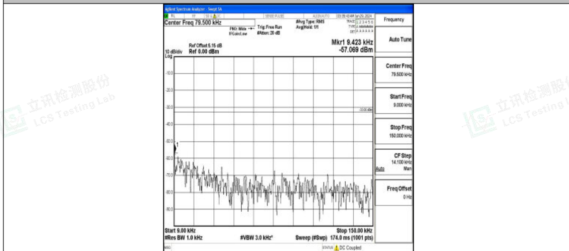
Band5_3MHz_QPSK_20525_1RB#0_0.009~0.15_0.009~0.15
