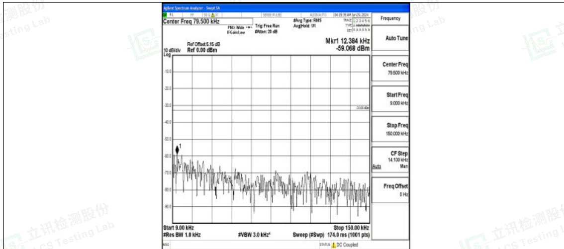
Band5_10MHz_QPSK_20600_1RB#0_0.009~0.15_0.009~0.15
