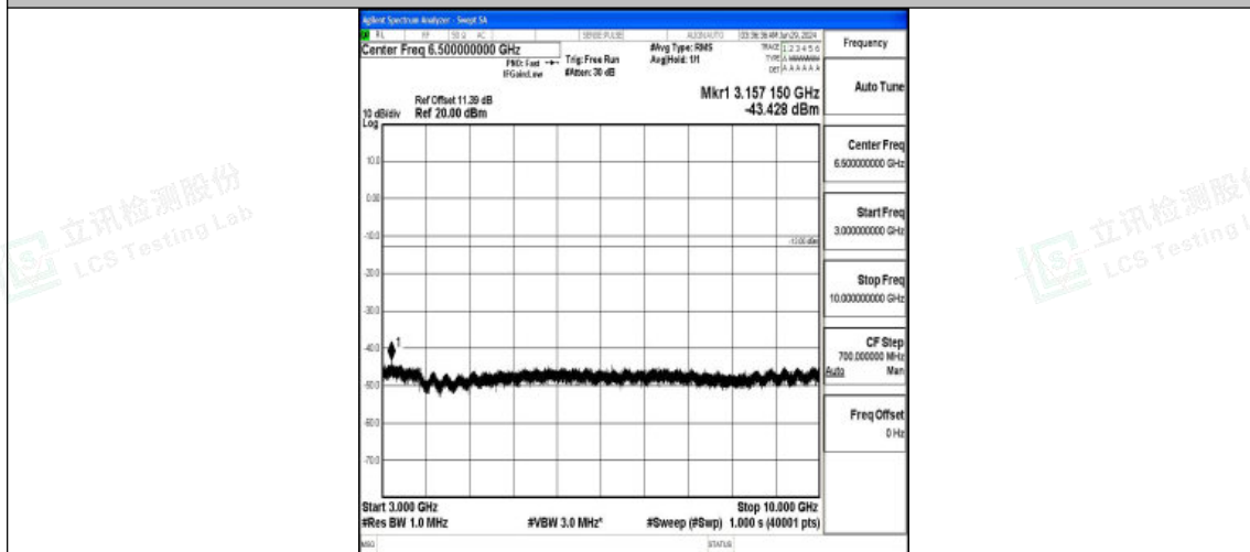
Band5_3MHz_16QAM_20525_1RB#0_3000~10000_3000~10000
