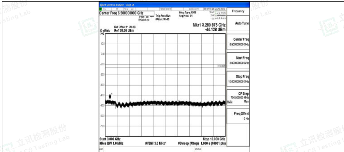
Band5_3MHz_16QAM_20635_1RB#0_3000~10000_3000~10000
