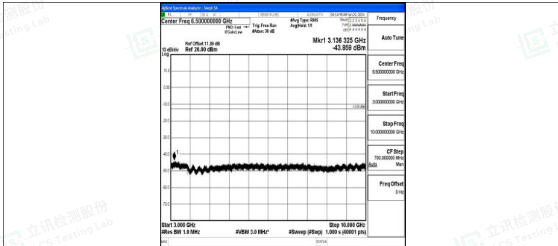
Band5_10MHz_QPSK_20525_1RB#0_3000~10000_3000~10000
