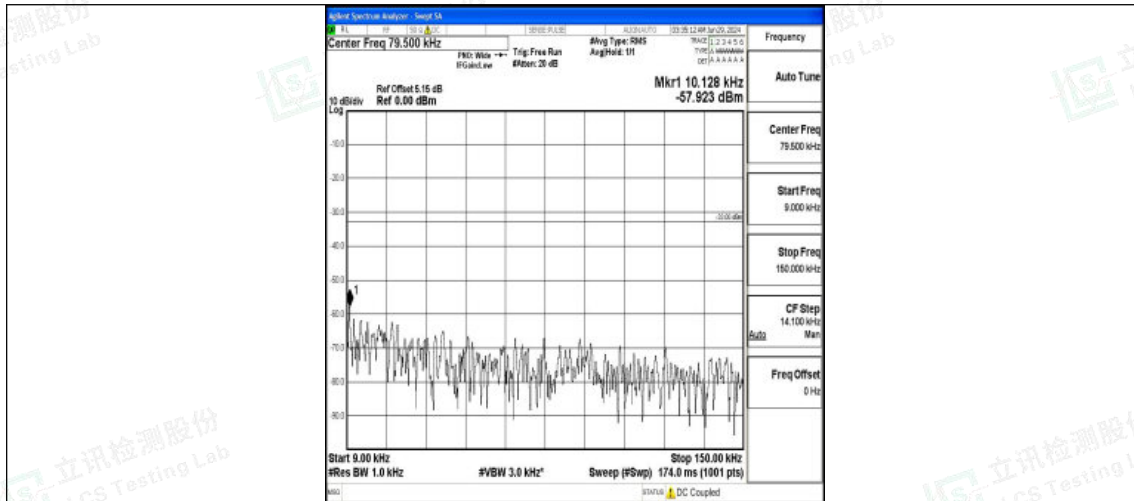
Band5_3MHz_16QAM_20415_1RB#0_0.009~0.15_0.009~0.15
