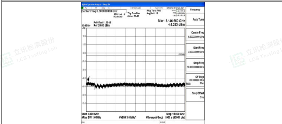
Band5_10MHz_QPSK_20450_1RB#0_3000~10000_3000~10000
