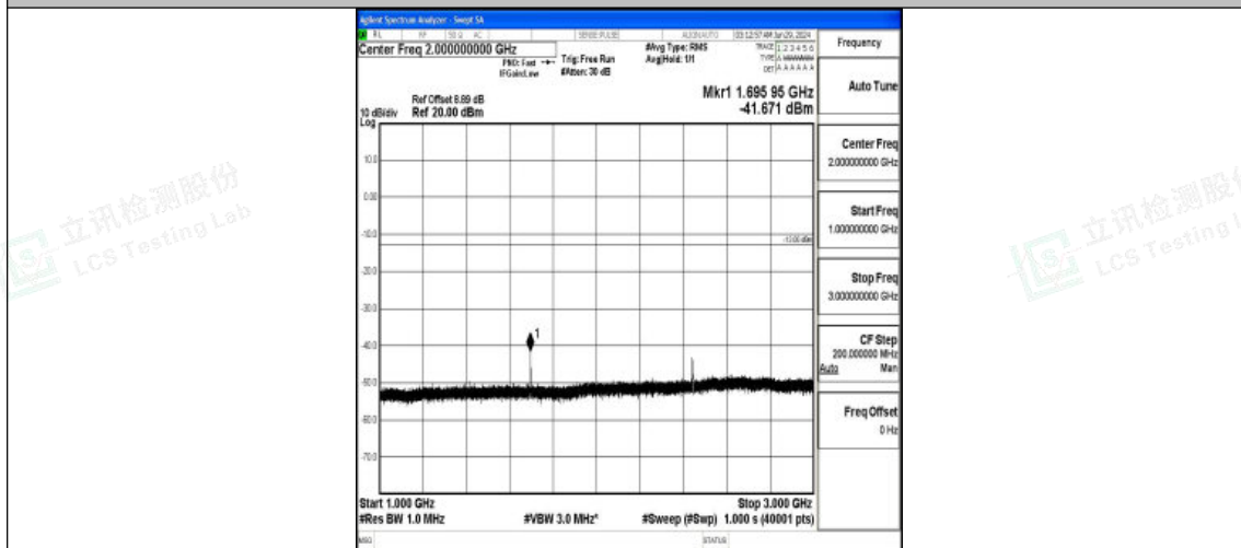
Band5_1.4MHz_16QAM_20643_1RB#0_1000~3000_1000~3000
