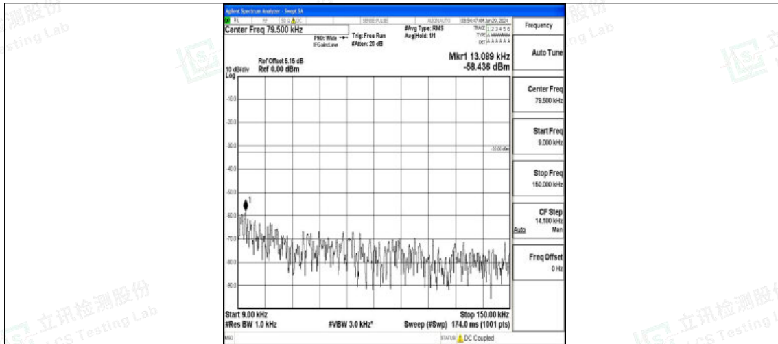
Band5_5MHz_16QAM_20425_1RB#0_0.009~0.15_0.009~0.15
