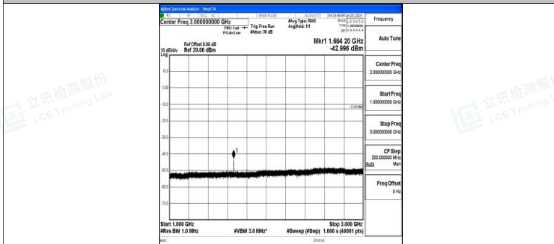
Band5_10MHz_QPSK_20525_1RB#0_1000~3000_1000~3000
