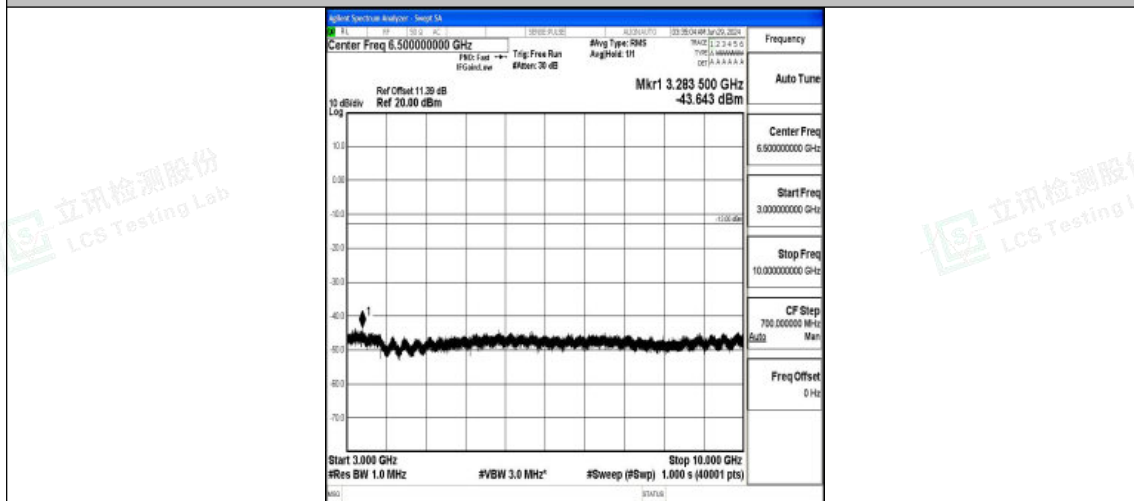
Band5_3MHz_QPSK_20415_1RB#0_3000~10000_3000~10000
