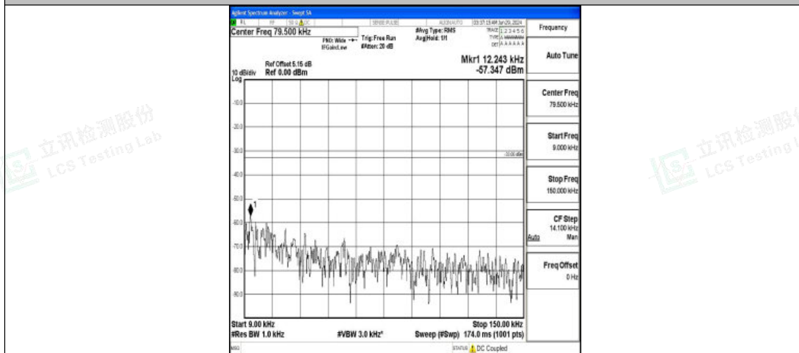
Band5_3MHz_16QAM_20635_1RB#0_0.009~0.15_0.009~0.15
