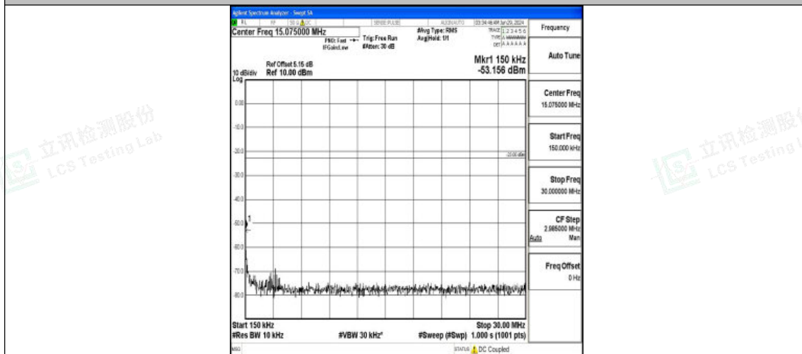
Band5_3MHz_QPSK_20415_1RB#0_0.15~30_0.15~30
