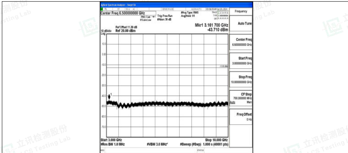
Band5_3MHz_QPSK_20525_1RB#0_3000~10000_3000~10000
