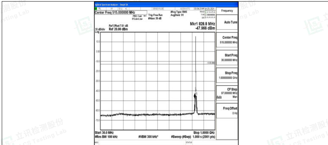
Band5_3MHz_16QAM_20525_1RB#0_30~1000_30~1000
