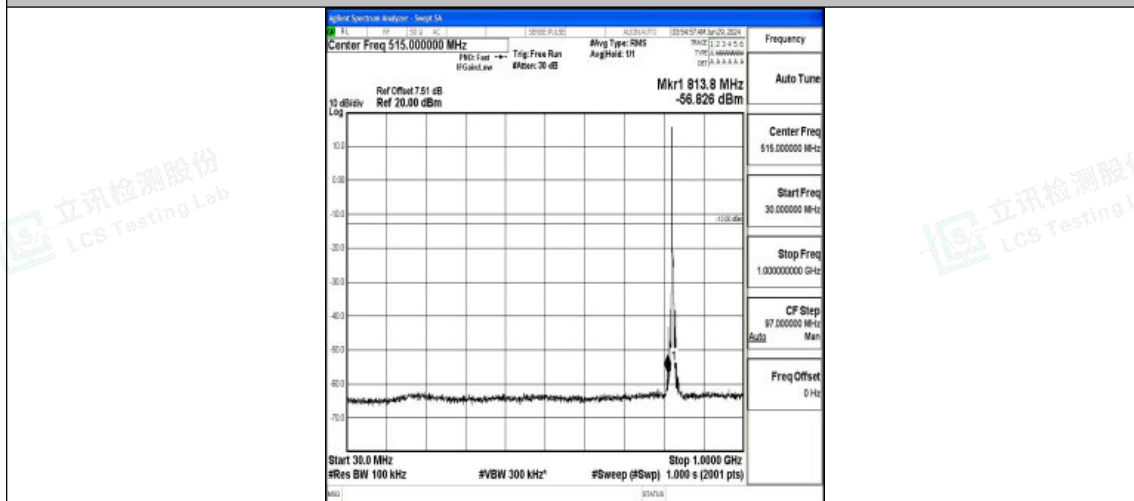
Band5_5MHz_16QAM_20425_1RB#0_30~1000_30~1000
