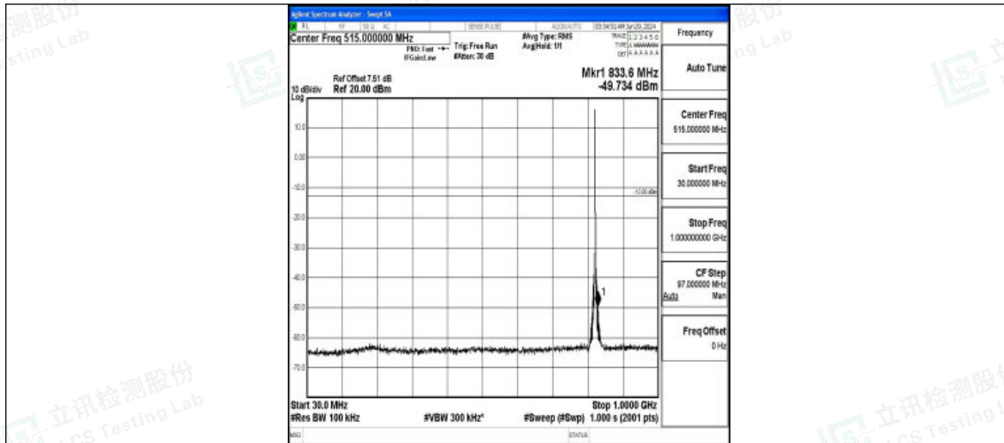
Band5_3MHz_QPSK_20415_1RB#0_30~1000_30~1000
