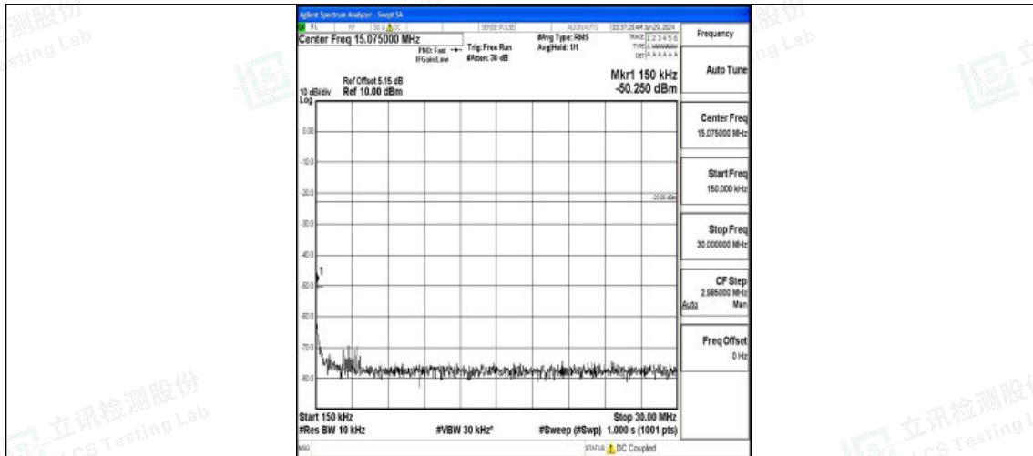
Band5_3MHz_16QAM_20635_1RB#0_0.15~30_0.15~30
