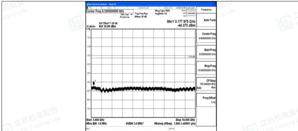
Band5_5MHz_QPSK_20525_1RB#0_3000~10000_3000~10000
