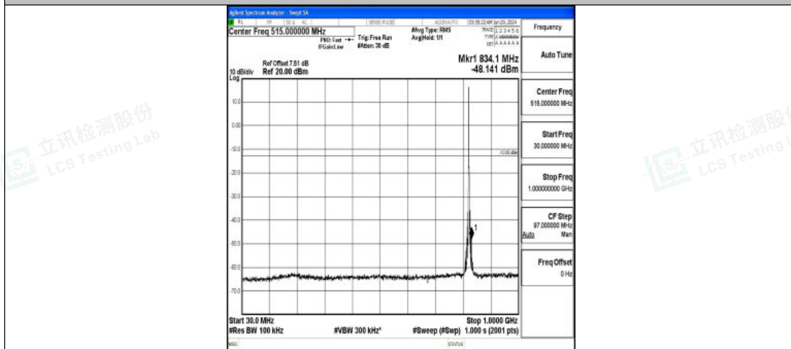
Band5_3MHz_16QAM_20415_1RB#0_30~1000_30~1000
