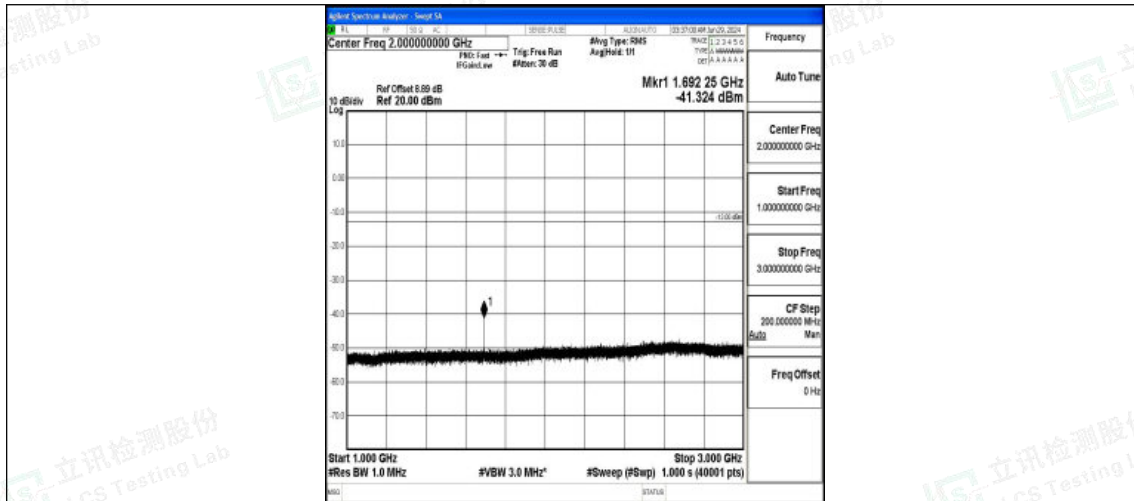
Band5_3MHz_QPSK_20635_1RB#0_1000~3000_1000~3000
