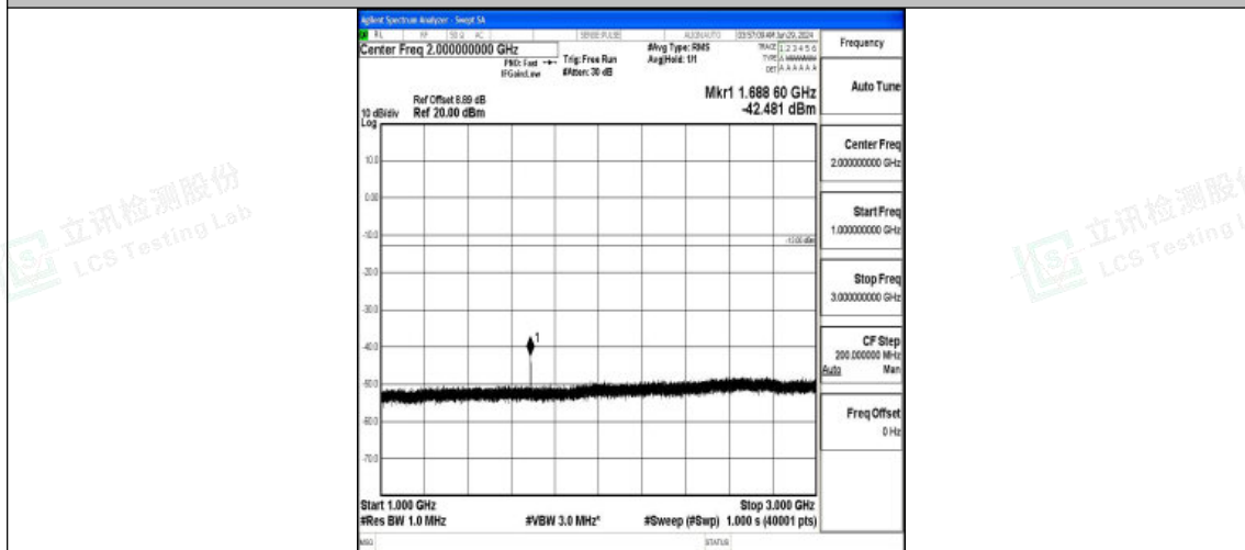
Band5_5MHz_16QAM_20625_1RB#0_1000~3000_1000~3000
