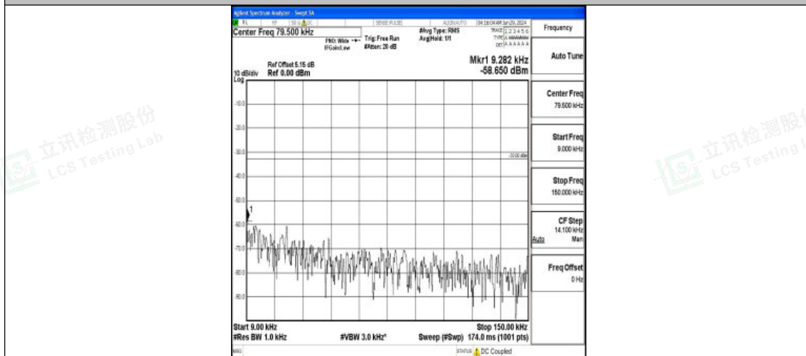
Band5_10MHz_16QAM_20600_1RB#0_0.009~0.15_0.009~0.15
