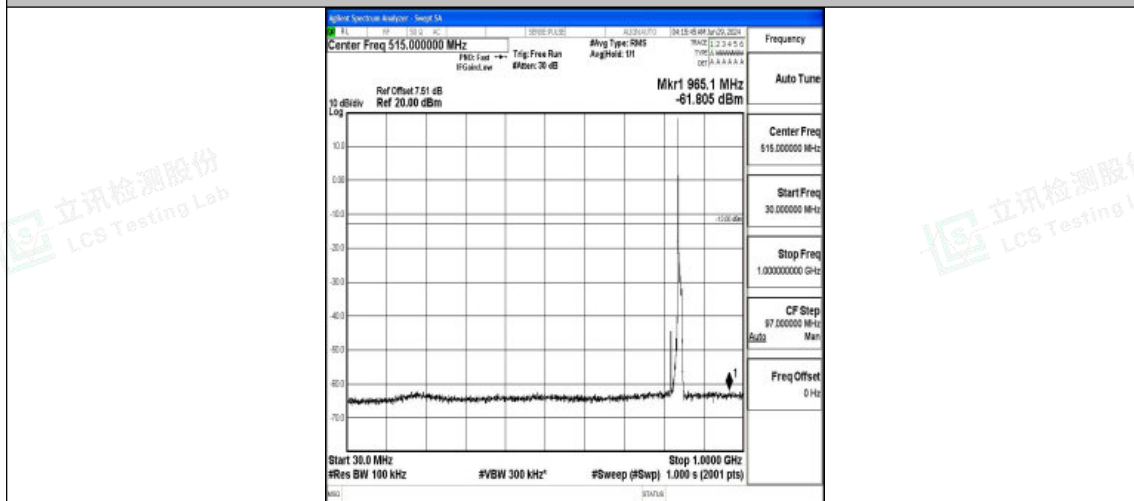
Band5_10MHz_QPSK_20600_1RB#0_30~1000_30~1000
