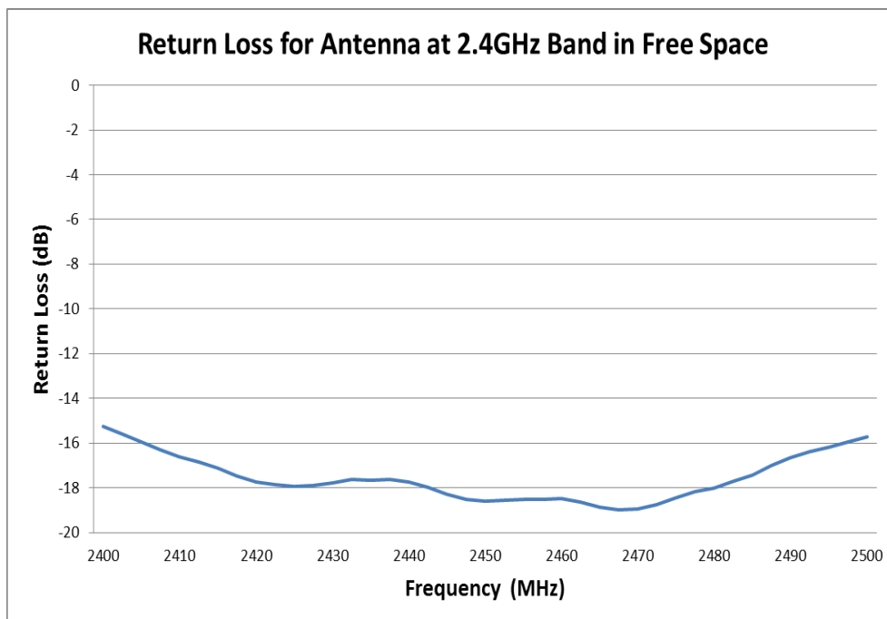
FIGURE 4.3.1 RETURN LOSS OF ANTENNA AT 2.4GHZ BAND IN FREE SPACE
