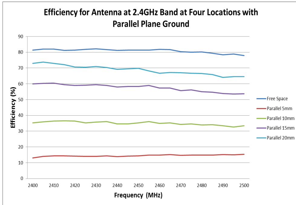
FIGURE 6.1.4 EFFICIENCY OF ANTENNA AT 2.4GHZ BAND AT FOUR LOCATIONS WITH PARALLEL PLANE GROUND
