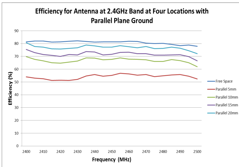
FIGURE 6.3.4 EFFICIENCY OF ANTENNA AT 2.4GHZ BAND AT FOUR LOCATIONS WITH PARALLEL PLANE GROUND
