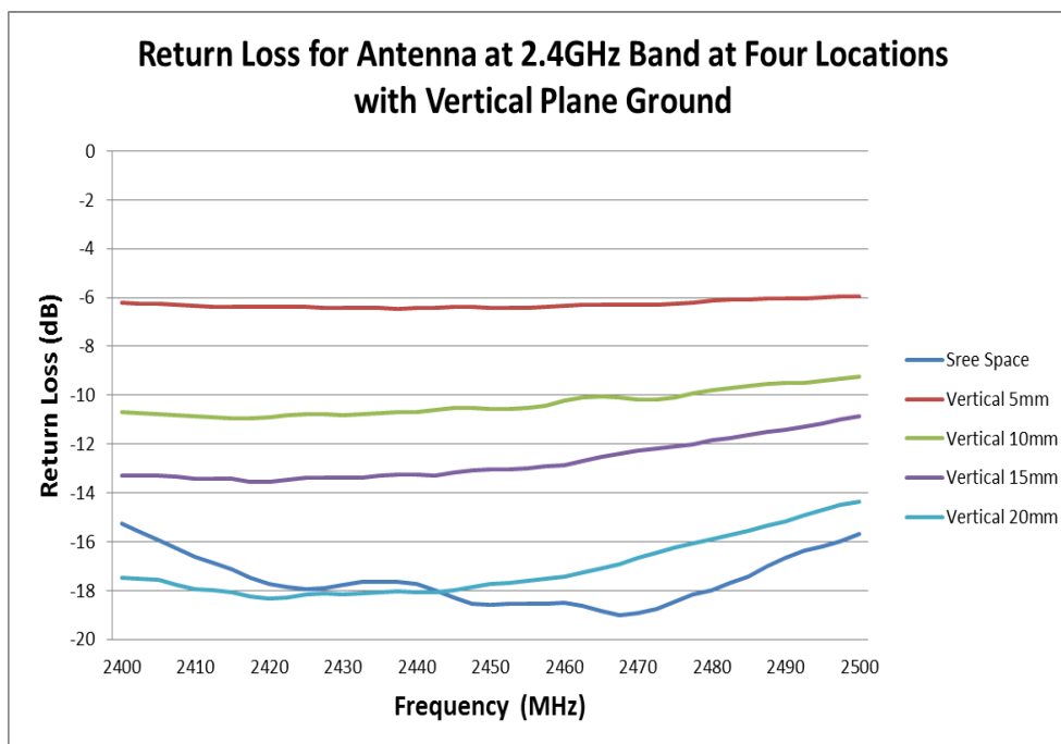
FIGURE 6.2.2 RETURN LOSS OF ANTENNA AT 2.4GHZ BAND AT FOUR LOCATIONS WITH VERTICAL PLANE GROUND
