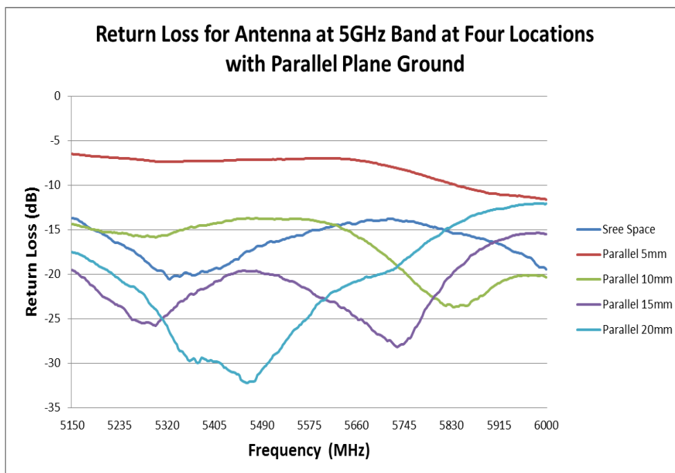
FIGURE 6.1.3 RETURN LOSS OF ANTENNA AT 5GHZ BAND AT FOUR LOCATIONS WITH PARALLEL PLANE GROUND
