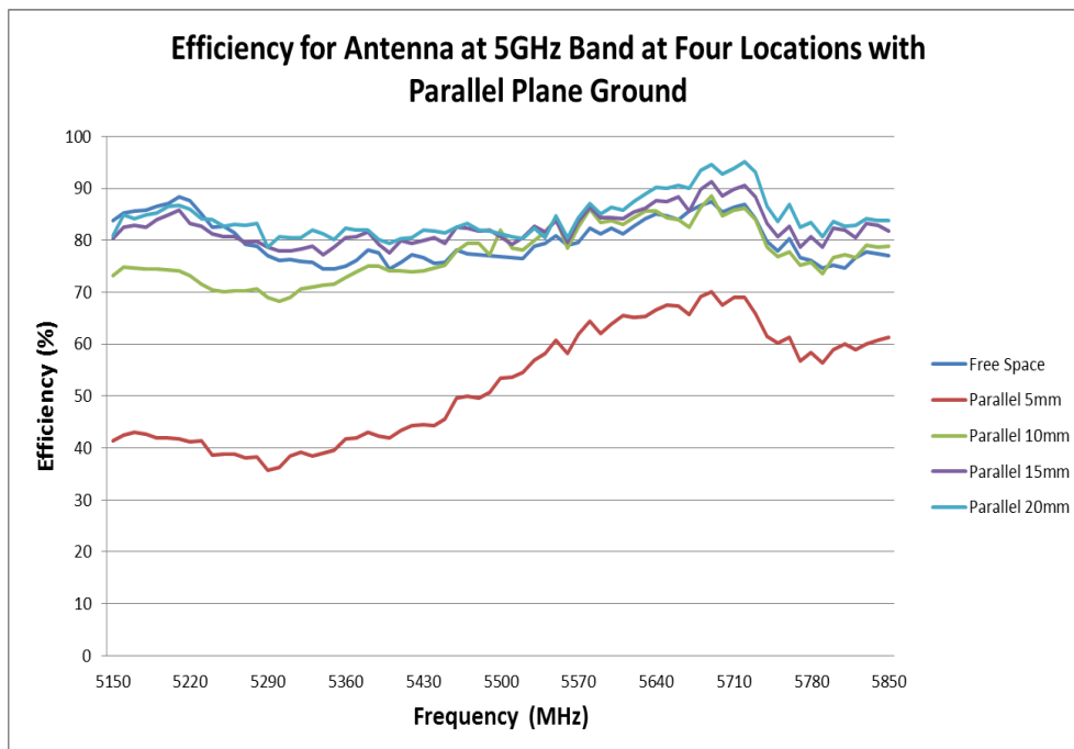
FIGURE 6.1.5 EFFICIENCY OF ANTENNA AT 5GHZ BAND AT FOUR LOCATIONS WITH PARALLEL PLANE GROUND
