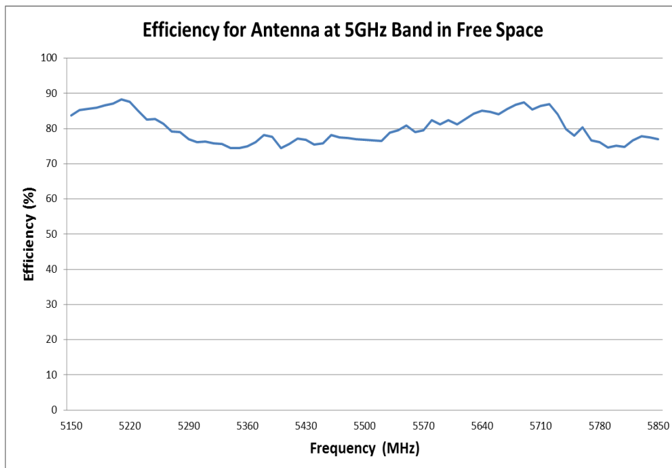
FIGURE 4.4.2 EFFICIENCY OF ANTENNA AT 5GHZ BAND IN FREE SPACE
