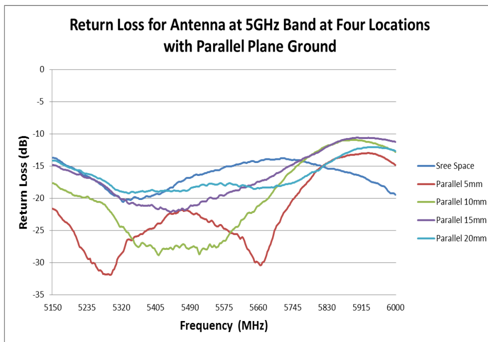
FIGURE 6.3.3 RETURN LOSS OF ANTENNA AT 5GHZ BAND AT FOUR LOCATIONS WITH PARALLEL PLANE GROUND
