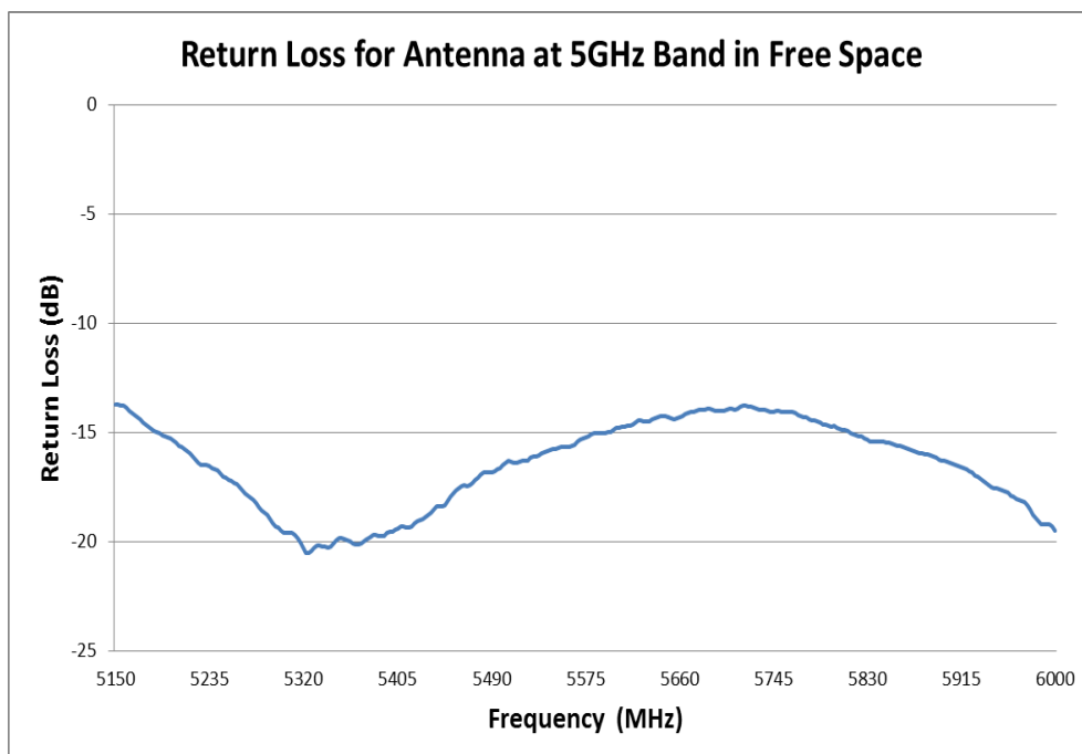
FIGURE 4.3.2 RETURN LOSS OF ANTENNA AT 5GHZ BAND IN FREE SPACE
