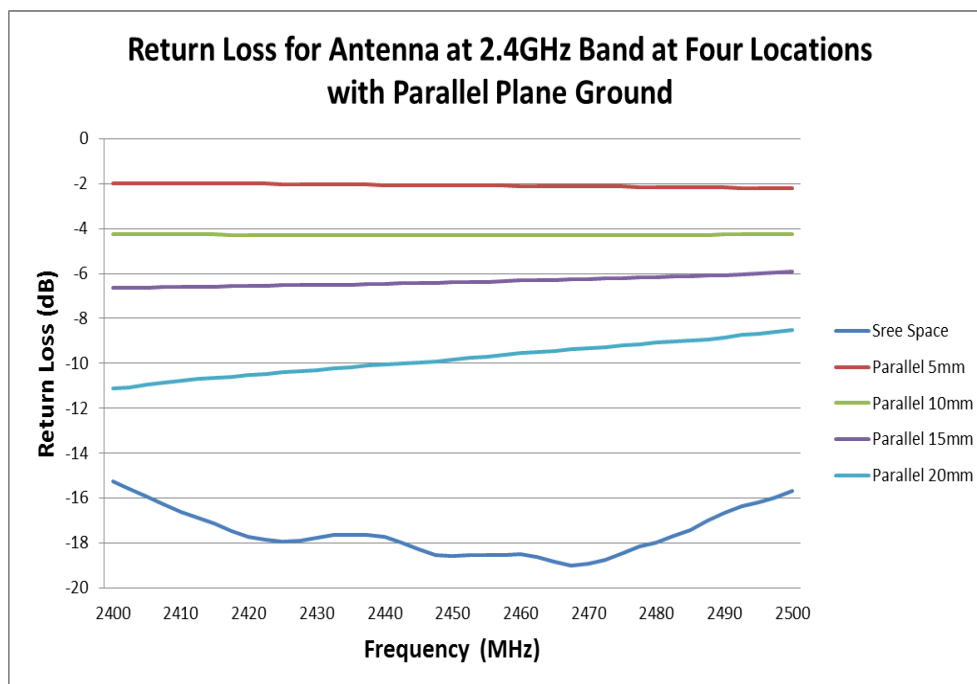
FIGURE 6.1.2 RETURN LOSS OF ANTENNA AT 2.4GHZ BAND AT FOUR LOCATIONS WITH PARALLEL PLANE GROUND
