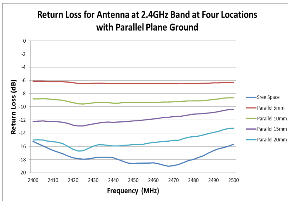
FIGURE 6.3.2 RETURN LOSS OF ANTENNA AT 2.4GHZ BAND AT FOUR LOCATIONS WITH PARALLEL PLANE GROUND
