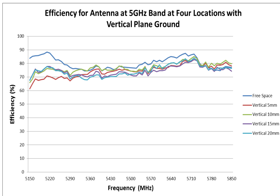
FIGURE 6.2.5 EFFICIENCY OF ANTENNA AT 5GHZ BAND AT FOUR LOCATIONS WITH VERTICAL PLANE GROUND
