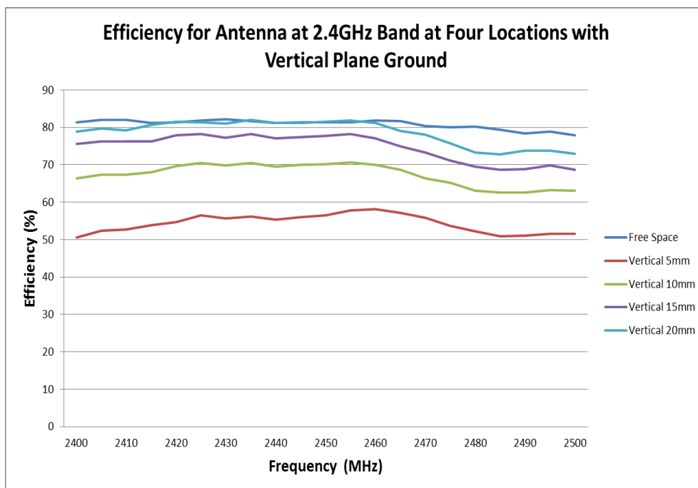
FIGURE 6.2.4 EFFICIENCY OF ANTENNA AT 2.4GHZ BAND AT FOUR LOCATIONS WITH VERTICAL PLANE GROUND
