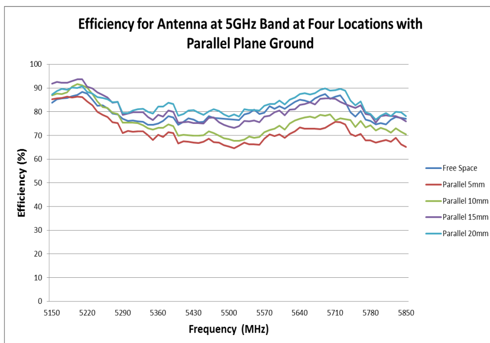
FIGURE 6.3.5 EFFICIENCY OF ANTENNA AT 5GHZ BAND AT FOUR LOCATIONS WITH PARALLEL PLANE GROUND
