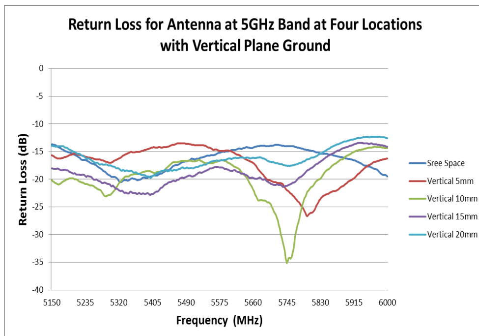
FIGURE 6.2.3 RETURN LOSS OF ANTENNA AT 5GHZ BAND AT FOUR LOCATIONS WITH VERTICAL PLANE GROUND
