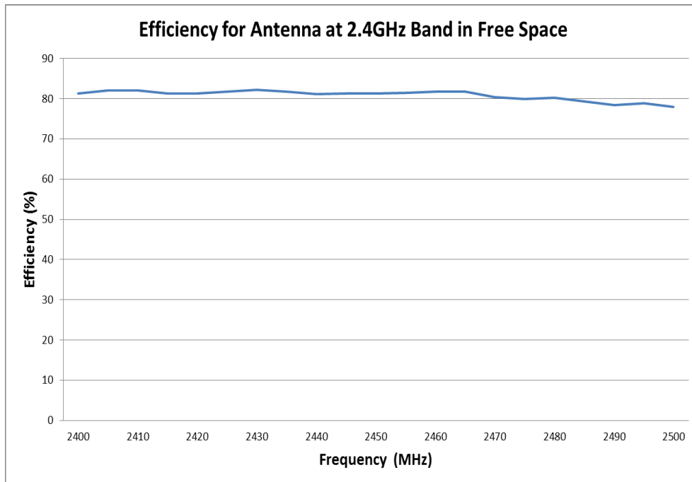
FIGURE 4.4.1 EFFICIENCY OF ANTENNA AT 2.4GHZ BAND IN FREE SPACE
