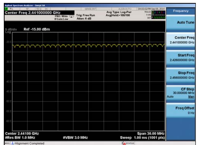
2-DH5_3
