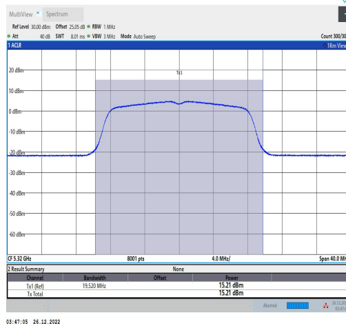
11A-Ant2-5320-TPC L-----15.03-95.89-0.18
