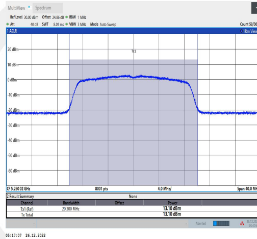
11N20MIMO-Ant1-5260-TPC L-----12.94-96.32-0.16
