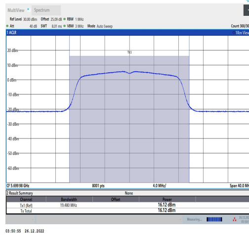
11A-Ant2-5700-TPC L-----15.94-95.89-0.18
