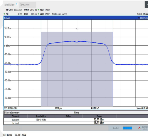
11A-Ant2-5260-TPC L-----15.59-96.55-0.15
