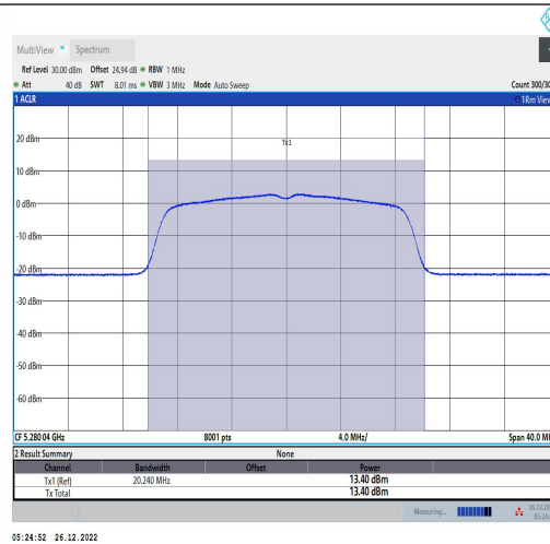
11N20MIMO-Ant1-5280-TPC L-----13.21-95.62-0.19
