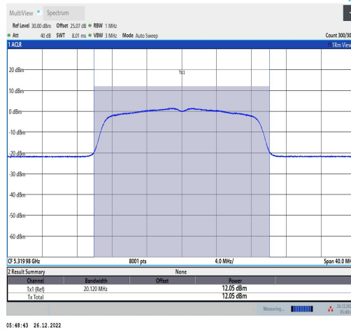
11N20MIMO-Ant2-5320-TPC L-----11.85-95.59-0.20
