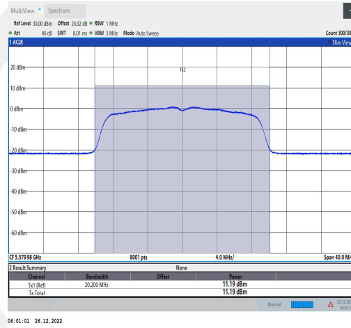
11N20MIMO-Ant2-5580-TPC L-----11.00-95.62-0.19
