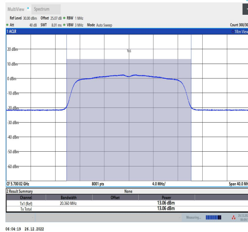
11N20MIMO-Ant1-5700-TPC L-----12.90-96.32-0.16
