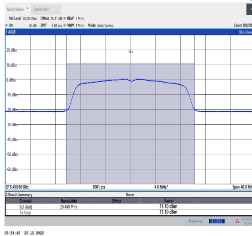
11N20MIMO-Ant2-5500-TPC L-----10.90-95.59-0.20
