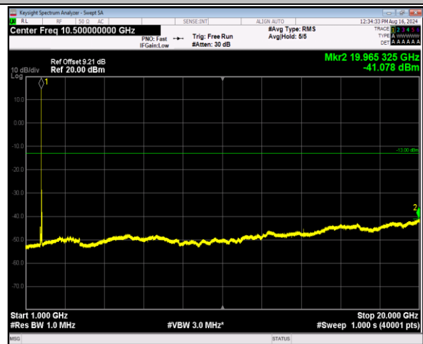
66-66-5MHz-20MHz-64QAM-64QAM-132455-132572-1RB# 0-1RB#99-1000~20000MHz-PASS
