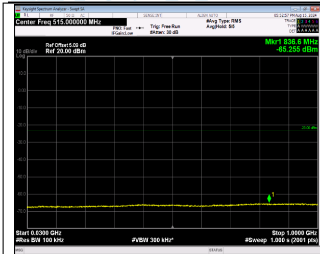
66-66-20MHz-5MHz-16QAM-16QAM-132522-132639-1R B#0-0RB#0-30~1000MHz-PASS
