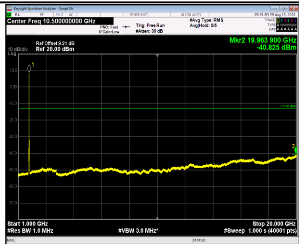
66-66-20MHz-5MHz-16QAM-16QAM-132397-132514-100R B#0-25RB#0-1000~20000MHz-PASS
