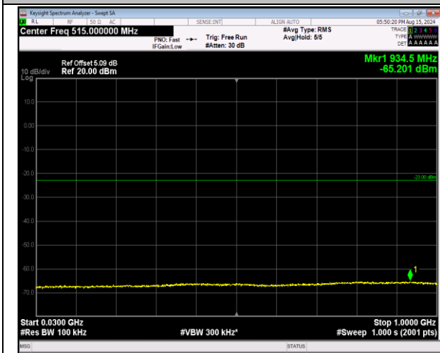
66-66-20MHz-5MHz-16QAM-16QAM-132397-132514-1R B#0-1RB#24-30~1000MHz-PASS
