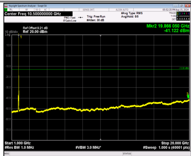
66-66-20MHz-5MHz-QPSK-QPSK-132522-132639-1RB#0- ORB#0-1000~20000MHz-PASS
