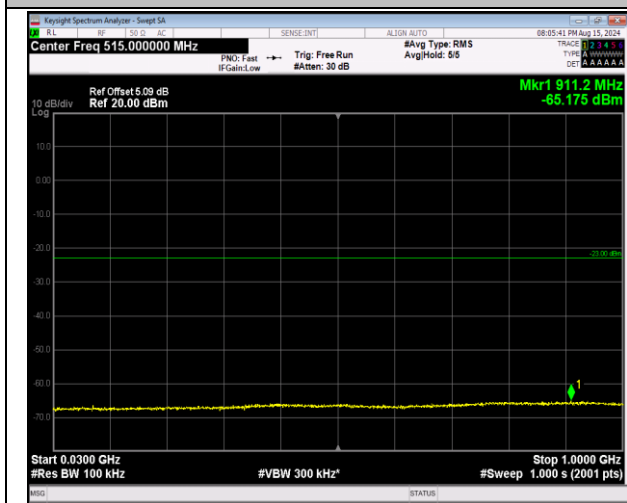
66-66-20MHz-5MHz-64QAM-64QAM-132397-132514-10 ORB#0-25RB#0-30~1000MHz-PASS
