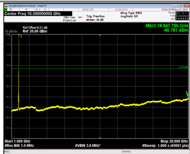
66-66-20MHz-5MHz-16QAM-16QAM-132522-132639-1RB# 99-0RB#0-1000~20000MHz-PASS
