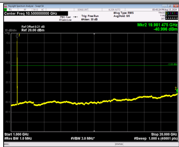
66-66-20MHz-5MHz-16QAM-16QAM-132072-132189-1RB# 0-1RB#24-1000~20000MHz-PASS
