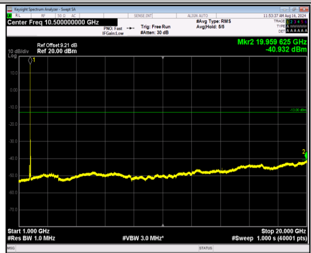
66-66-5MHz-20MHz-16QAM-16QAM-132455-132572-1RB# 0-1RB#99-1000~20000MHz-PASS
