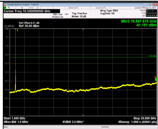
66-66-5MHz-20MHz-64QAM-64QAM-132455-132572-1RB# 24-ORB#0-1000~20000MHz-PASS
