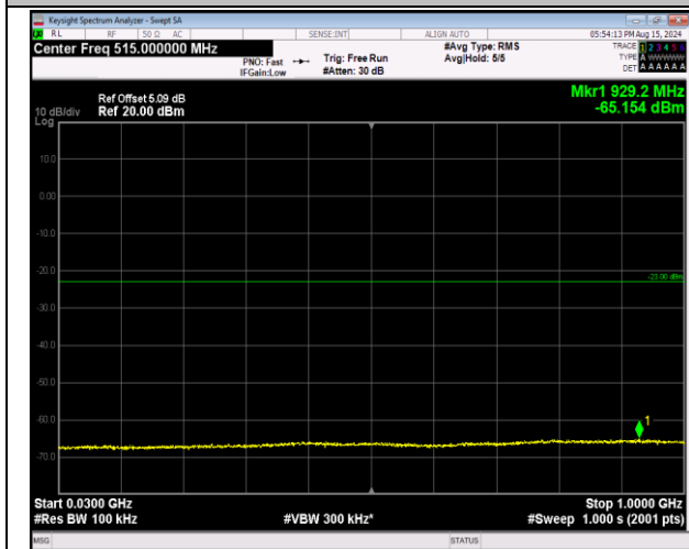
66-66-20MHz-5MHz-16QAM-16QAM-132522-132639-1R B#99-0RB#0-30~1000MHz-PASS
