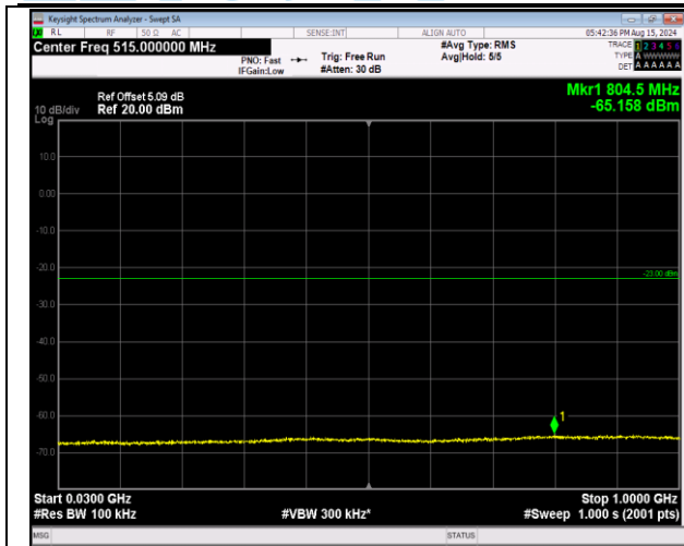
66-66-20MHz-5MHz-16QAM-16QAM-132072-132189-1R B#0-ORB#0-30~1000MHz-PASS
