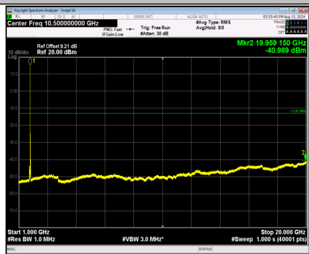
66-66-20MHz-5MHz-16QAM-16QAM-132522-132639-1RB# 0-1RB#24-1000~20000MHz-PASS
