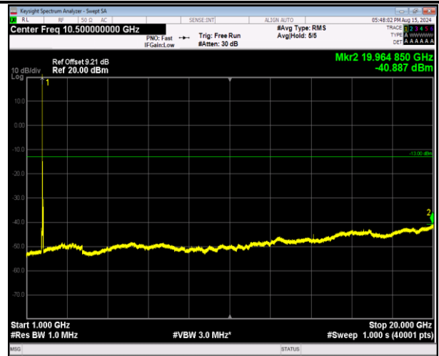
66-66-20MHz-5MHz-16QAM-16QAM-132397-132514-1RB# 0-0RB#0-1000~20000MHz-PASS
