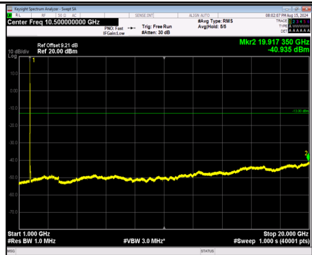
66-66-20MHz-5MHz-64QAM-64QAM-132072-132189-1RB# 99-ORB#0-1000~20000MHz-PASS
