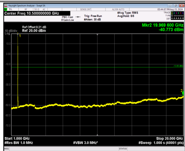
66-66-20MHz-5MHz-16QAM-16QAM-132072-132189-1RB# 99-0RB#0-1000~20000MHz-PASS
