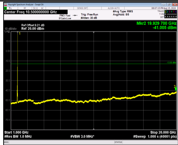
66-66-20MHz-5MHz-64QAM-64QAM-132522-132639-1RB# 99-ORB#0-1000~20000MHz-PASS
