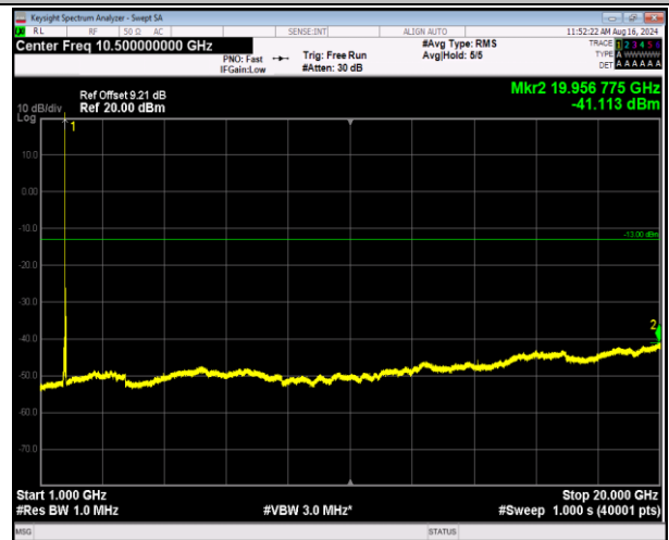
66-66-5MHz-20MHz-16QAM-16QAM-132455-132572-1RB# 24-0RB#0-1000~20000MHz-PASS
