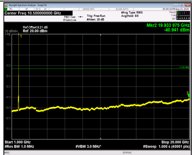
66-66-20MHz-5MHz-16QAM-16QAM-132397-132514-1RB# 99-0RB#0-1000~20000MHz-PASS
