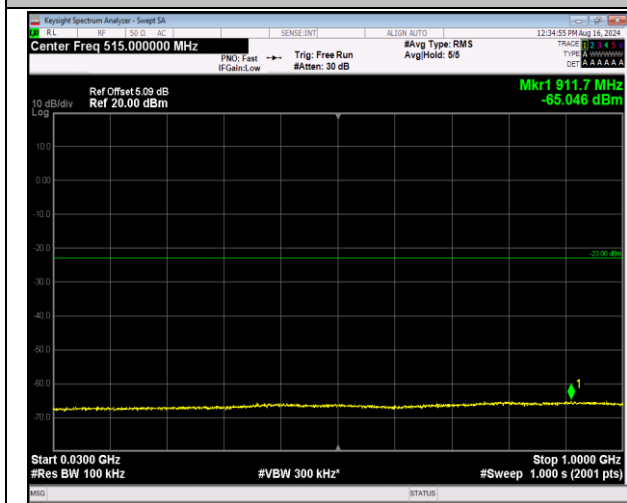
66-66-5MHz-20MHz-64QAM-64QAM-132455-132572-25 RB#0-100RB#0-30~1000MHz-PASS
