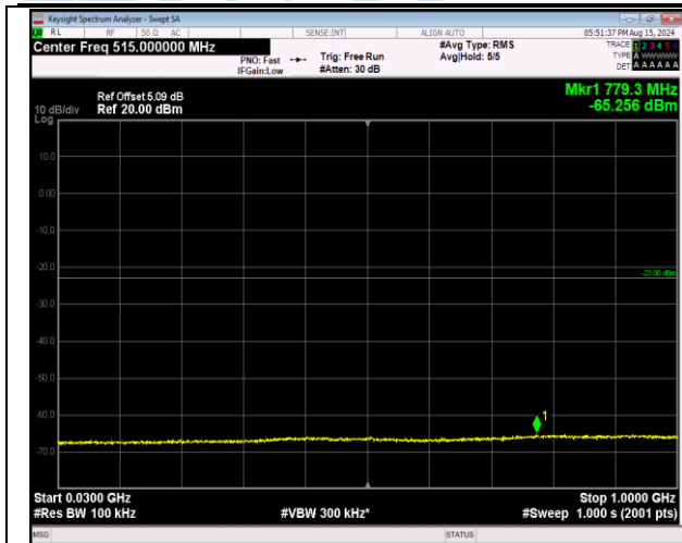
66-66-20MHz-5MHz-16QAM-16QAM-132397-132514-10 ORB#0-25RB#0-30~1000MHz-PASS
