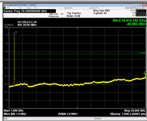
66-66-20MHz-5MHz-64QAM-64QAM-132397-132514-100R B#0-25RB#0-1000~20000MHz-PASS
