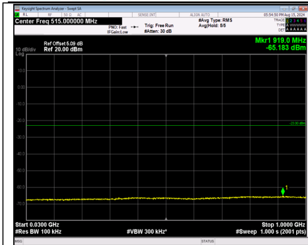
66-66-20MHz-5MHz-QPSK-QPSK-132522-132639-1RB# 0-1RB#24-30~1000MHz-PASS
