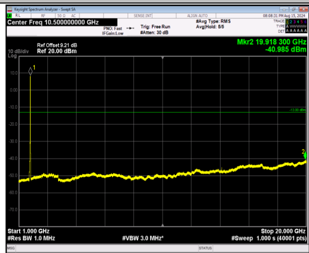
66-66-20MHz-5MHz-64QAM-64QAM-132522-132639-100R B#0-25RB#0-1000~20000MHz-PASS
