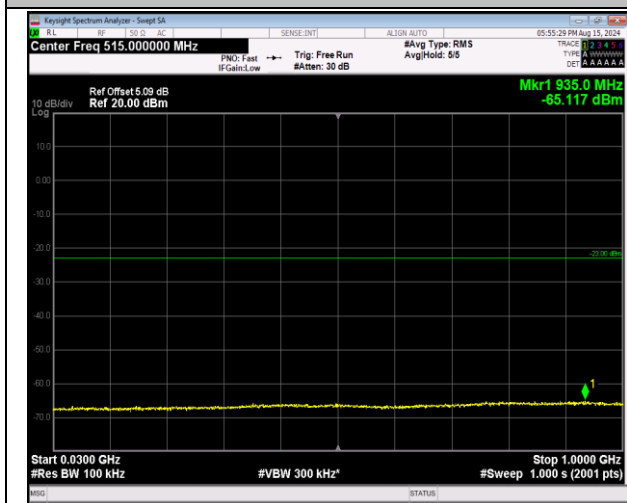
66-66-20MHz-5MHz-16QAM-16QAM-132522-132639-1R B#0-1RB#24-30~1000MHz-PASS
