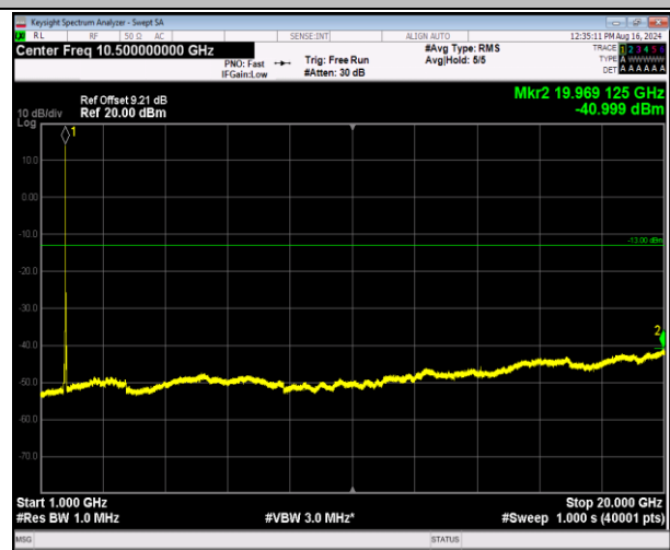
66-66-5MHz-20MHz-64QAM-64QAM-132455-132572-25RB #0-100RB#0-1000~20000MHz-PASS
