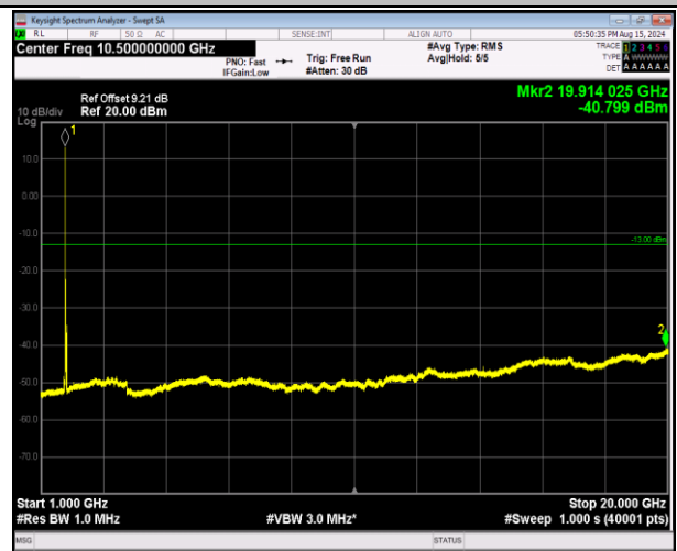
66-66-20MHz-5MHz-16QAM-16QAM-132397-132514-1RB# 0-1RB#24-1000~20000MHz-PASS
