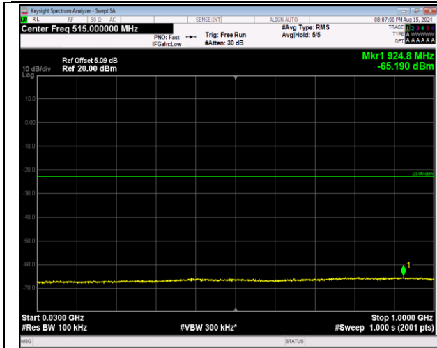
66-66-20MHz-5MHz-64QAM-64QAM-132522-132639-1R B#99-ORB#0-30~1000MHz-PASS
