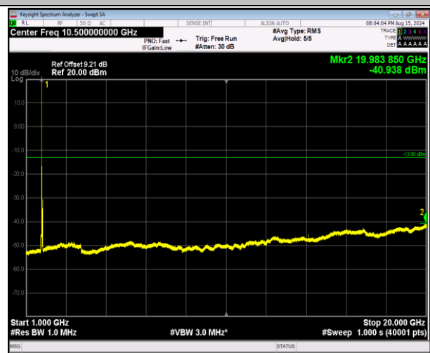
66-66-20MHz-5MHz-64QAM-64QAM-132397-132514-1RB# 0-ORB#0-1000~20000MHz-PASS
