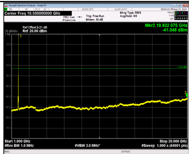
66-66-20MHz-5MHz-64QAM-64QAM-132397-132514-1RB# 99-ORB#0-1000~20000MHz-PASS
