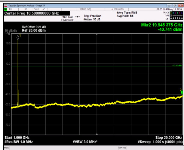
66-66-20MHz-5MHz-64QAM-64QAM-132397-132514-1RB# 0-1RB#24-1000~20000MHz-PASS
