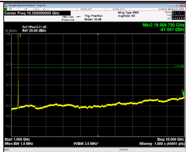
66-66-5MHz-20MHz-16QAM-16QAM-132455-132572-25RB #0-100RB#0-1000~20000MHz-PASS
