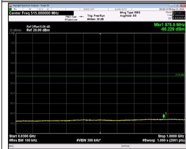
66-66-20MHz-5MHz-64QAM-64QAM-132522-132639-10 ORB#0-25RB#0-30~1000MHz-PASS
