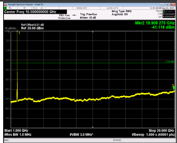
66-66-5MHz-20MHz-16QAM-16QAM-132455-132572-1RB# 0-0RB#0-1000~20000MHz-PASS
