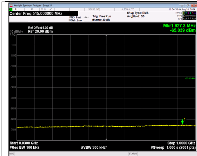
66-66-5MHz-20MHz-16QAM-16QAM-132455-132572-25 RB#0-100RB#0-30~1000MHz-PASS
