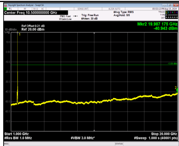
66-66-20MHz-5MHz-16QAM-16QAM-132522-132639-1RB# 0-0RB#0-1000~20000MHz-PASS
