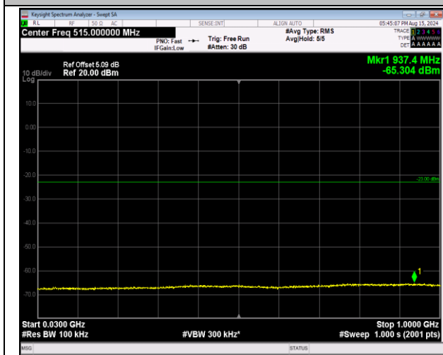
66-66-20MHz-5MHz-16QAM-16QAM-132072-132189-1R B#0-1RB#24-30~1000MHz-PASS
