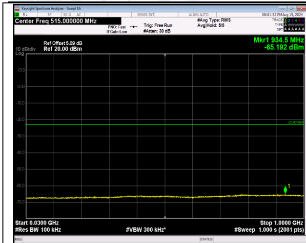
66-66-20MHz-5MHz-64QAM-64QAM-132072-132189-1R B#99-ORB#0-30~1000MHz-PASS
