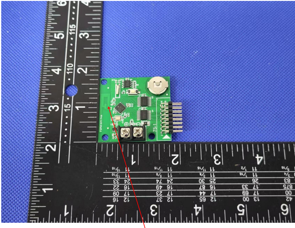
PCB antenna
