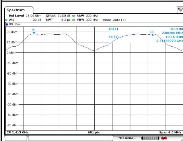
Channel Separation Plot on Channel 01 - 02
