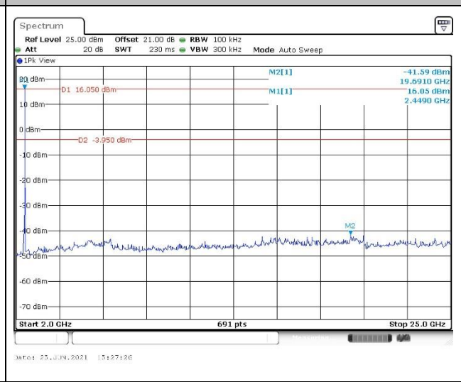
CSE Plot on CH 27 between 2 GHz ~ 25 GHz
