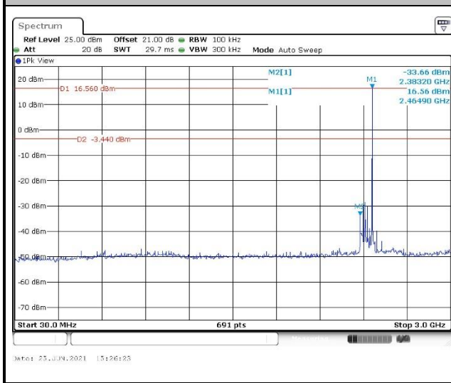
CSE Plot on CH 27 between 30 MHz ~ 3 GHz
