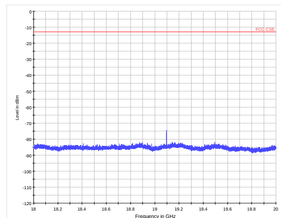
GSM 1900 CH-High 18GHz~20GHz
