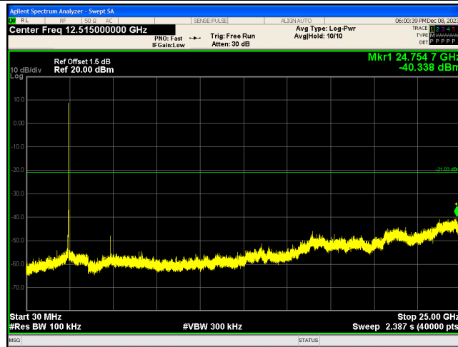
802.11b_2462_0~Reference
