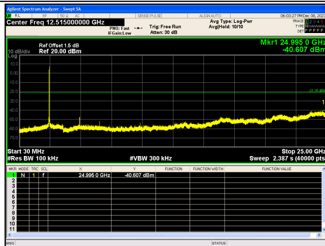
802.11g_2412_0~Reference
