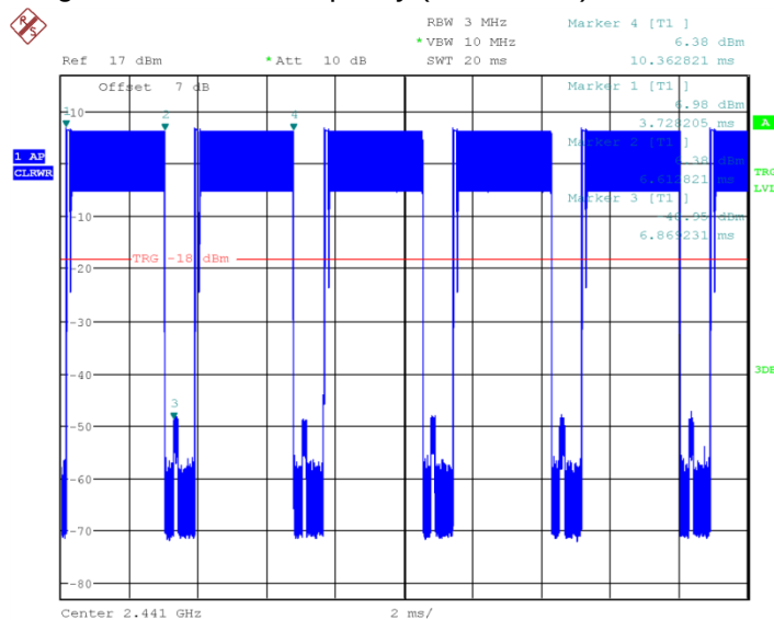
Fig 94. Time of occupancy (Dwell Time): Ch39,Packet 3-DH5
