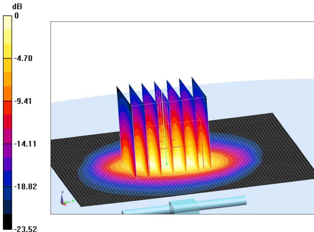
Fig.J.4 validation 2600 MHz 250mW
