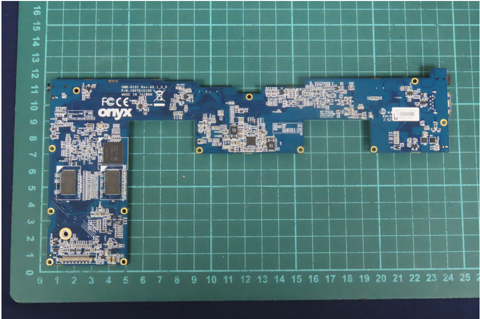
(23) EUT Photo
