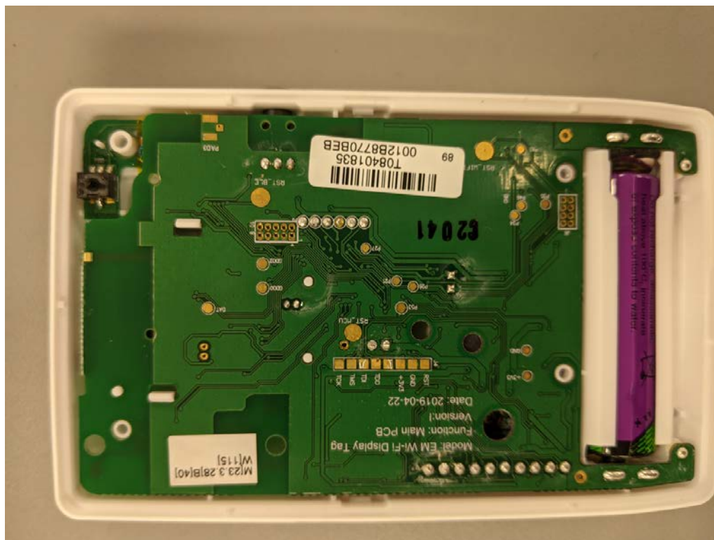
5 Inside Back View
