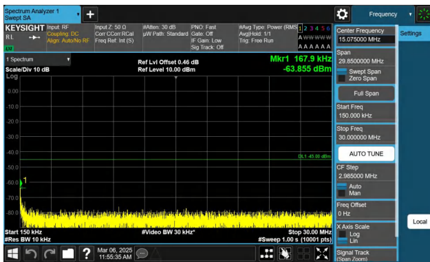
Band7-20MHz-QPSK-21100-1RB#99-0.15~30-PASS
