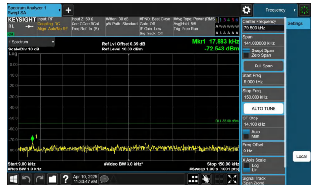
Band7-15MHz-QPSK-21100-1RB#74-0.009~0.15-PASS
