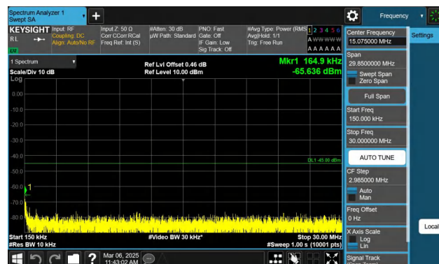
Band7-15MHz-QPSK-21375-1RB#0-0.15~30-PASS
