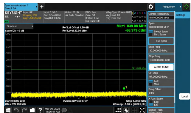
Band7-10MHz-QPSK-21400-1RB#49-30~1000-PASS
