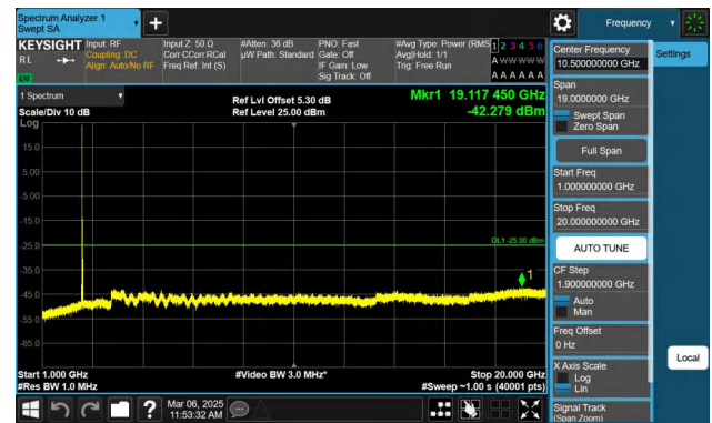
Band7-20MHz-QPSK-20850-1RB#0-1000~20000-PASS
