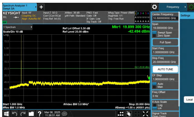
Band7-10MHz-QPSK-21400-1RB#49-1000~20000-PASS
