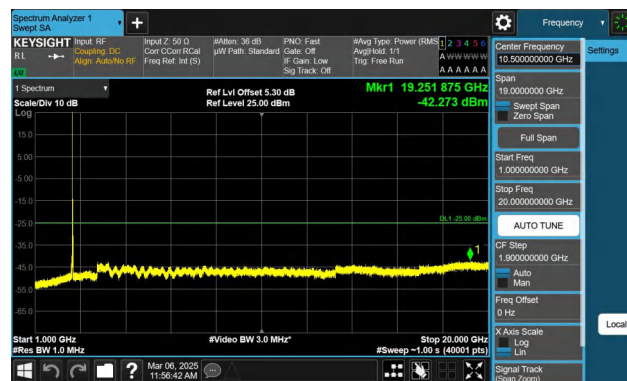
Band7-20MHz-QPSK-21350-1RB#0-1000~20000-PASS
