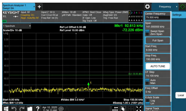
Band7-15MHz-QPSK-21375-1RB#0-0.009~0.15-PASS
