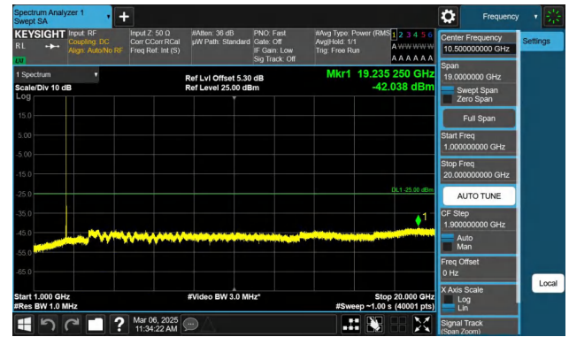
Band7-10MHz-QPSK-21100-1RB#0-1000~20000-PASS
