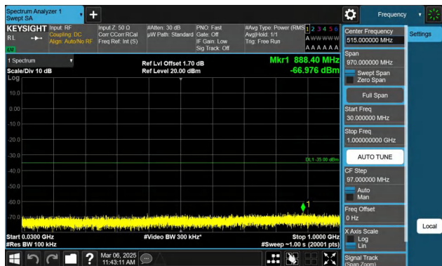
Band7-15MHz-QPSK-21375-1RB#0-30~1000-PASS
