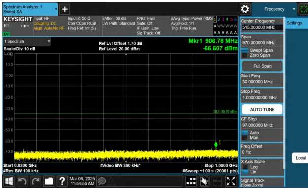
Band7-20MHz-QPSK-21100-1RB#0-30~1000-PASS
