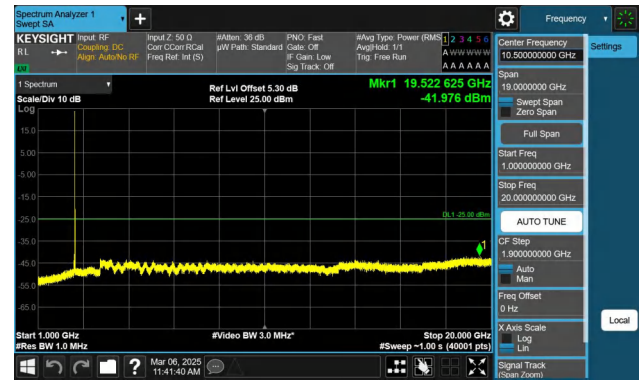
Band7-15MHz-QPSK-21100-1RB#0-1000~20000-PASS
