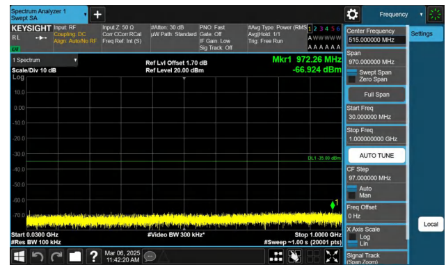
Band7-15MHz-QPSK-21100-1RB#74-30~1000-PASS
