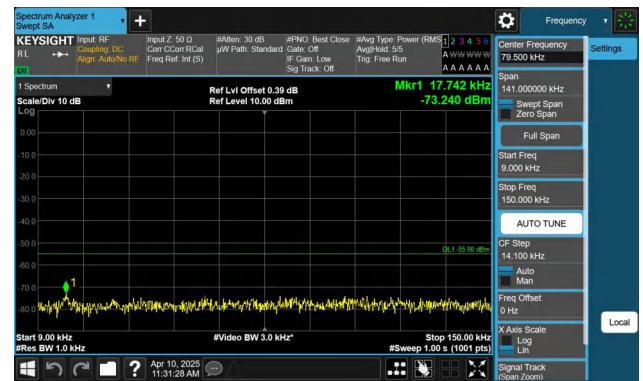
Band7-10MHz-QPSK-21100-1RB#49-0.009~0.15-PASS
