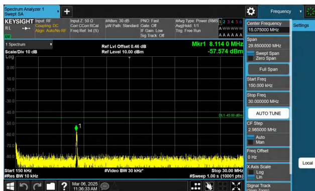
Band7-10MHz-QPSK-21400-1RB#49-0.15~30-PASS
