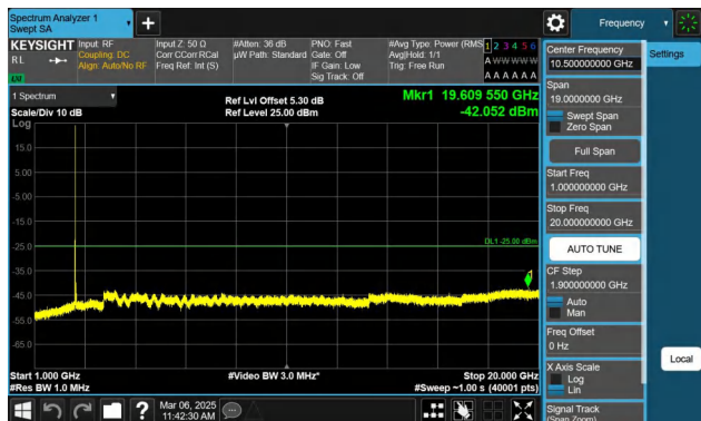
Band7-15MHz-QPSK-21100-1RB#74-1000~20000-PASS
