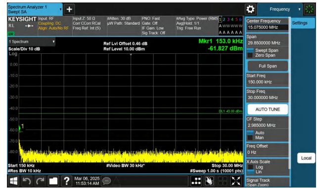
Band7-20MHz-QPSK-20850-1RB#0-0.15~30-PASS
