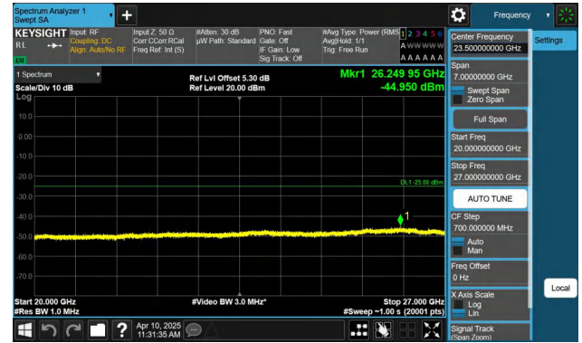
Band7-10MHz-QPSK-21100-1RB#49-20000~27000-PASS
