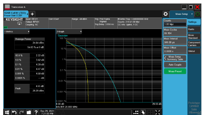
5G NR n77_CH656000_20M_1RB_16-QAM_Ratio
