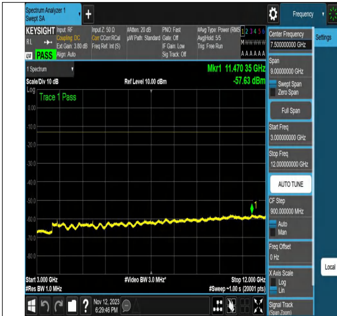
NTNV-N2-PC3-15-20-H-CP-256QAM-Out_ Full-Ant1-PASS
