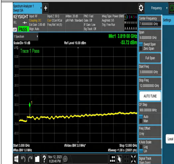
NTNV-N2-PC3-15-20-H-CP-64QAM-Edge_1RB_Right-Ant1-PA
