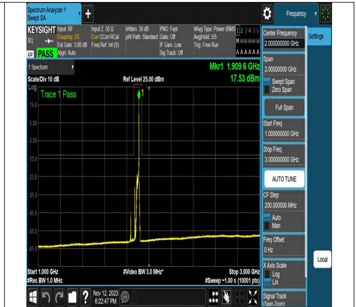
NTNV-N2-PC3-15-20-H-CP-QPSK-Edge_1RB_Right-Ant1-PAS
