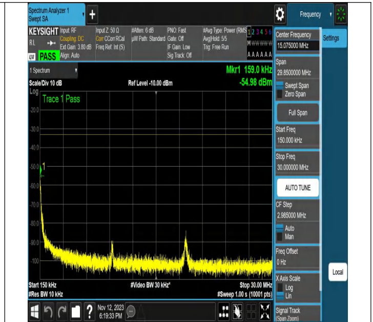
NTNV-N2-PC3-15-20-H-DFT-256QAM-Edge_1RB_Right-Ant1-P
