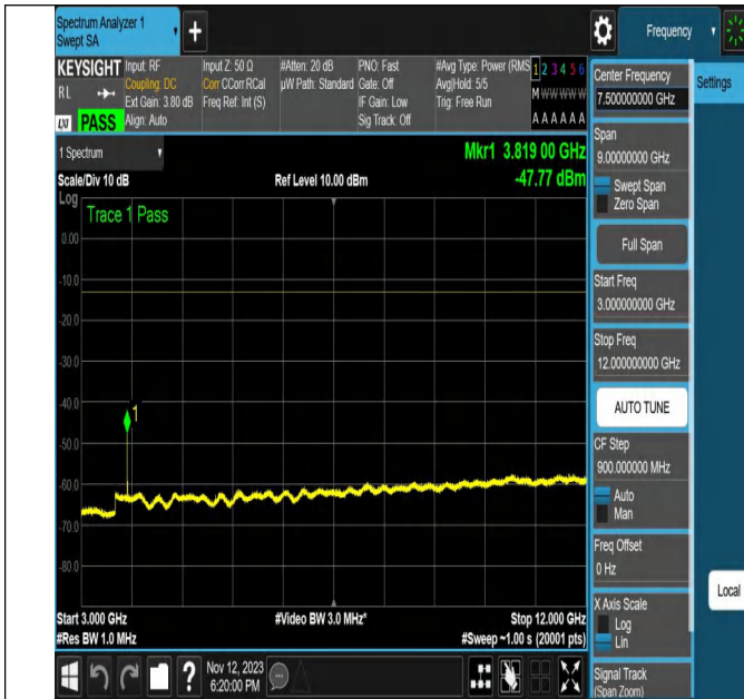
NTVN-N2-PC3-15-20-H-DFT-256QAM-Edge_1RB_Right-Ant1-P
