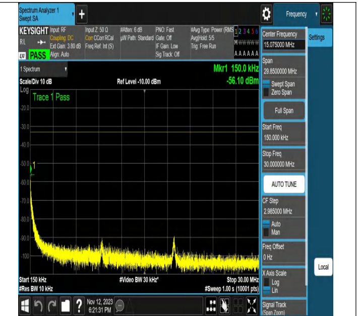
NTNV-N2-PC3-15-20-H-CP-QPSK-Edge_1RB_Left-Ant1-PASS
