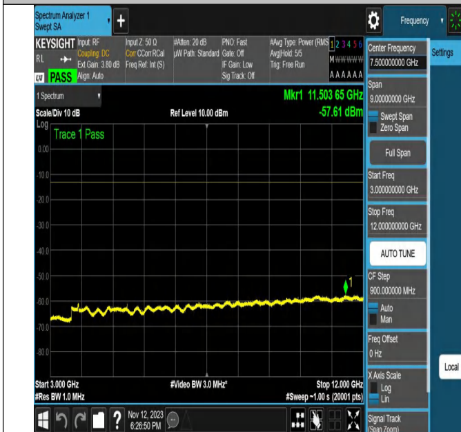
NTNV-N2-PC3-15-20-H-CP-64QAM-Outer_Full-Ant1-PASS
