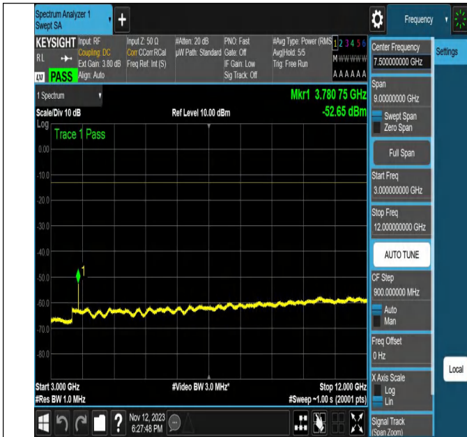
NTNV-N2-PC3-15-20-H-CP-64QAM-Edge_1RB_Left-Ant1-PAS
