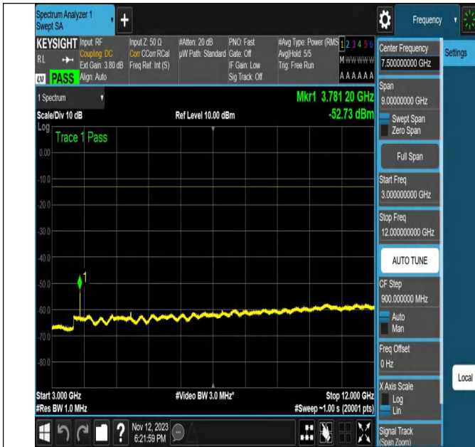
NTNV-N2-PC3-15-20-H-CP-QPSK-Edge_1RB_Left-Ant1-PASS
