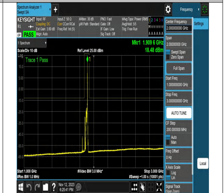
NTNV-N2-PC3-15-20-H-CP-16QAM-Edge_1RB_Right-Ant1-PA
