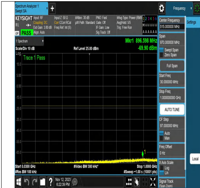
NTNV-N2-PC3-15-20-H-CP-QPSK-Edge_1RB_Right-Ant1-PAS
