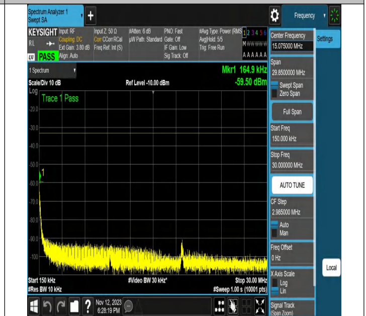
NTNV-N2-PC3-15-20-H-CP-64QAM-Edge_1RB_Right-Ant1-PA
