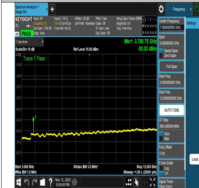
NTNV-N2-PC3-15-20-H-CP-256QAM-Edge_1RB_Left-Ant1-PAS
