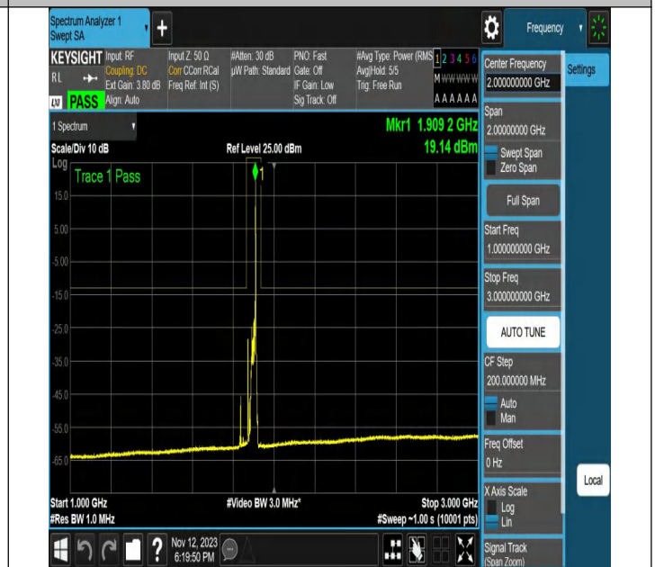
NTNV-N2-PC3-15-20-H-DFT-256QAM-Edge_1RB_Right-Ant1-P
