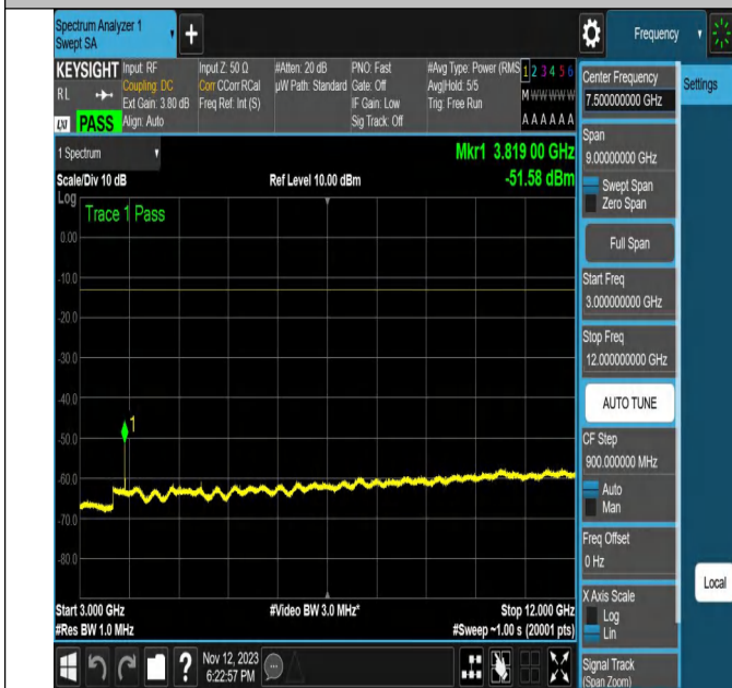
NTNV-N2-PC3-15-20-H-CP-QPSK-Edge_1RB_Right-Ant1-PAS
