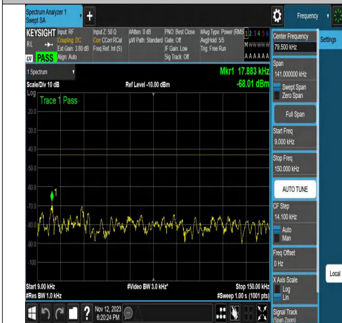
NTVN-N2-PC3-15-20-H-CP-QPSK-Outer_Full-Ant1-PASS
