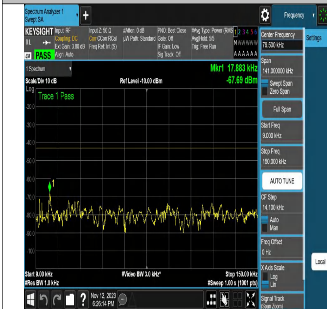
NTNV-N2-PC3-15-20-H-CP-64QAM-Outer_Full-Ant1-PASS
