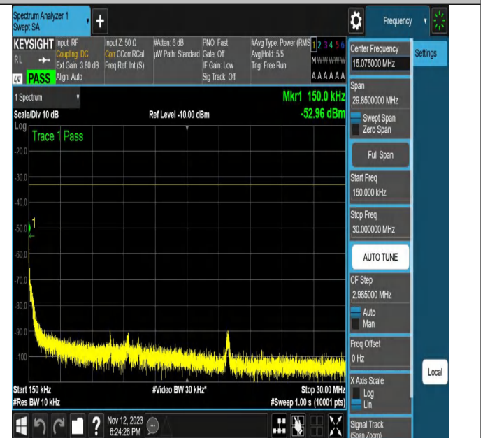
NTNV-N2-PC3-15-20-H-CP-16QAM-Edge_1RB_Left-Ant1-PAS
