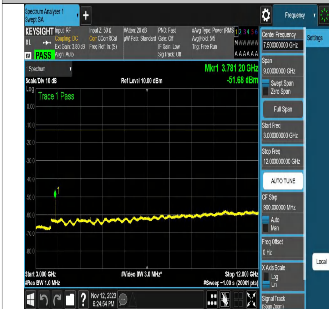
NTNV-N2-PC3-15-20-H-CP-16QAM-Edge_1RB_Left-Ant1-PAS
