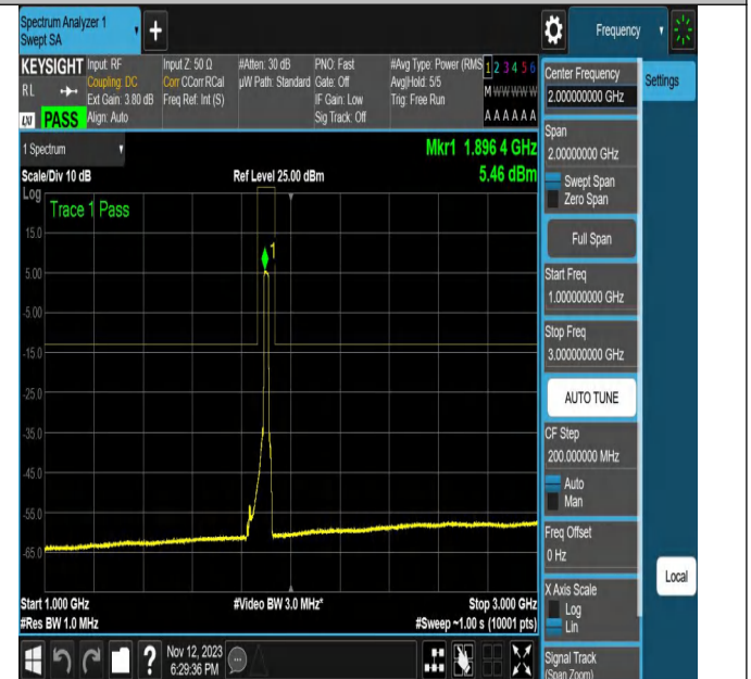
NTNV-N2-PC3-15-20-H-CP-256QAM-Outer_Full-Ant1-PASS
