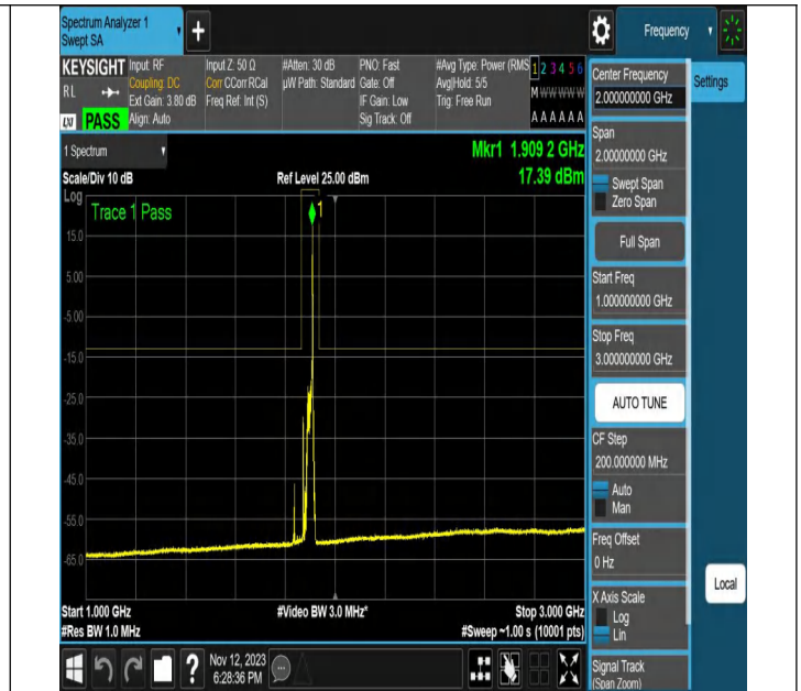
NTNV-N2-PC3-15-20-H-CP-64QAM-Edge_1RB_Right-Ant1-PA
