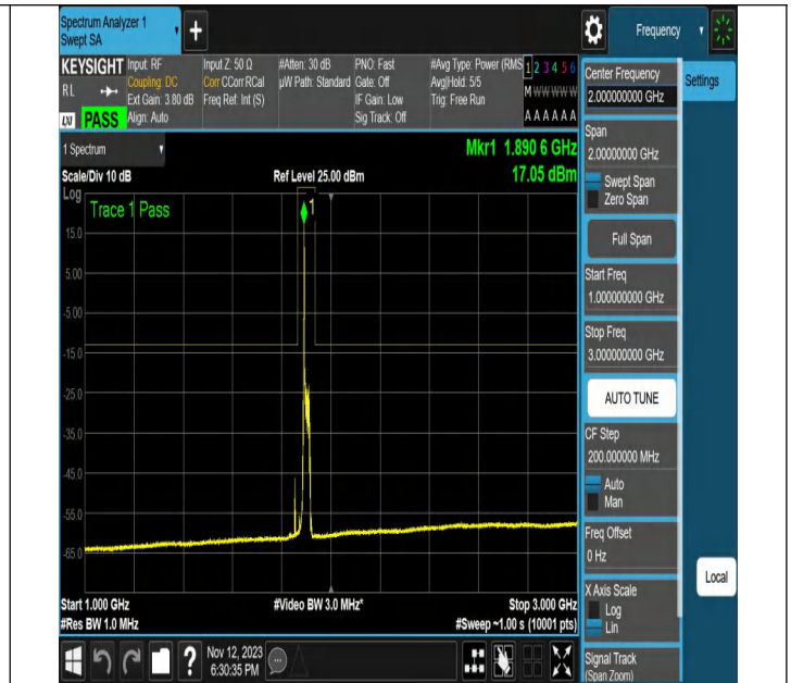
NTNV-N2-PC3-15-20-H-CP-256QAM-Edge_1RB_Left-Ant1-PAS
