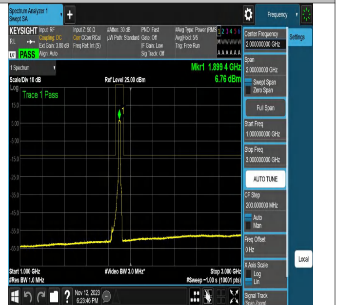
NTNV-N2-PC3-15-20-H-CP-16QAM-Outer_Full-Ant1-PASS
