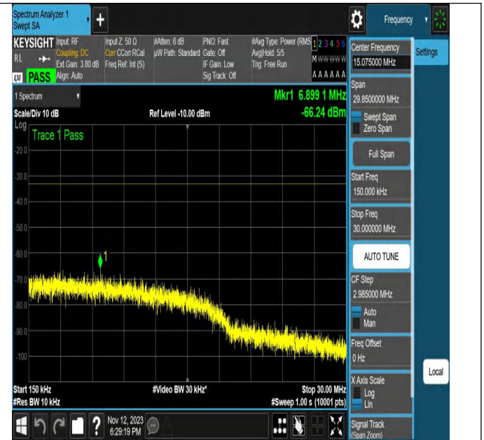
NTNV-N2-PC3-15-20-H-CP-256QAM-Outer_Full-Ant1-PASS
