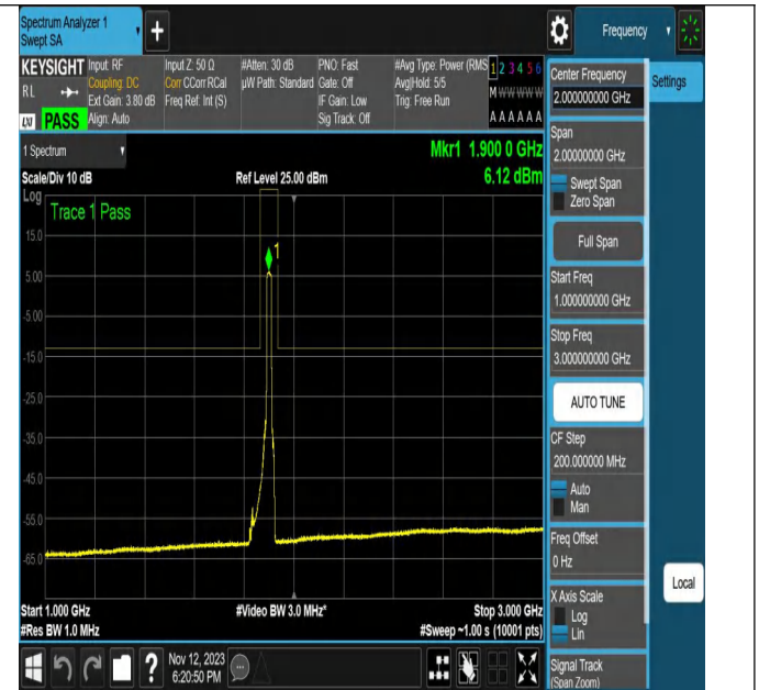
NTNV-N2-PC3-15-20-H-CP-QPSK-Outer_Full-Ant1-PASS
