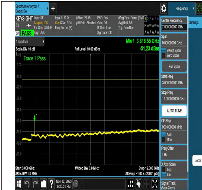
NTNV-N2-PC3-15-20-H-CP-16QAM-Edge_1RB_Right-Ant1-PA
