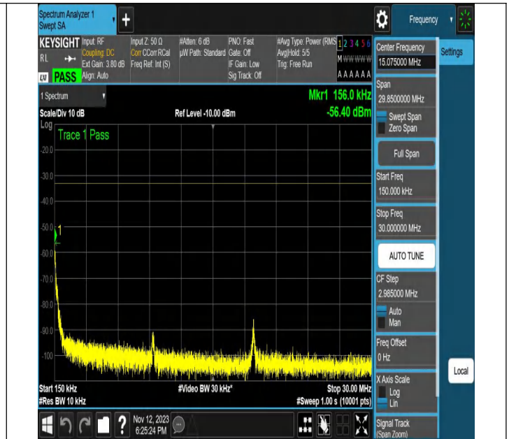
NTNV-N2-PC3-15-20-H-CP-16QAM-Edge_1RB_Right-Ant1-PA
