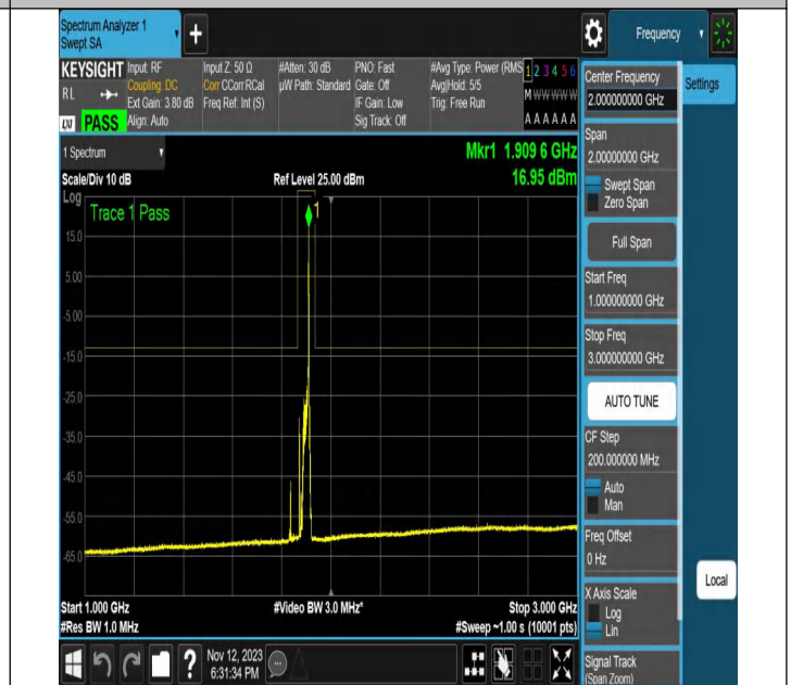
NTNV-N2-PC3-15-20-H-CP-256QAM-Edge_1RB_Right-Ant1-PA
