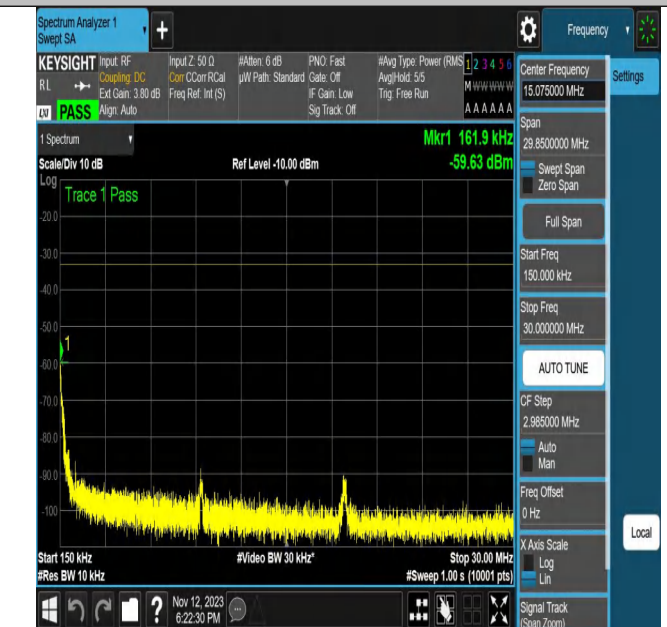
NTNV-N2-PC3-15-20-H-CP-QPSK-Edge_1RB_Right-Ant1-PAS
