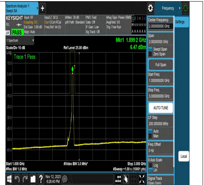
NTNV-N2-PC3-15-20-H-CP-64QAM-Outer_Full-Ant1-PASS
