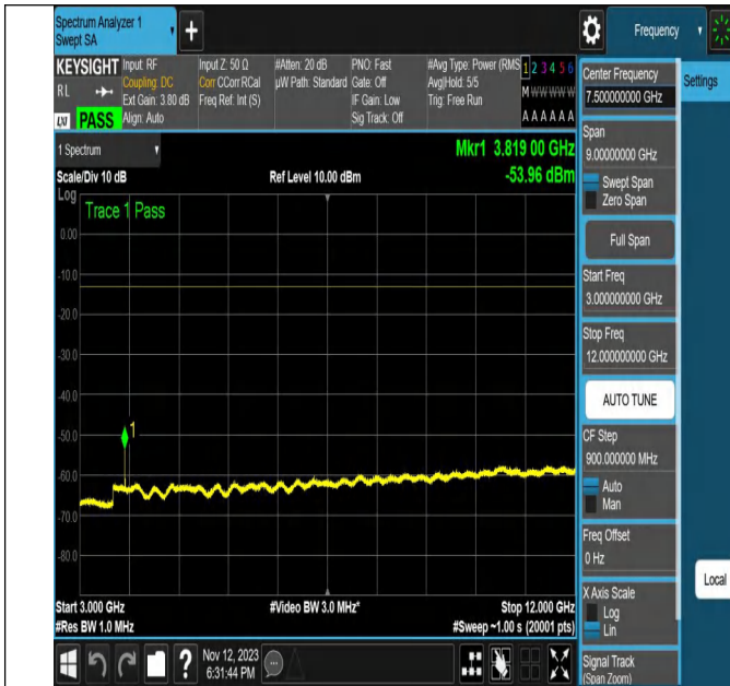
NTNV-N2-PC3-15-20-H-CP-256QAM-Edge_1RB_Right-Ant1-PA
