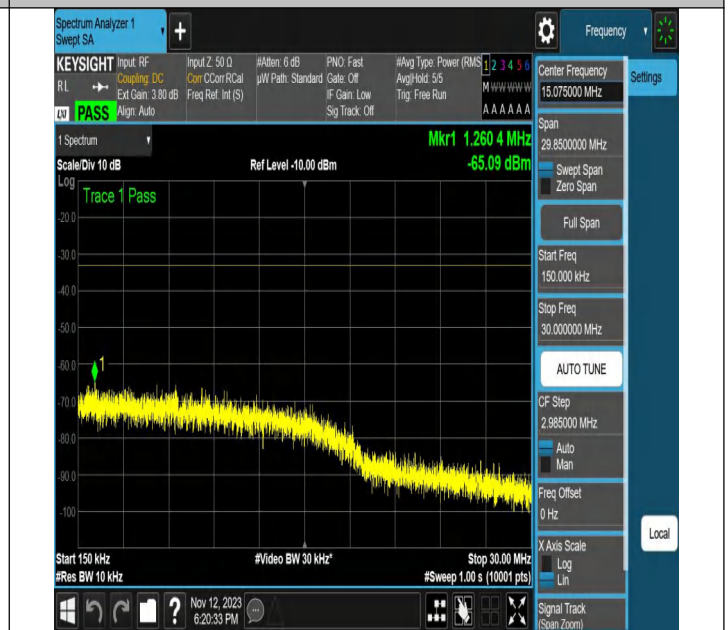
NTVN-N2-PC3-15-20-H-CP-QPSK-Outer_Full-Ant1-PASS
