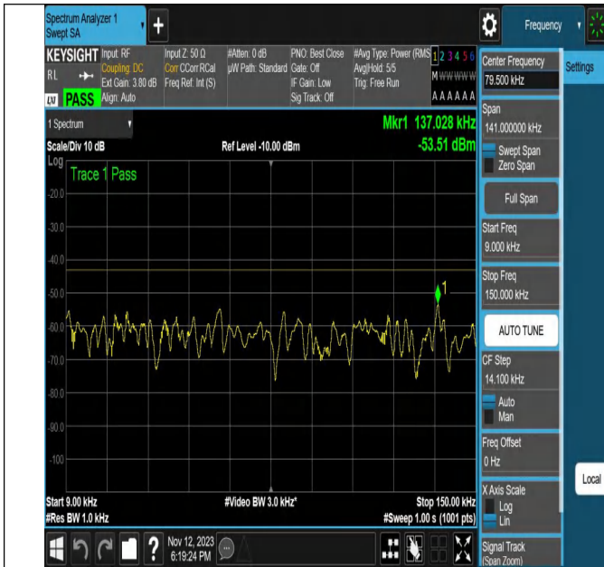
NTNV-N2-PC3-15-20-H-DFT-256QAM-Edge_1RB_Right-Ant1-P
