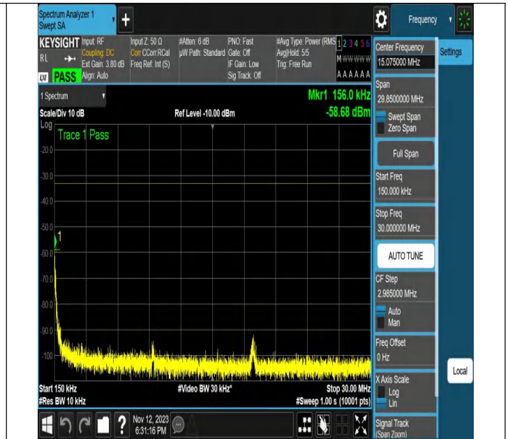
NTNV-N2-PC3-15-20-H-CP-256QAM-Edge_1RB_Right-Ant1-PA
