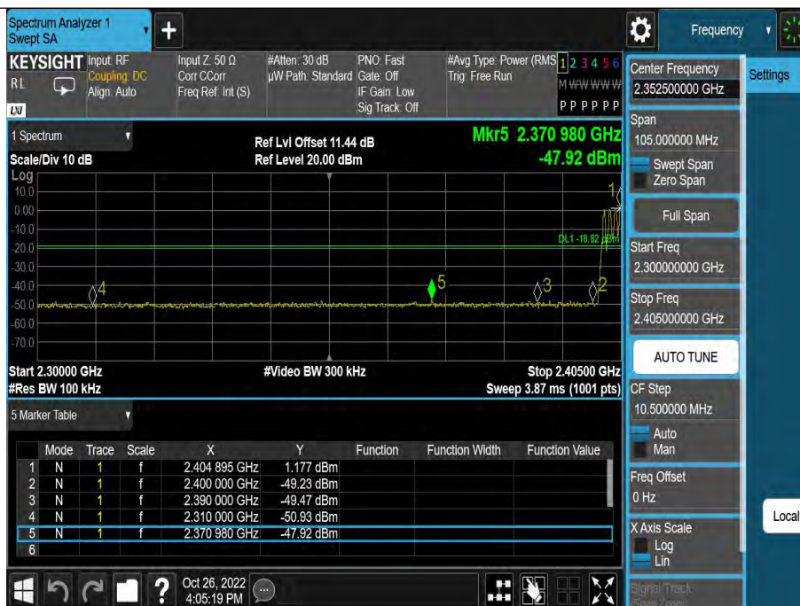
DH5-Ant1-Low-Hop_2402-1.18
