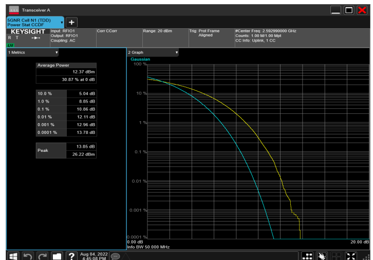
n41_40MHz_30kHz_2592.99MHz_CP-OFDM 256 QAM_RB106@0
