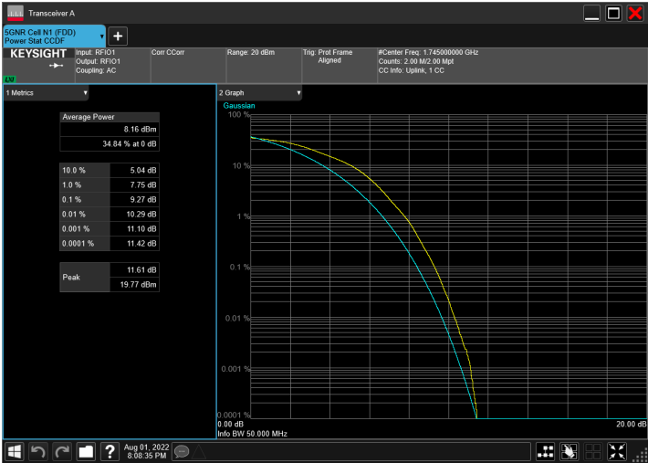
n66_40MHz_15kHz_1745MHz_DFT-s-OFDM 16 QAM_RB216@0
