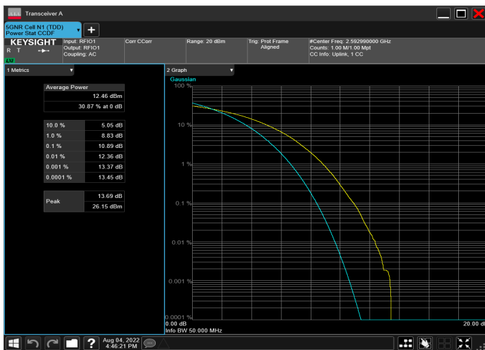
n41_50MHz_30kHz_2592.99MHz_CP-OFDM 256 QAM_RB133@0
