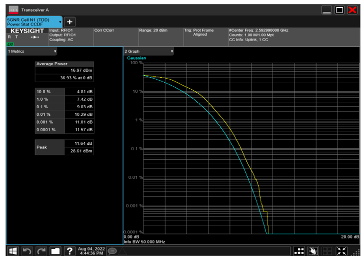
n41_40MHz_30kHz_2592.99MHz_DFT-s-OFDM 16 QAM_RB100@0
