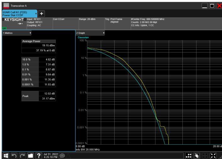
n71_15MHz_15kHz_680.5MHz_DFT-s-OFDM 16 QAM_RB75@0
