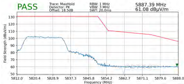
Plot 7-293. Radiated Upper Band Edge Plot MIMO (Peak – UNII Band 3)
