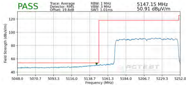
Plot 7-305. Radiated Lower Band Edge Plot MIMO (Average – UNII Band 1)
