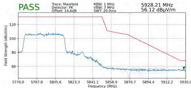
Plot 7-302. Radiated Upper Band Edge Plot MIMO (Peak – UNII Band 3)
