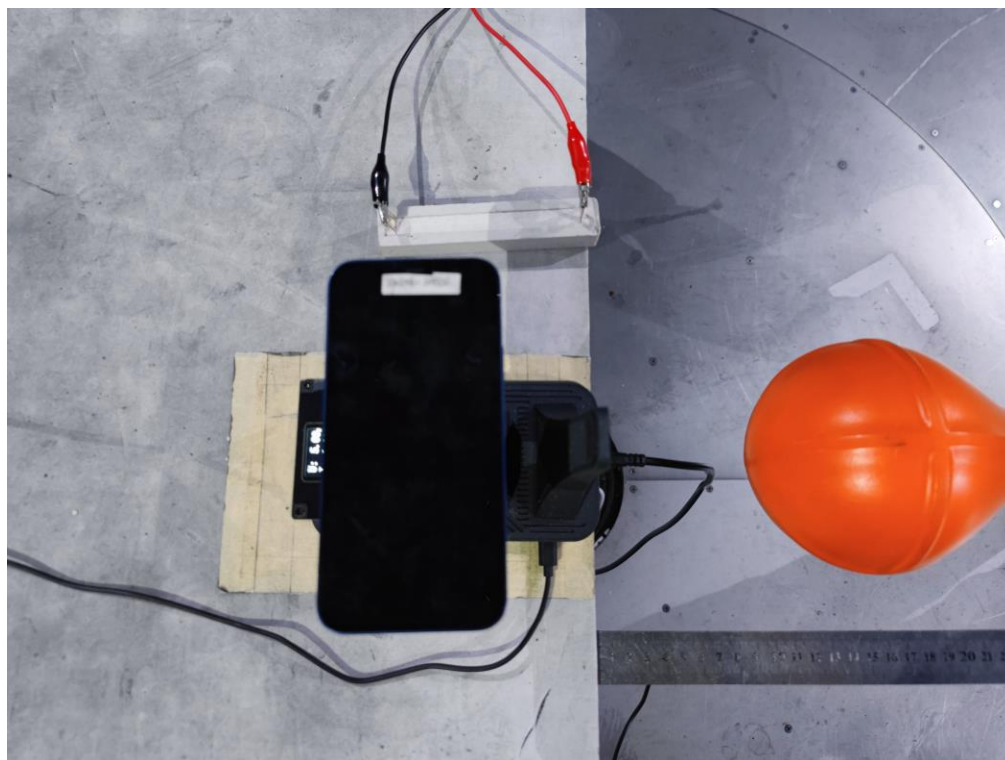
H-Field &amp; E-Field Strength_ Position C
