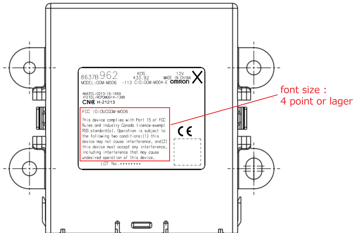
Figure 9.2 GGM-M006 appearance
