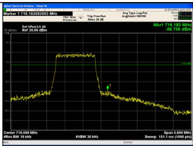
LTE Band 12 - High Channel QPSK-1.4
