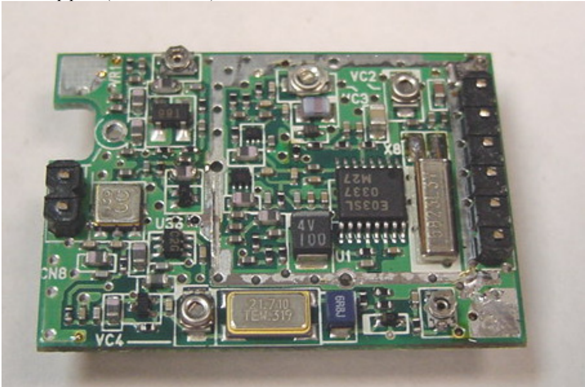
3. Synthesizer top parts (shield removed)
