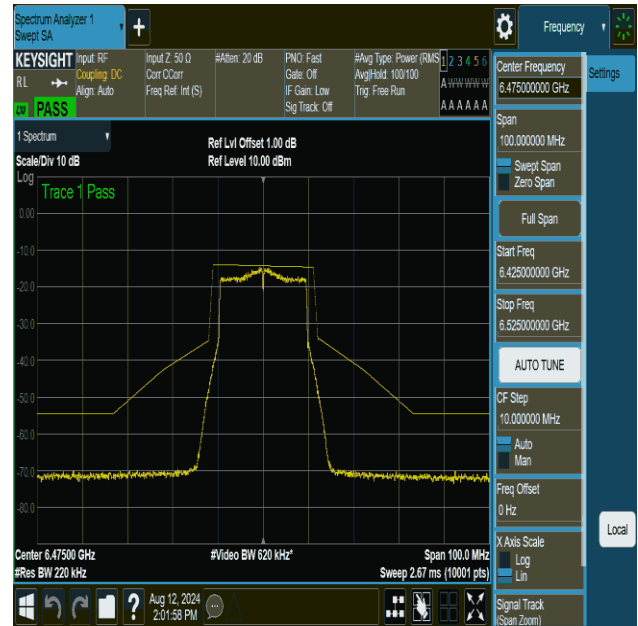
NTVN-11be20MIMO-Ant2-6475-PASS
