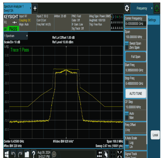
NTNV-11ax20MIMO-Ant2-6435-PASS
