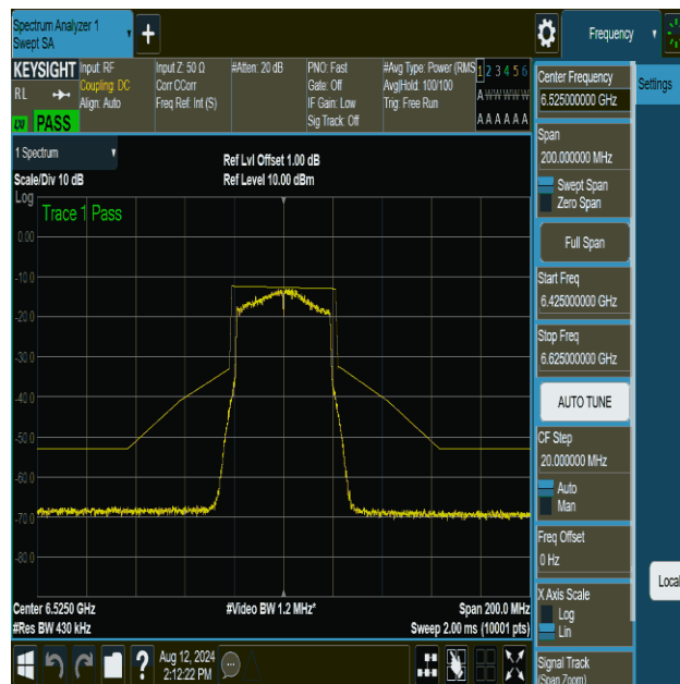
NTVN-11be40MIMO-Ant2-6525-PASS
