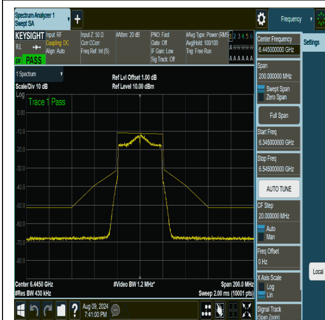
NTNV-11ax40MIMO-Ant1-6445-PASS
