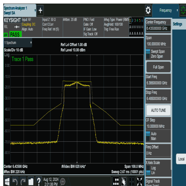
NTNV-11be20MIMO-Ant2-6435-PASS
