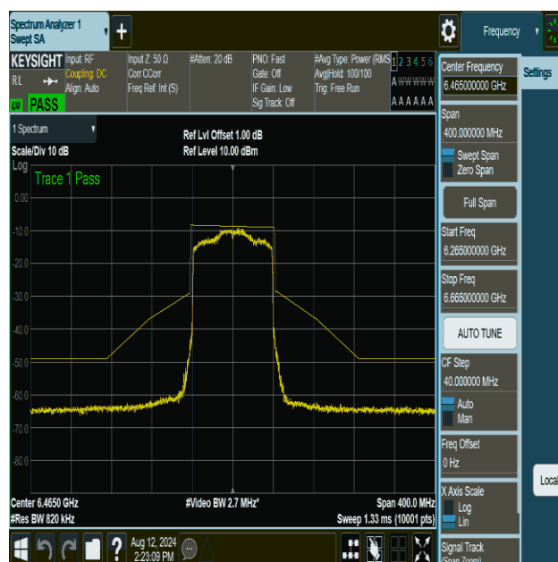
NTVN-11be80MIMO-Ant2-6465-PASS
