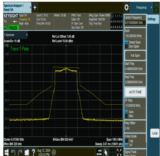
NTVN-11be20MIMO-Ant2-6515-PASS
