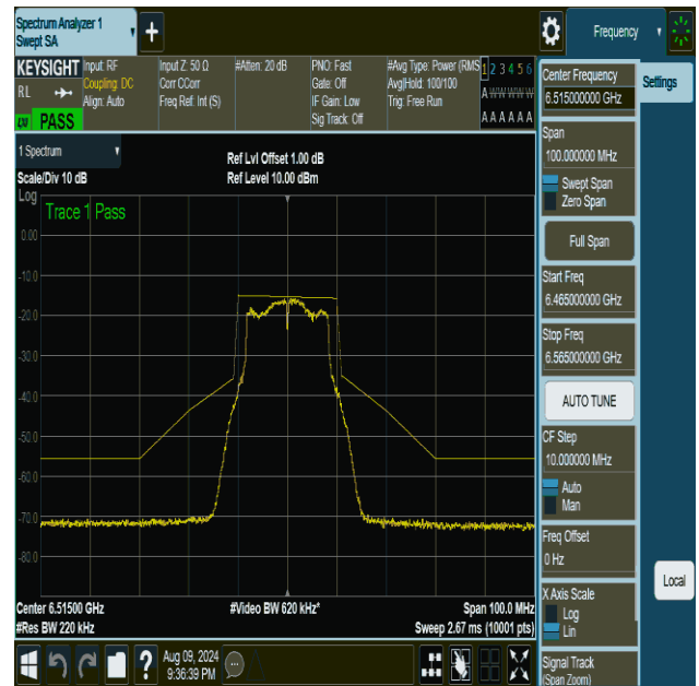
NTNV-11a-CDD-Ant2-6515-PASS
