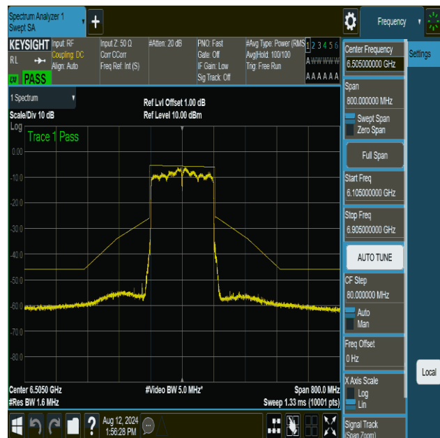
NTNV-11ax160MIMO-Ant2-6505-PASS
