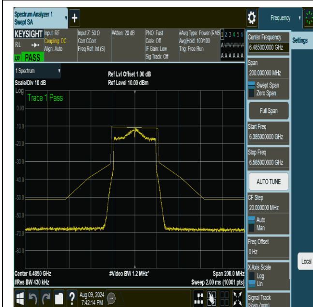
NTNV-11ax40MIMO-Ant1-6485-PASS
