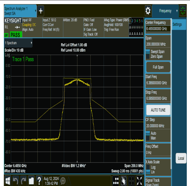
NTNV-11ax40MIMO-Ant2-6485-PASS
