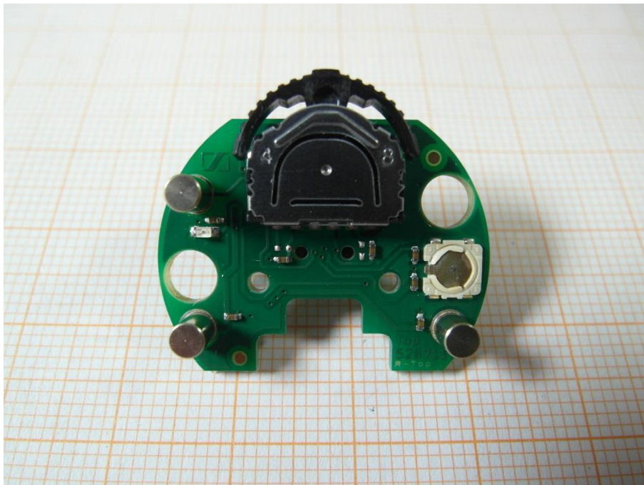
Photo 5: control & power buttons
