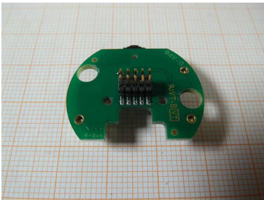
Photo 6: backside of the part above
