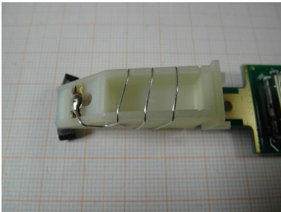
Photo 10: antenna
