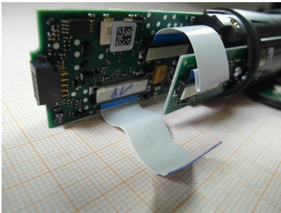
Photo 4: EUT control & RF part
