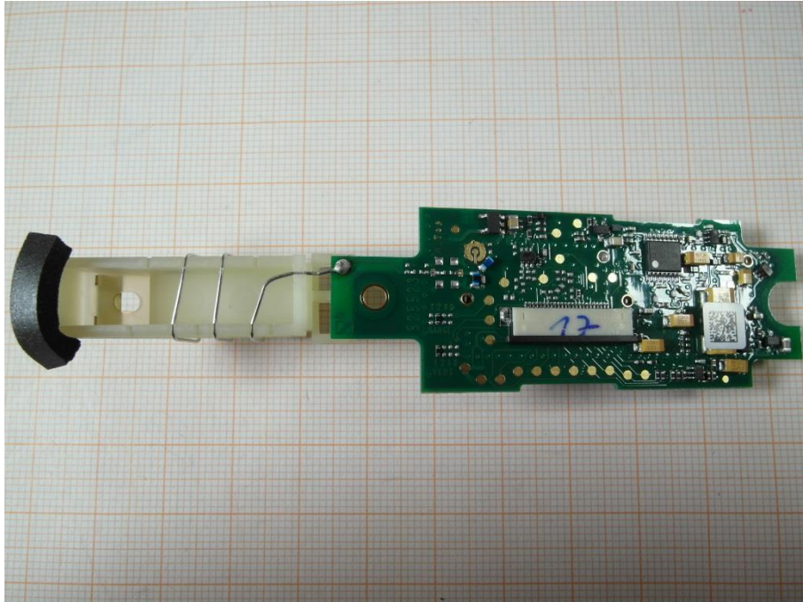
Photo 9: RF part with antenna backside
