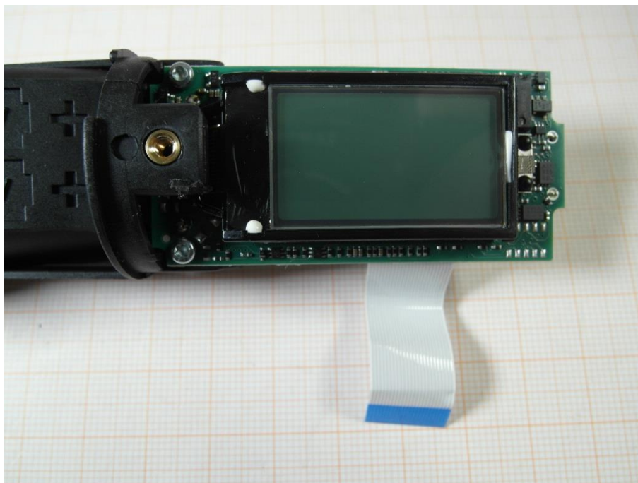
Photo 2: display
