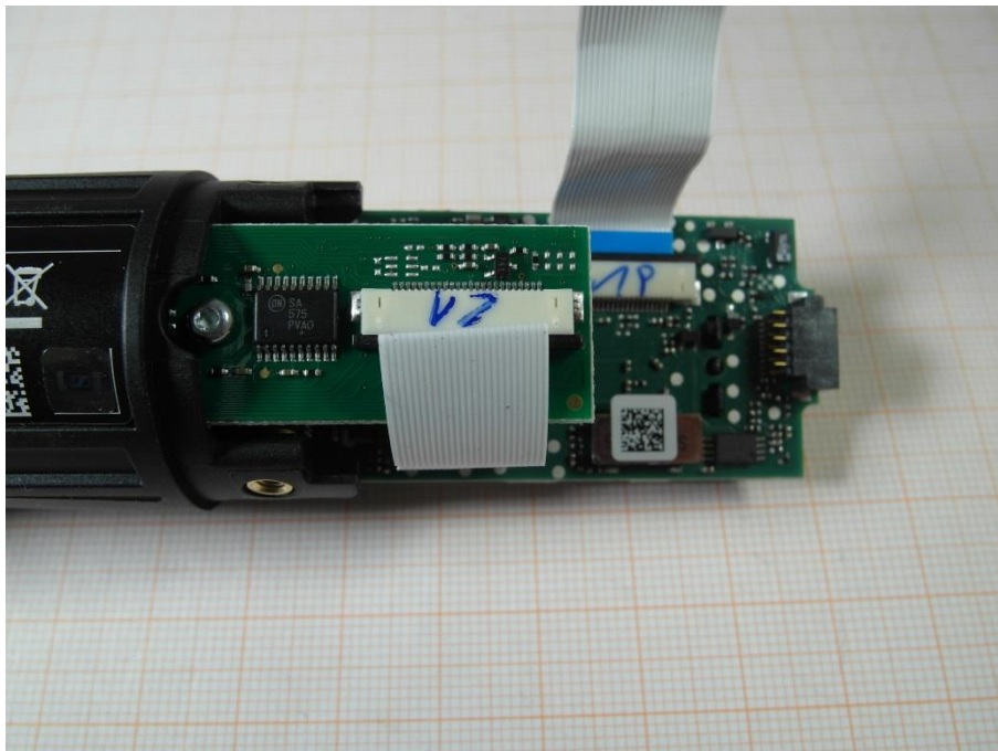
Photo 3: EUT control & RF part
