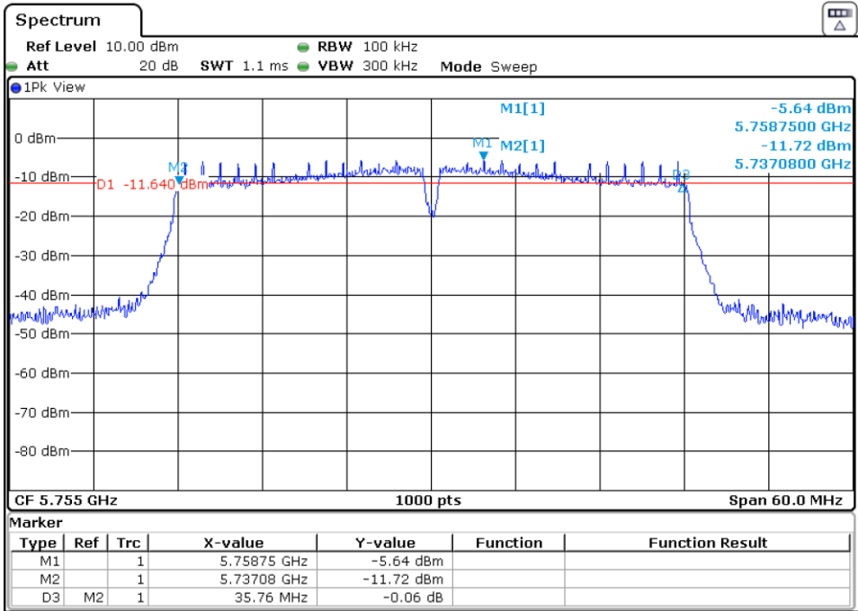
Port 1 Antenna
