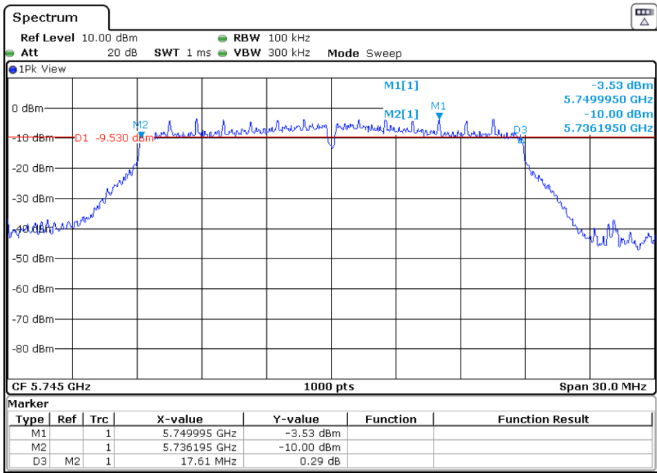
Port 1 Antenna
