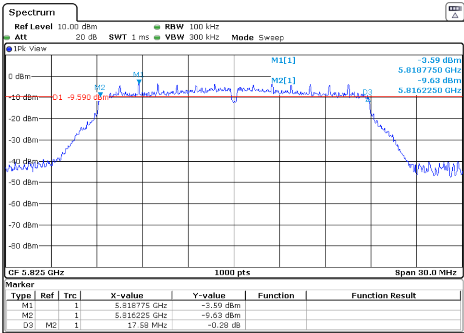
Port 1 Antenna
