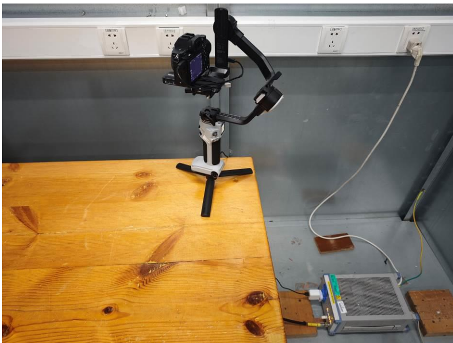
4. Conducted Emission (Part 15B, Normal Working)
