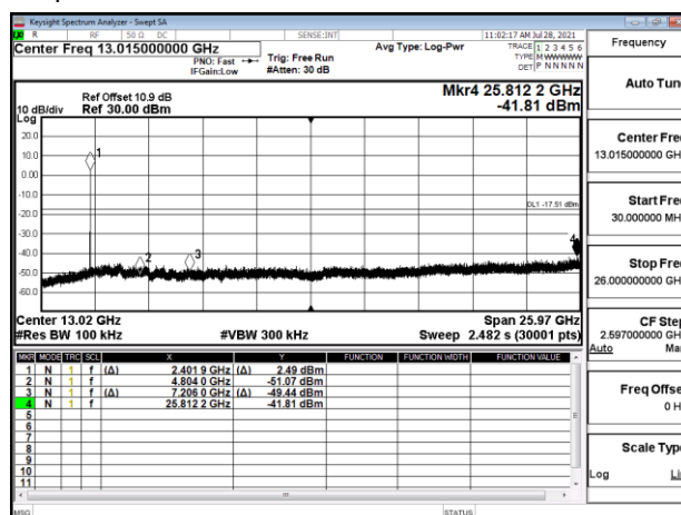
Spurious Emission_pi/4-DQPSK_2M_DH5_2402MHz
