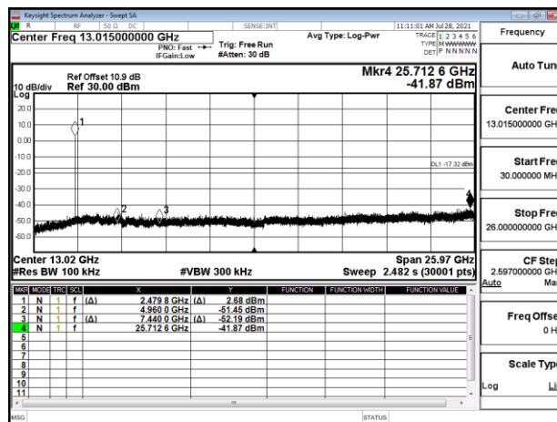
Spurious Emission_8DPSK_3M_DH5_2480MHz
