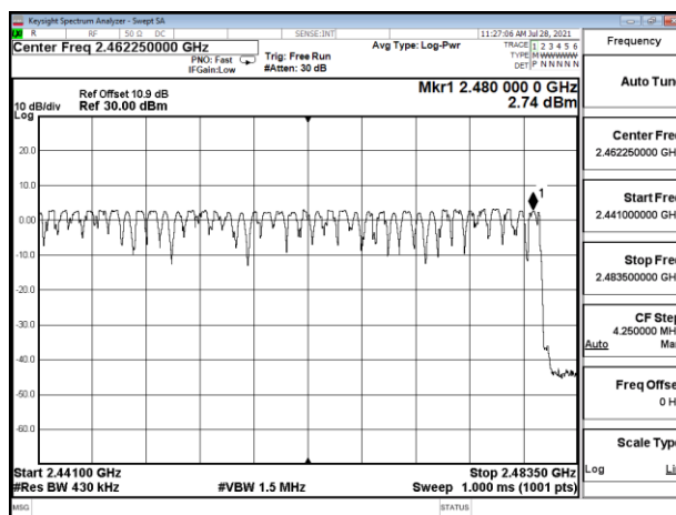
8DPSK_3M_DH5_2441-2480
