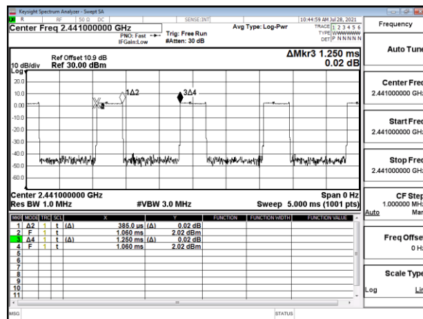
Dwell Time_π/4-DQPSK_2M_DH3_2441MHz
