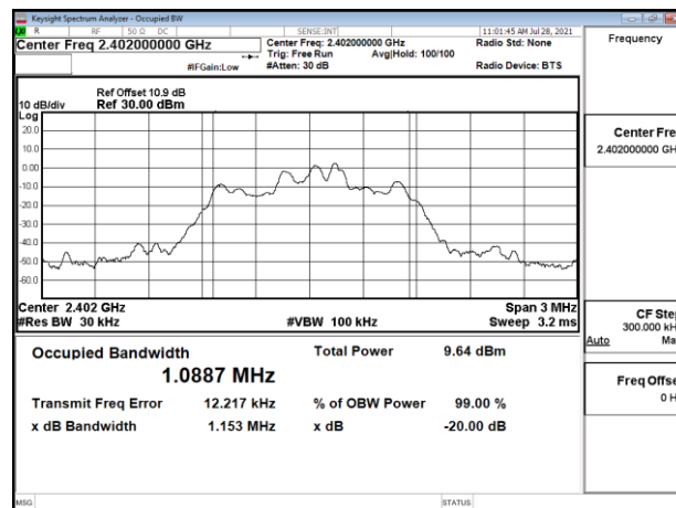
OBW 20dB_π/4-DQPSK_2M_DH5_2402MHz
