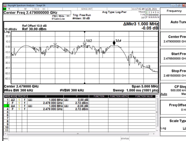
8DPSK_3M_DH5_CH76CH77CH78
