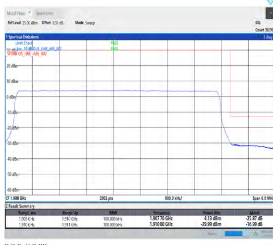
1-N2-PC3-15-5-H-6-CP-QPSK-Outer_Full-25@0-A nt1-1-seegraph-PASS-see graph
