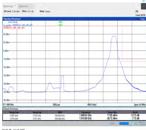
1-N2-PC3-15-5-H-2-DFT-PI2BPSK-Edge_1RB_Right-1 @24-Ant1-1-seegraph-PASS-see graph
