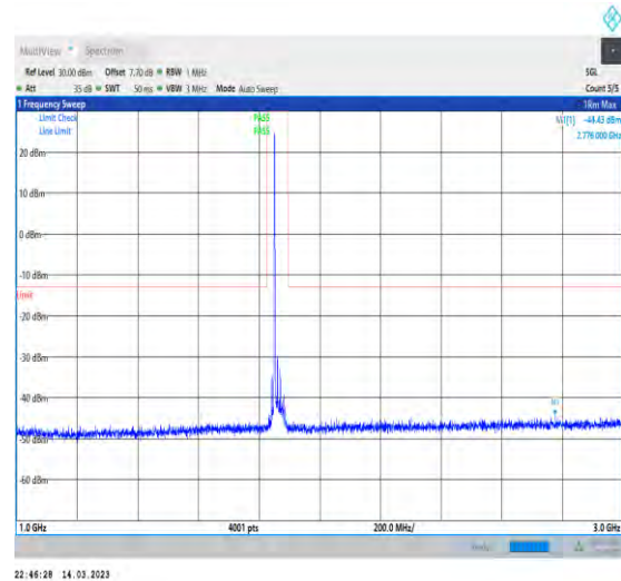
1-N2-PC3-15-20-L-1-DFT-PI2BPSK-Inner_1RB_Left- 1@1-1000-3000-Ant1-2776.00--44.43--13-PASS
