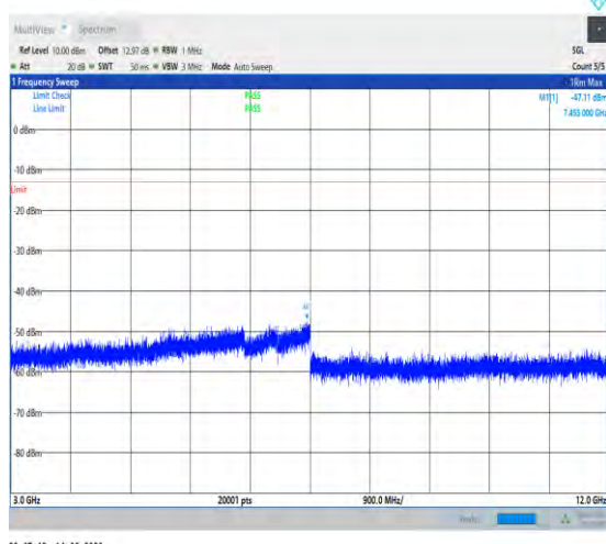
1-N2-PC3-15-20-M-1-DFT-PI2BPSK-Inner_1RB_Lef t-1@1-3000-12000-Ant1-7455.00--47.11--13-PASS
