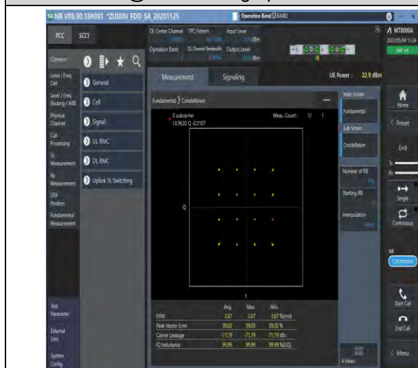
1-N2-PC3-15-20-M-3-DFT-16QAM-Outter_Full-100@ 0-Ant1-see graph-PASS
