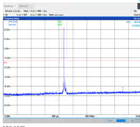
1-N2-PC3-15-20-M-1-DFT-PI2BPSK-Inner_1RB_Left- 1@1-1000-3000-Ant1-2716.50--44.35--13-PASS
