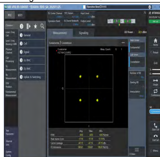
1-N2-PC3-15-20-M-6-CP-QPSK-Outer_Full-106@0- Ant1-see graph-PASS
