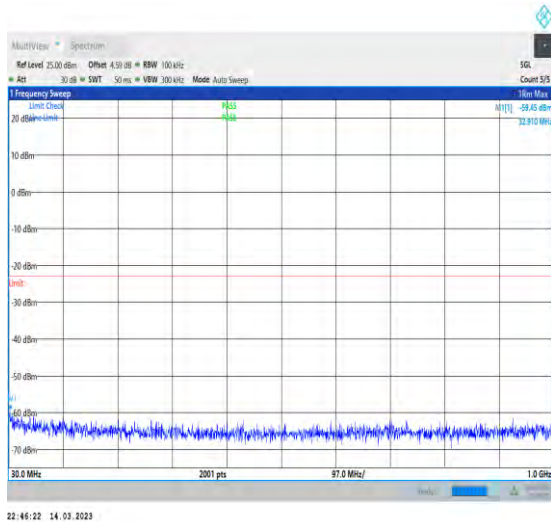
1-N2-PC3-15-20-L-1-DFT-PI2BPSK-Inner_1RB_Left -1@1-30-1000-Ant1-32.91--59.45--23-PASS
