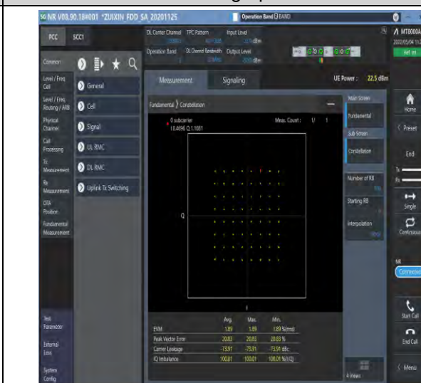
1-N2-PC3-15-20-M-4-DFT-64QAM-Outter_Full-100 @0-Ant1-see graph-PASS
