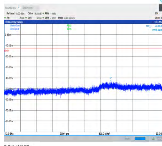
1-N2-PC3-15-20-L-1-DFT-PI2BPSK-Inner_1RB_Left-1@1-12000-20000-Ant1-17312.00--43.56--13-PASS
