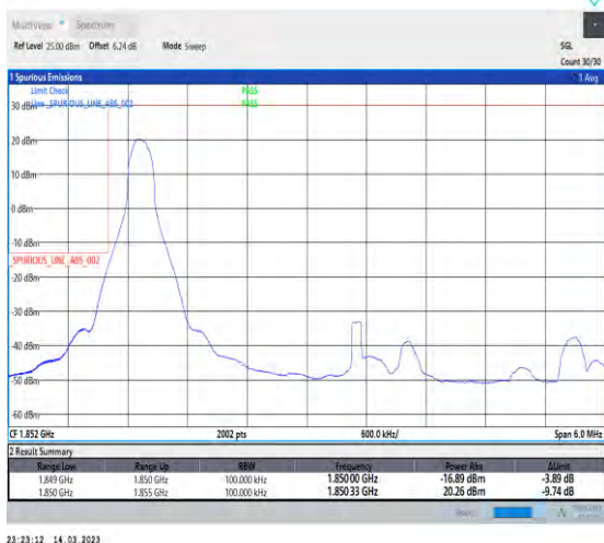
1-N2-PC3-15-5-L-1-DFT-PI2BPSK-Edge_1RB_Left-1 @0-Ant1-1-seegraph-PASS-see graph
