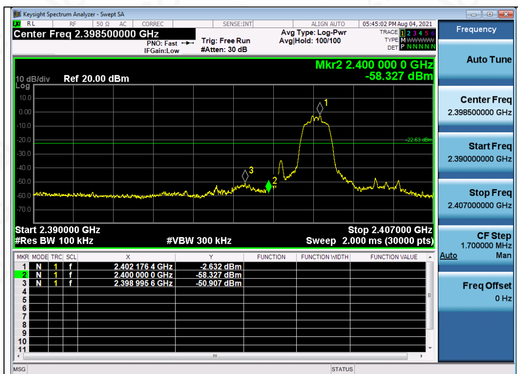
Test Graph EDR ANT1 2402 2Mbps Lower Band Edge Emissions
