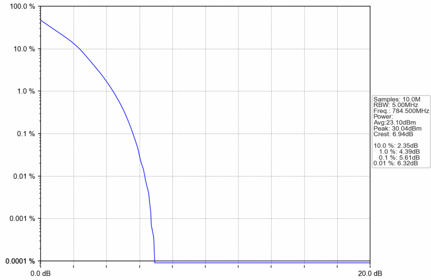
Band13_5MHz_QPSK_HCH_784.5MHz_RB_25_0_NTNV
