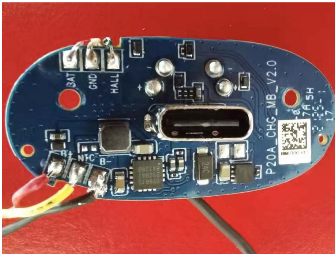
Charger internal photos
