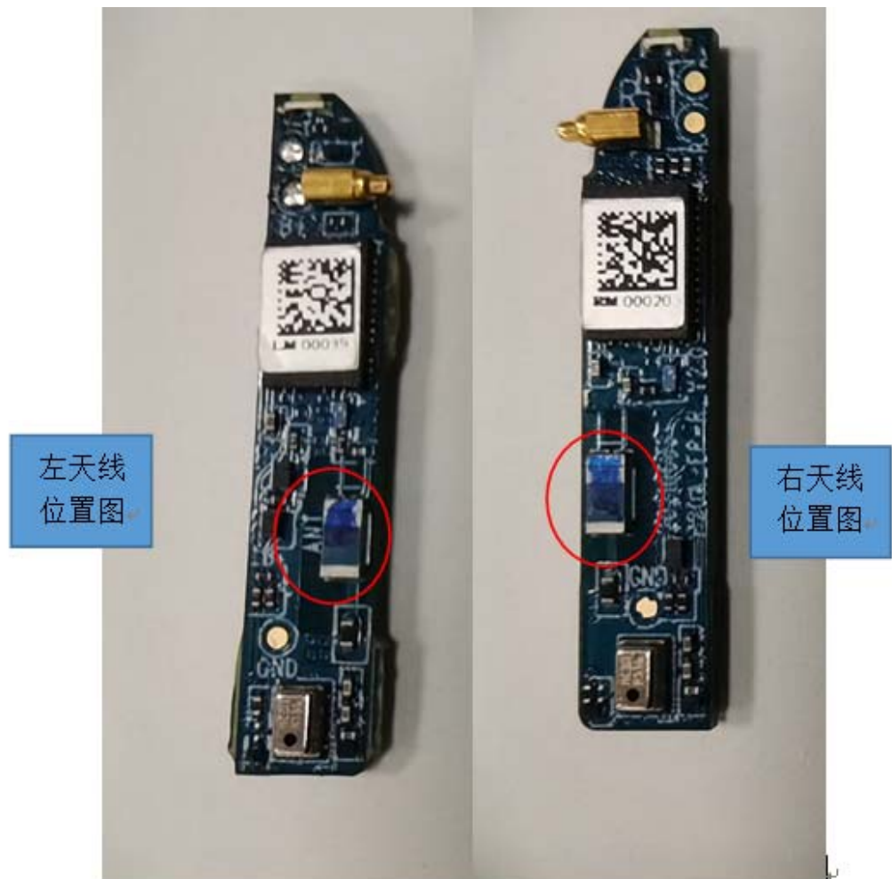
Location diagram of left earphone antenna
