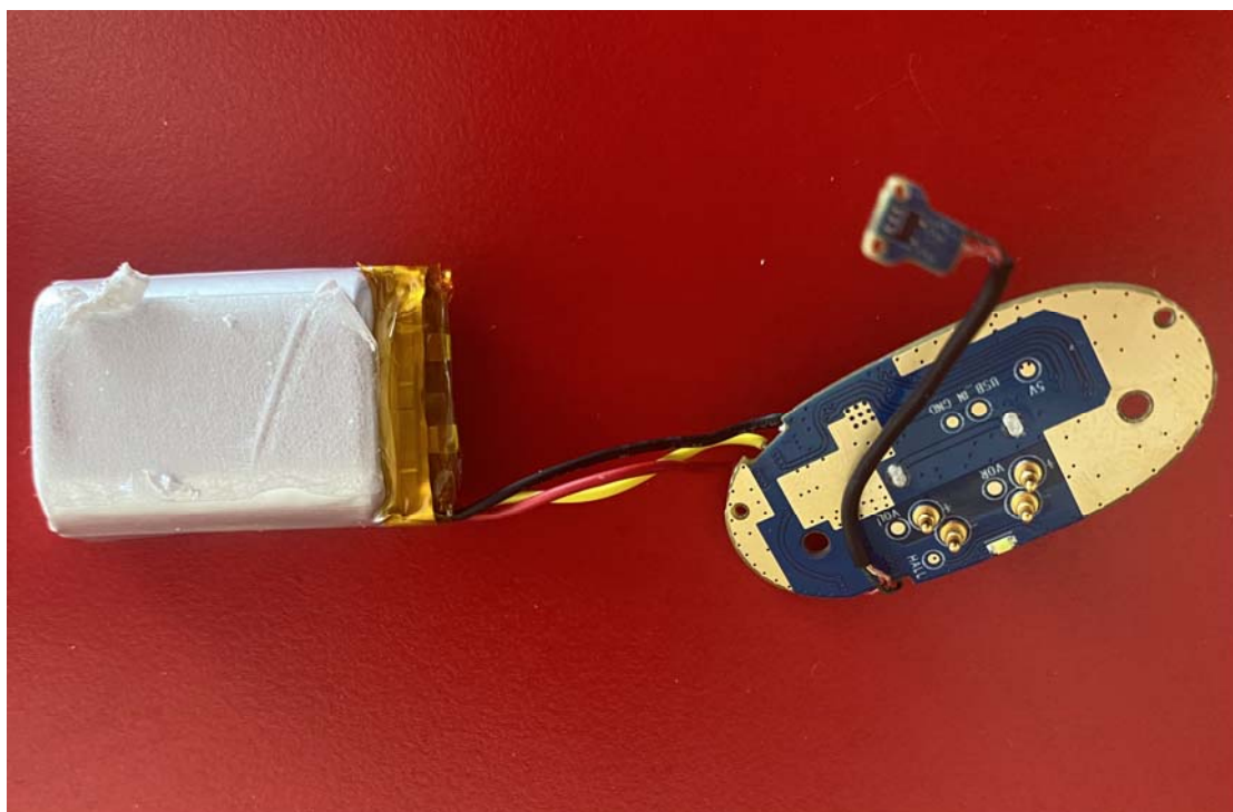
Charger internal photos
