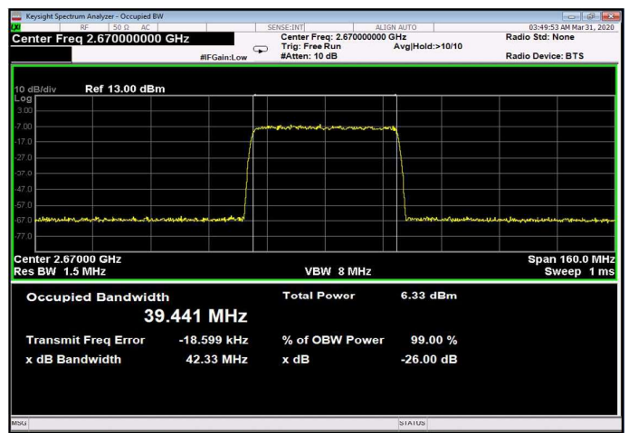
Figure 288: 256QAM 40MHz B.W.; 2670.0MHz, 15kHz Input
