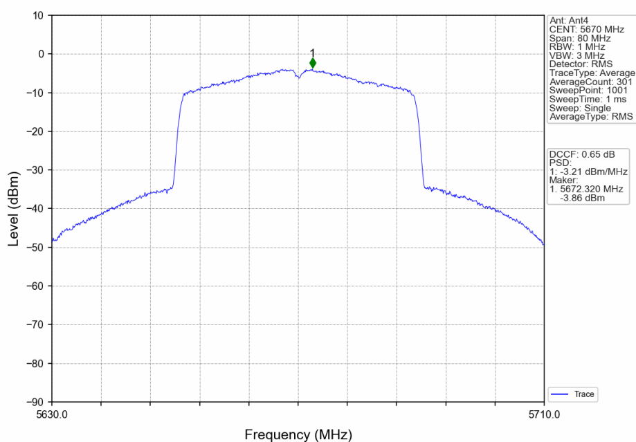
802.11ax(HEW40)_HCH_5670MHz_RU484_Left_Ant4_NTNV
