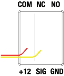
Figure 5. Contact for Self-Powered Voltage Source Device
