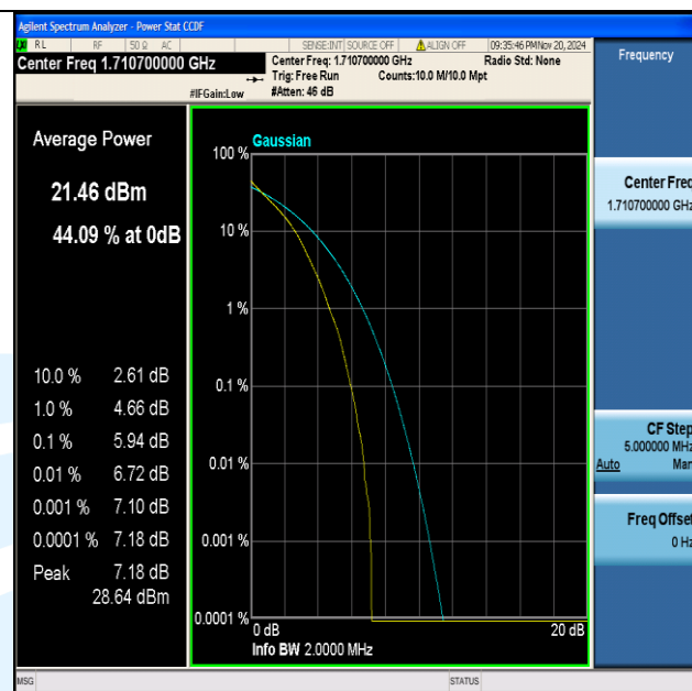
Band66-1.4MHz-QPSK-131979-6RB#0-PASS
