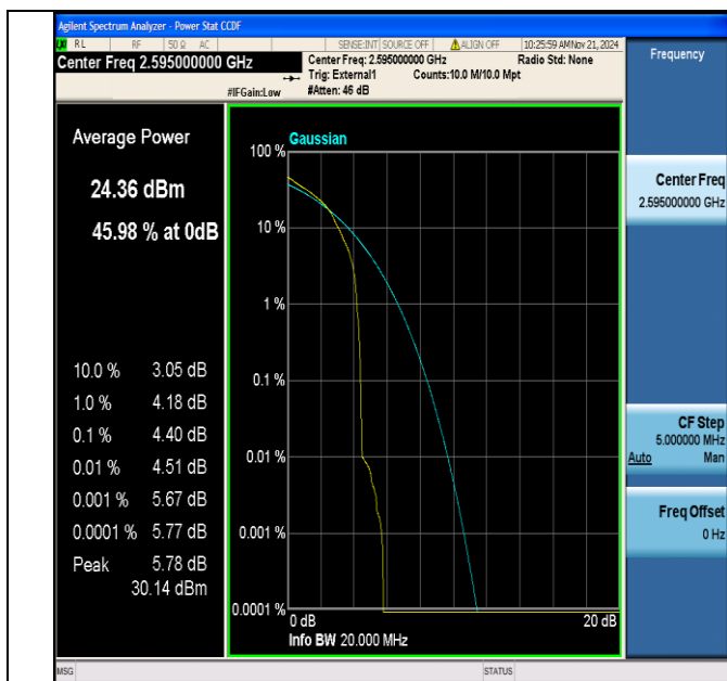
Band38-20MHz-16QAM-38000-1RB#0-PASS
