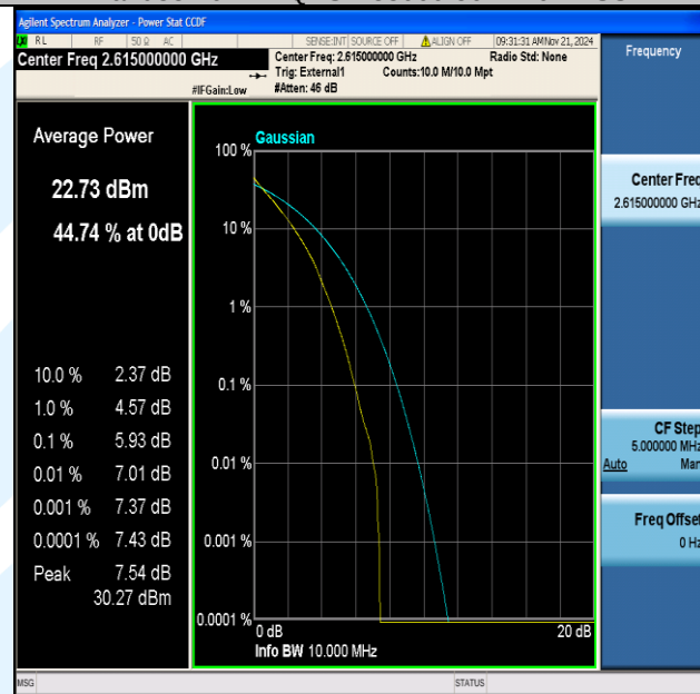
Band38-10MHz-QPSK-38200-50RB#0-PASS
