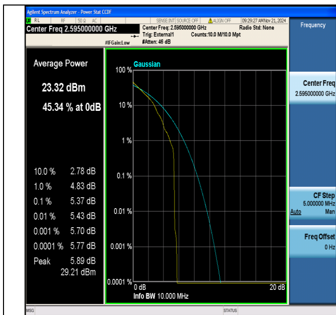
Band38-10MHz-QPSK-38000-1RB#0-PASS
