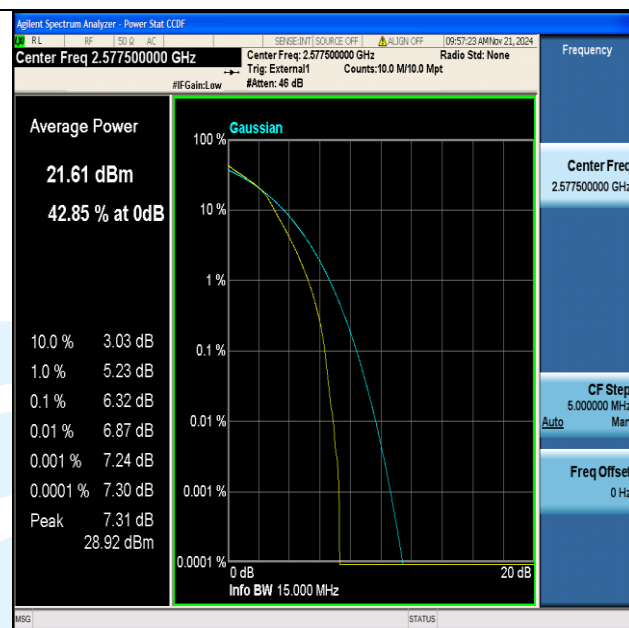
Band38-15MHz-16QAM-37825-75RB#0-PASS
