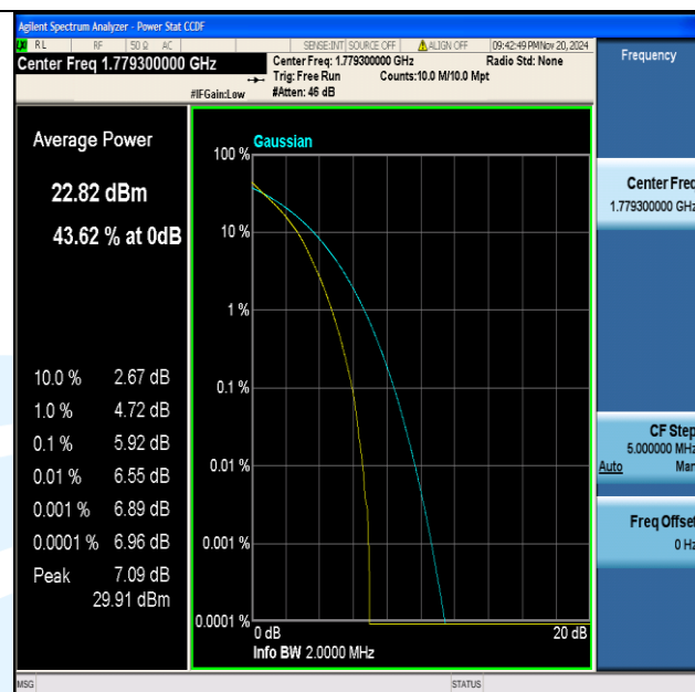
Band66-1.4MHz-QPSK-132665-6RB#0-PASS
