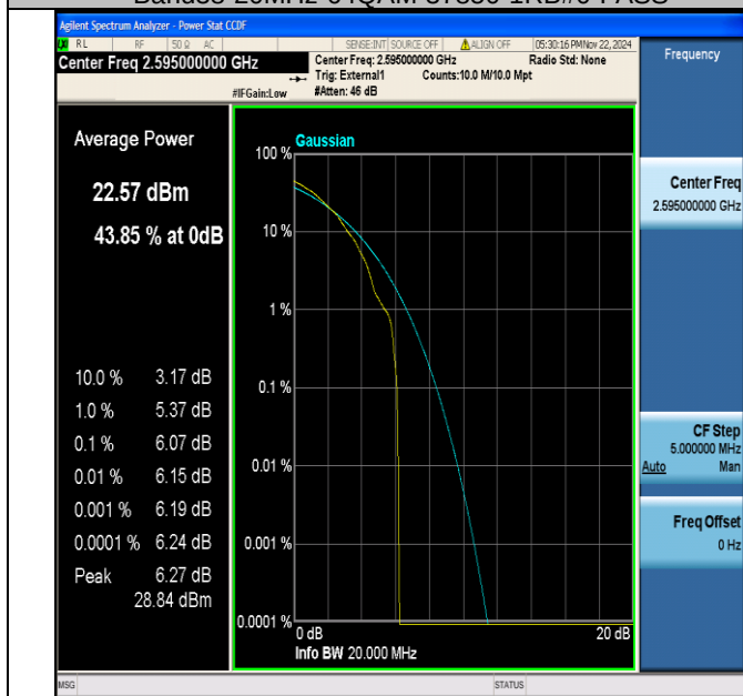
Band38-20MHz-64QAM-38000-1RB#0-PASS
