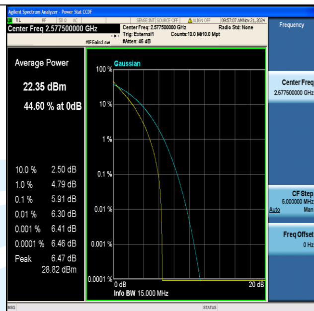
Band38-15MHz-QPSK-37825-75RB#0-PASS
