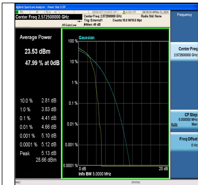
Band38-5MHz-16QAM-37775-1RB#0-PASS
