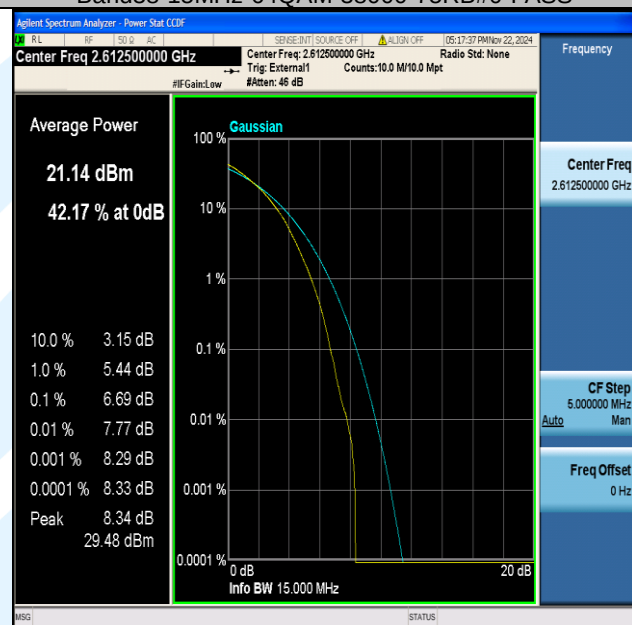
Band38-15MHz-64QAM-38175-75RB#0-PASS
