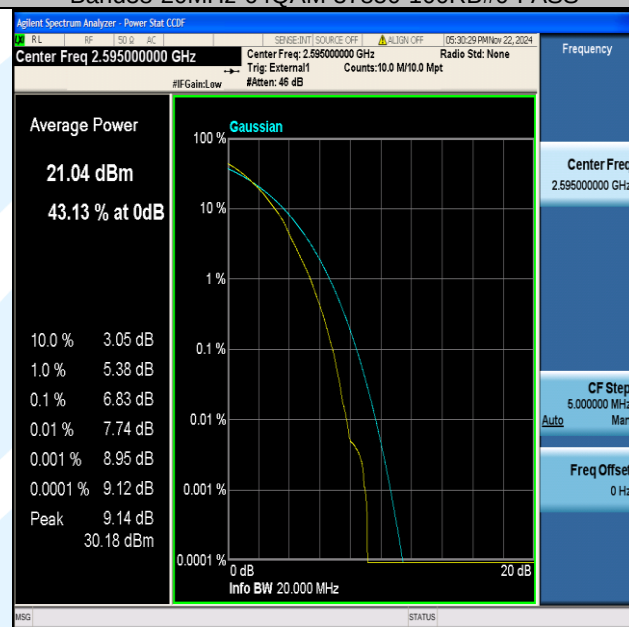
Band38-20MHz-64QAM-38000-100RB#0-PASS
