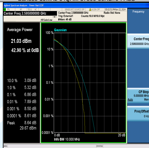
Band38-10MHz-64QAM-38000-50RB#0-PASS
