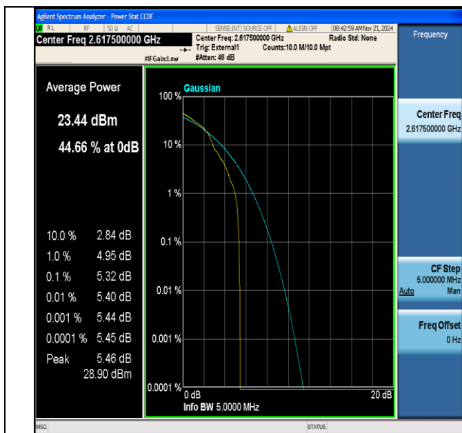
Band38-5MHz-16QAM-38225-1RB#0-PASS
