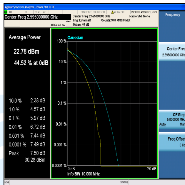
Band38-10MHz-QPSK-38000-50RB#0-PASS
