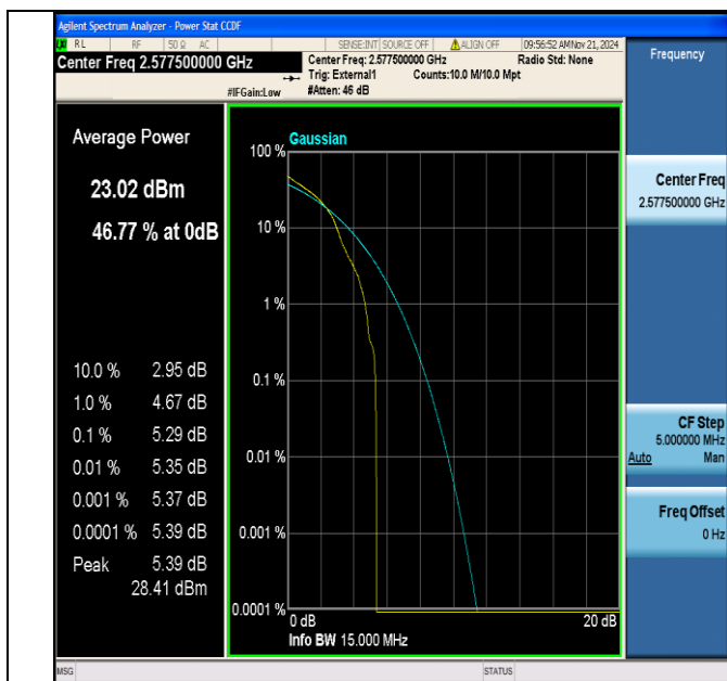
Band38-15MHz-16QAM-37825-1RB#0-PASS
