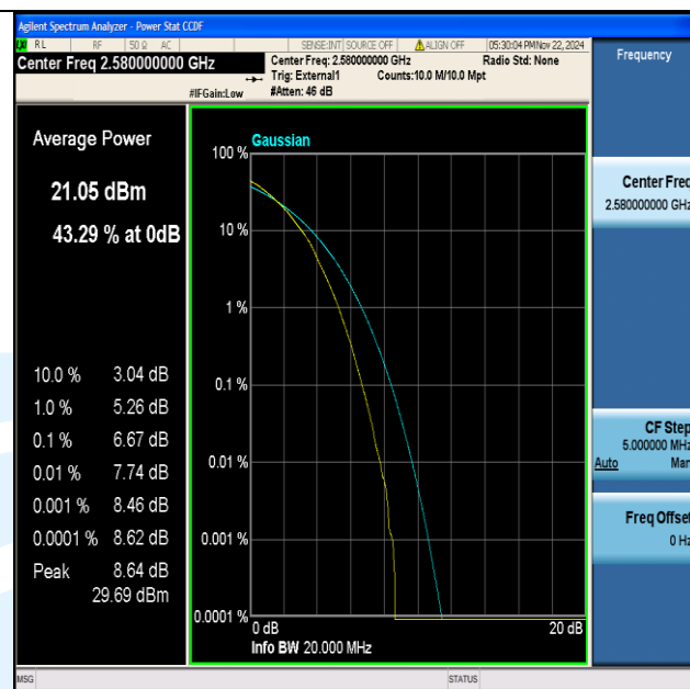
Band38-20MHz-64QAM-37850-100RB#0-PASS
