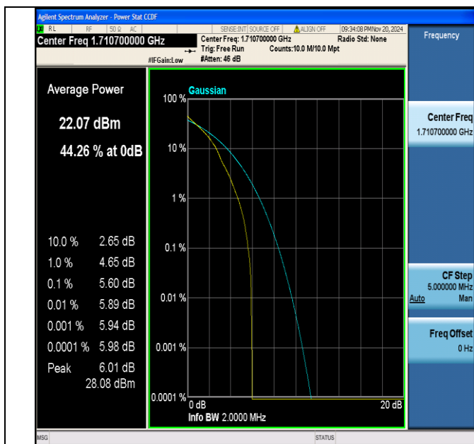
Band66-1.4MHz-QPSK-131979-1RB#0-PASS
