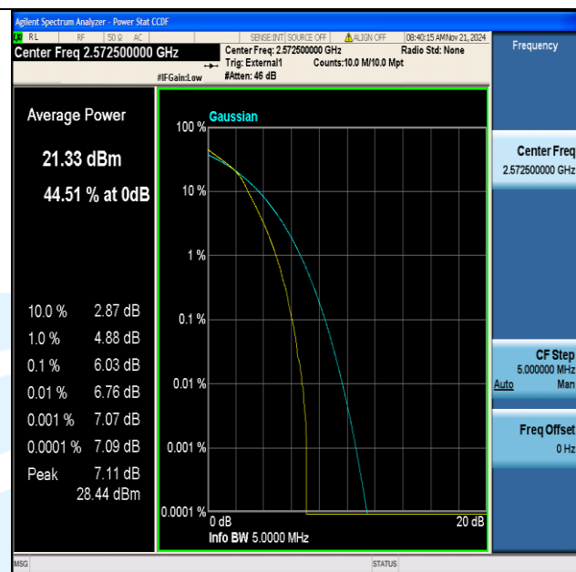
Band38-5MHz-16QAM-37775-25RB#0-PASS
