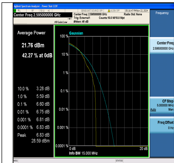
Band38-15MHz-64QAM-38000-1RB#0-PASS
