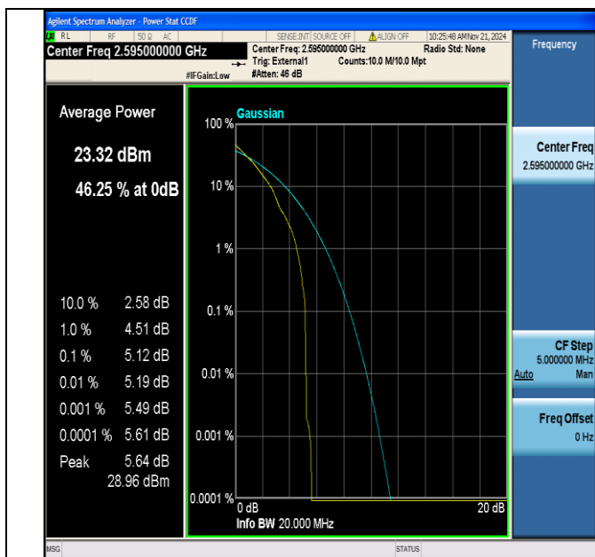
Band38-20MHz-QPSK-38000-1RB#0-PASS
