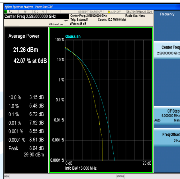
Band38-15MHz-64QAM-38000-75RB#0-PASS
