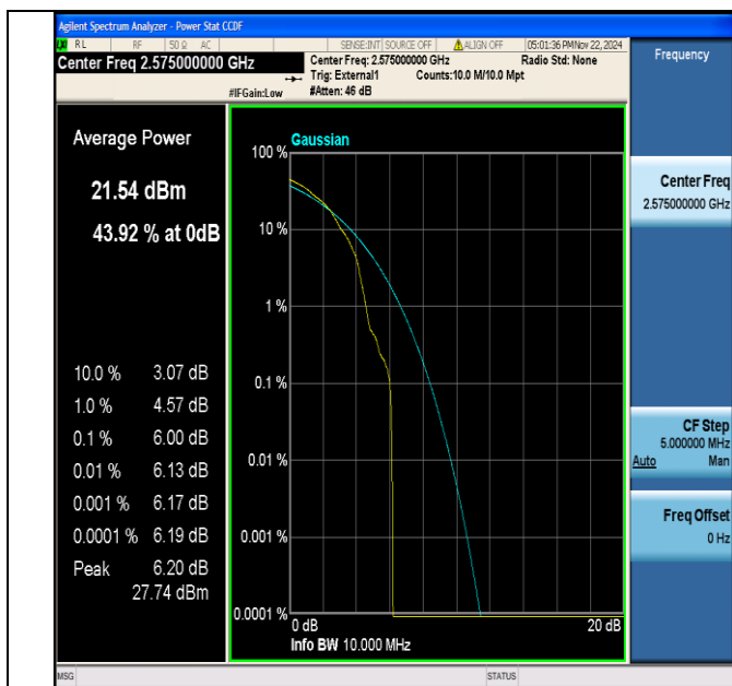
Band38-10MHz-64QAM-37800-1RB#0-PASS
