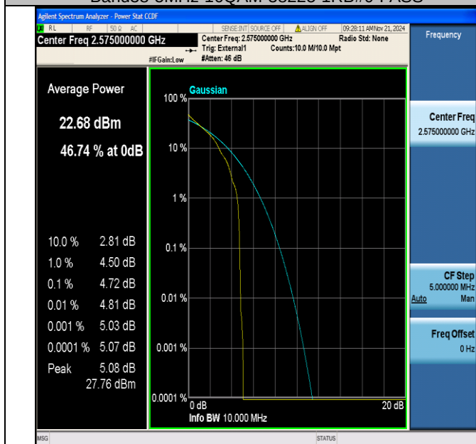
Band38-10MHz-QPSK-37800-1RB#0-PASS
