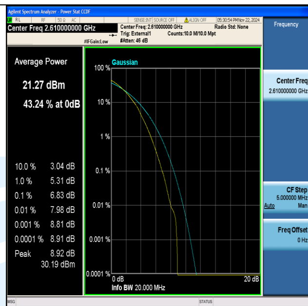
Band38-20MHz-64QAM-38150-100RB#0-PASS
