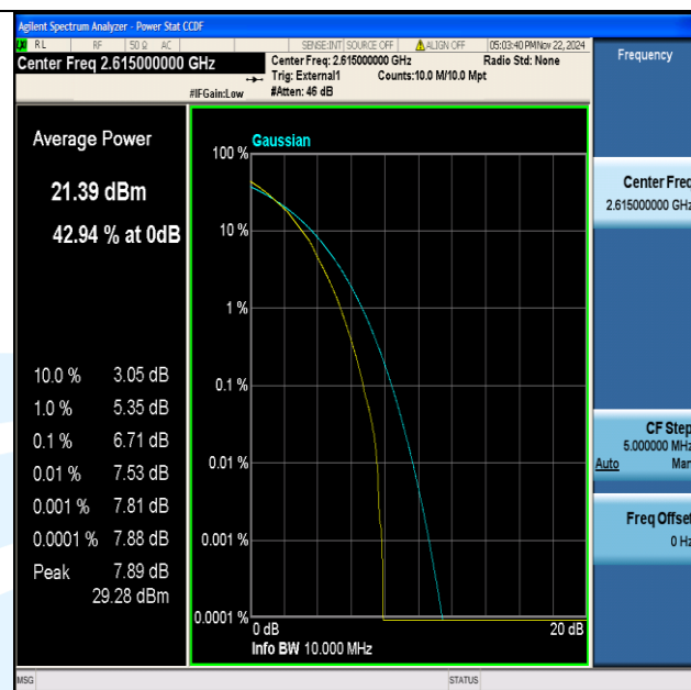
Band38-10MHz-64QAM-38200-50RB#0-PASS
