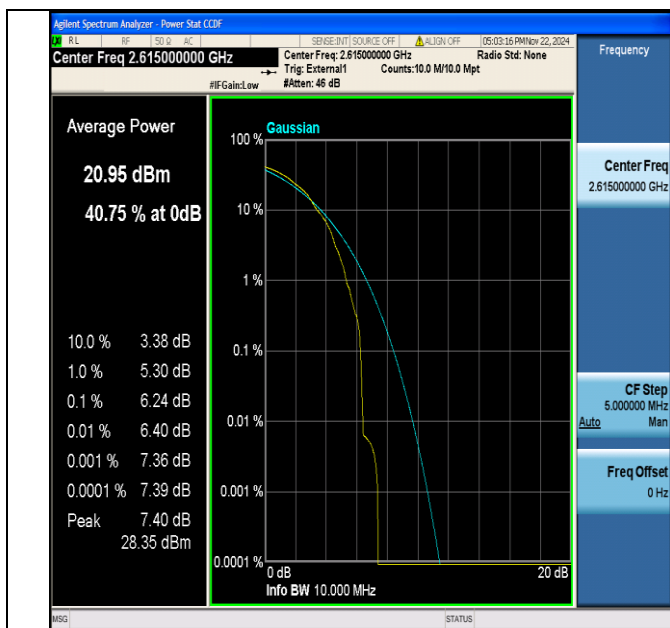
Band38-10MHz-64QAM-38200-1RB#0-PASS
