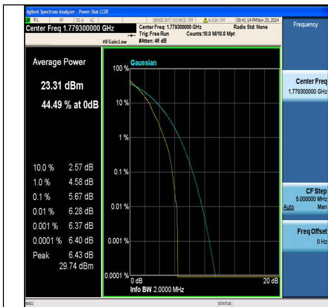
Band66-1.4MHz-QPSK-132665-1RB#0-PASS
