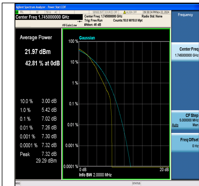
Band66-1.4MHz-64QAM-132322-1RB#0-PASS
