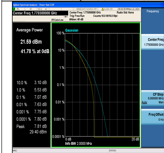
Band66-1.4MHz-64QAM-132665-1RB#0-PASS
