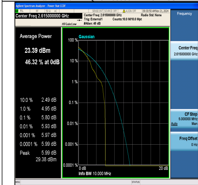
Band38-10MHz-QPSK-38200-1RB#0-PASS
