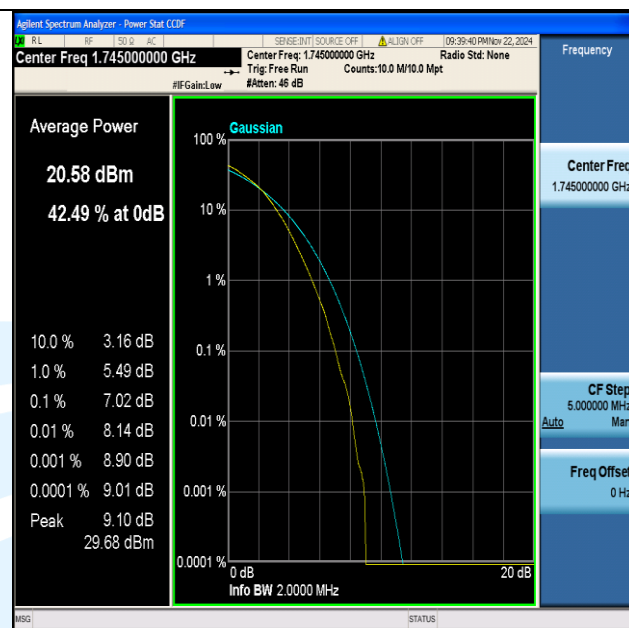
Band66-1.4MHz-64QAM-132322-6RB#0-PASS
