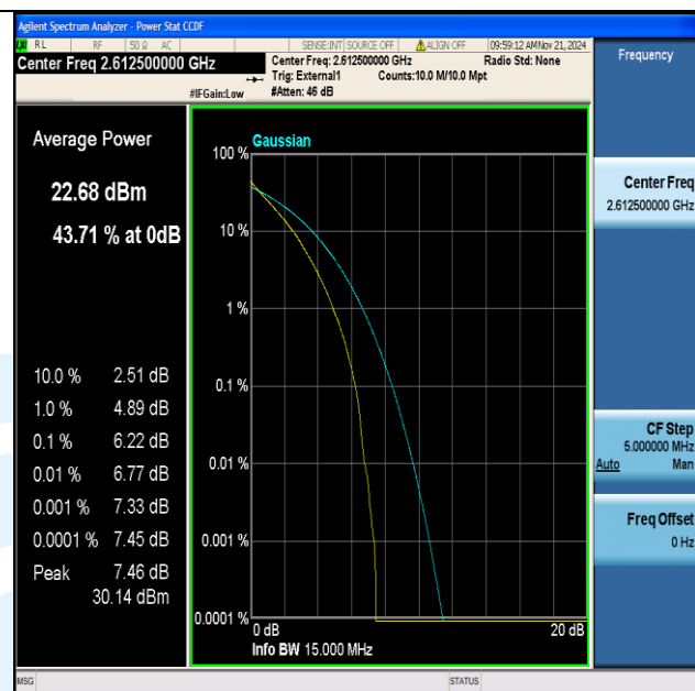
Band38-15MHz-QPSK-38175-75RB#0-PASS
