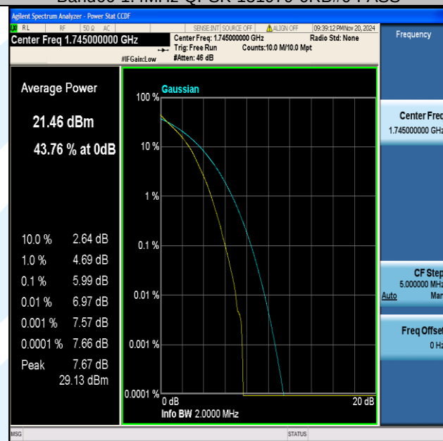
Band66-1.4MHz-QPSK-132322-6RB#0-PASS
