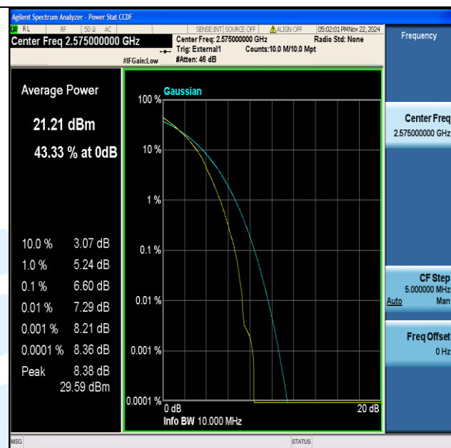
Band38-10MHz-64QAM-37800-50RB#0-PASS
