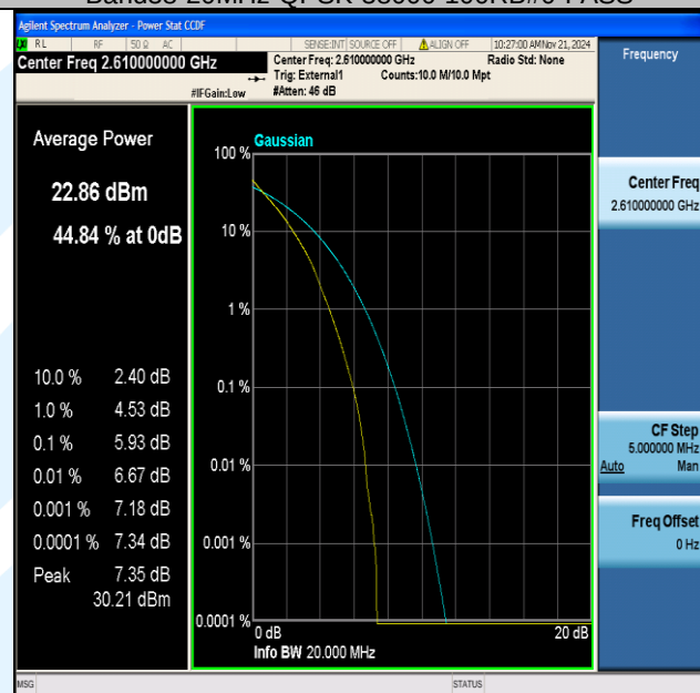
Band38-20MHz-QPSK-38150-100RB#0-PASS
