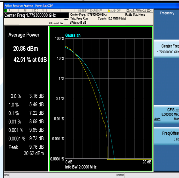
Band66-1.4MHz-64QAM-132665-6RB#0-PASS
