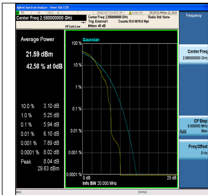
Band38-20MHz-64QAM-37850-1RB#0-PASS
