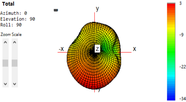
1900MHz 3D Antenna pattern
