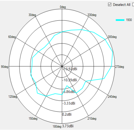
2D Antenna pattern (X->Y;X->Z;Y->Z)
