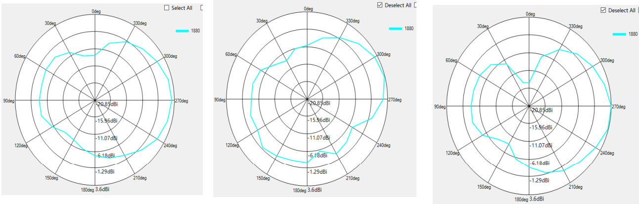
2D Antenna pattern (X->Y;X->Z;Y->Z)
