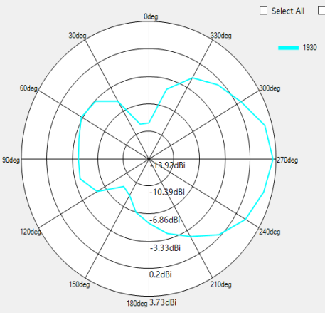
2D Antenna pattern (X->Y;X->Z;Y->Z)
