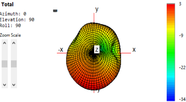
1880MHz 3D Antenna pattern
