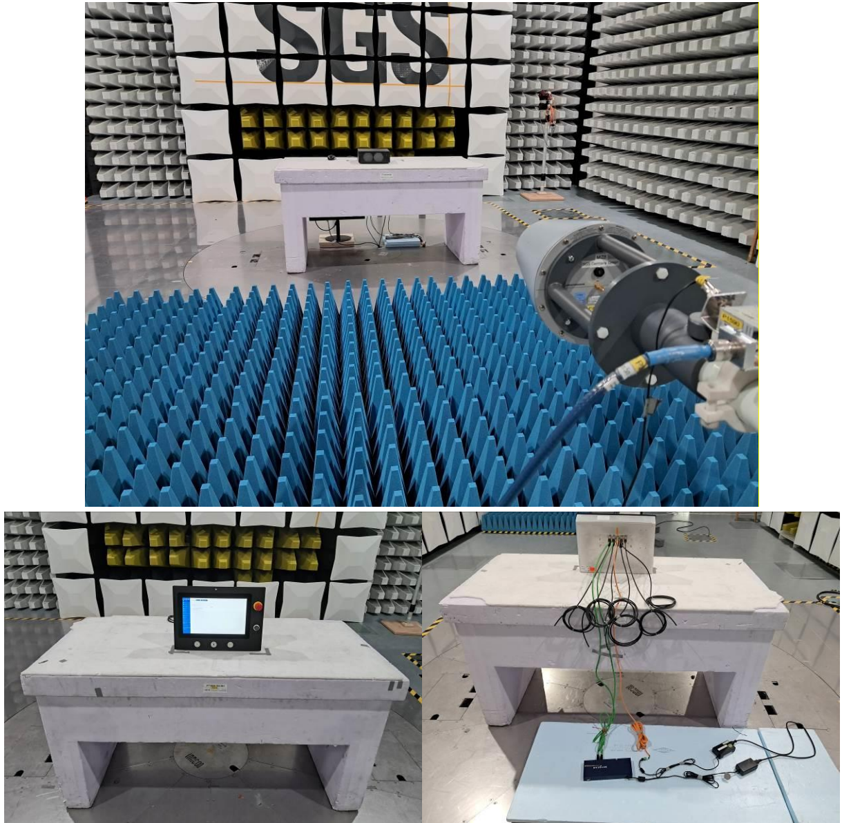
Figure 6-6: test setup for radiated disturbances 1 GHz to 18 GHz
