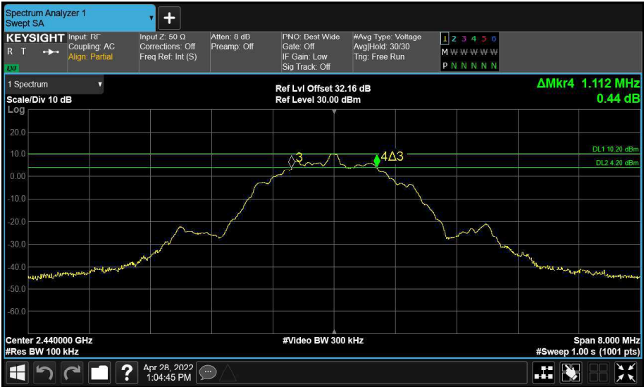
Figure 16 - Main (A) 2440 MHz (CH17) 6 dB Bandwidth
