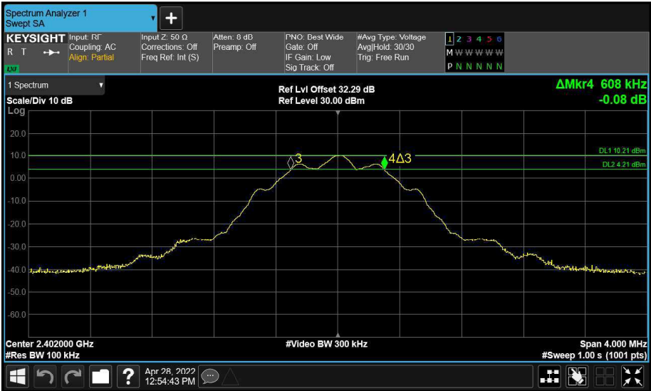
Figure 20 - Main (A) 2402 MHz (CH37) 6 dB Bandwidth
