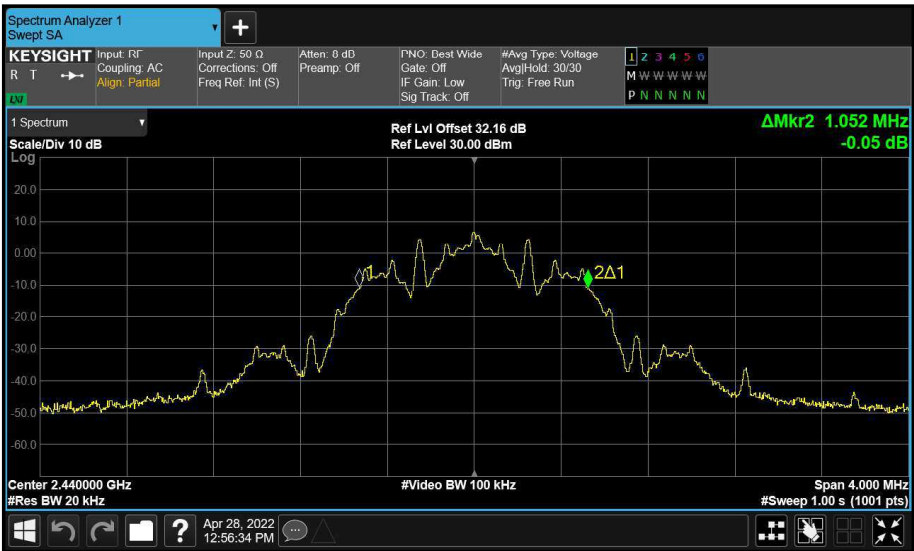
Figure 21 - Main (A) 2440 MHz (CH17) 99% Bandwidth
