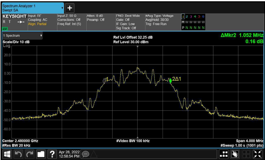
Figure 23 - Main (A) 2480 MHz (CH39) 99% Bandwidth
