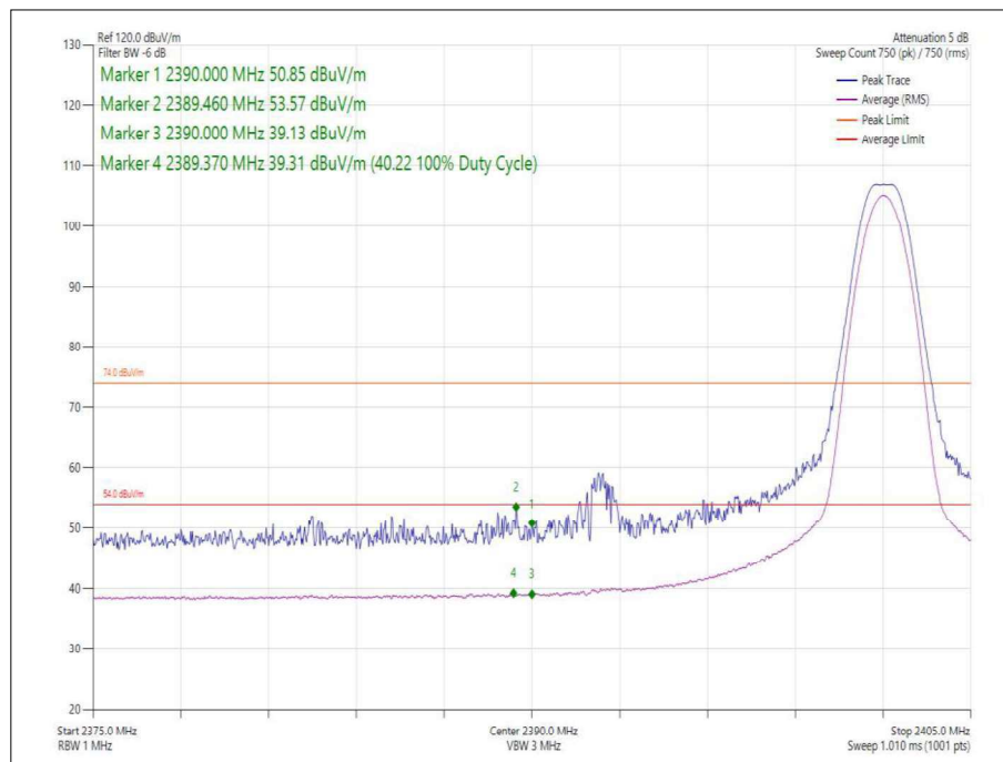
Figure 3 - GFSK (LE 8-Coding) - 2402 MHz - Band Edge Frequency 2390 MHz
