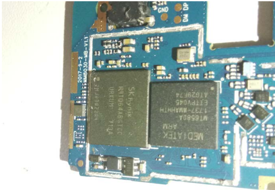
EUT – Main Chip 4 View
