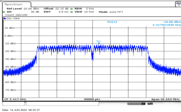
11G-CDD_Ant3_2417
