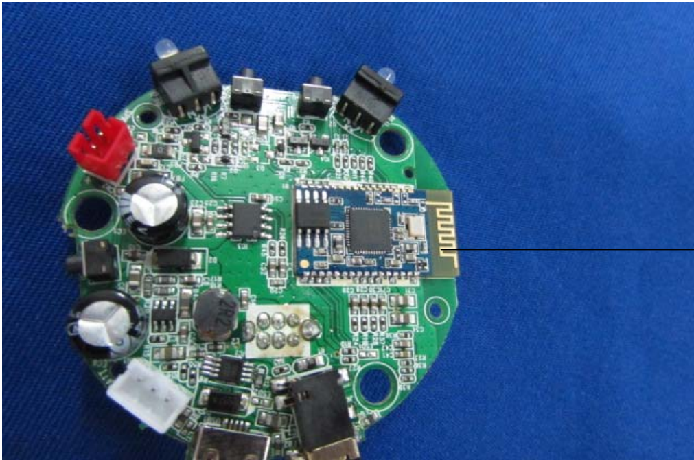
Bluetooth Antenna
