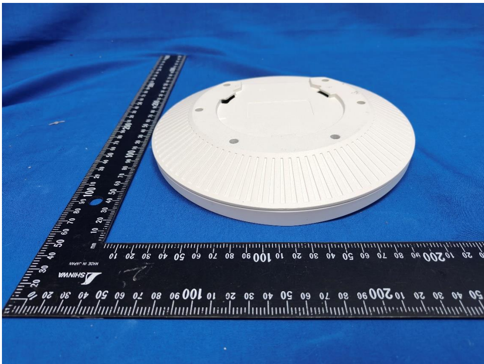
(4) EUT Photo (Model name: Festa F76) – Front View
