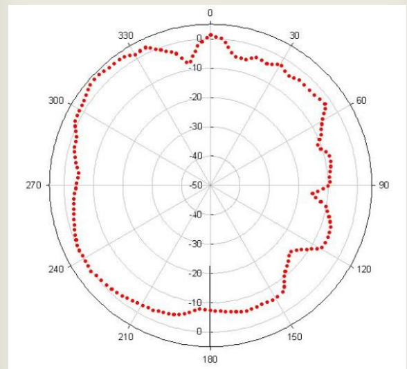
[Elevation1 plane @5.5GHz ]
