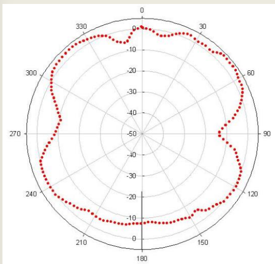
[Elevation2 plane @5.5GHz ]
