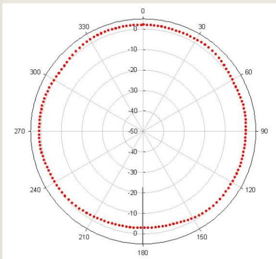
[Azimuth plane @2.442GHz ]
