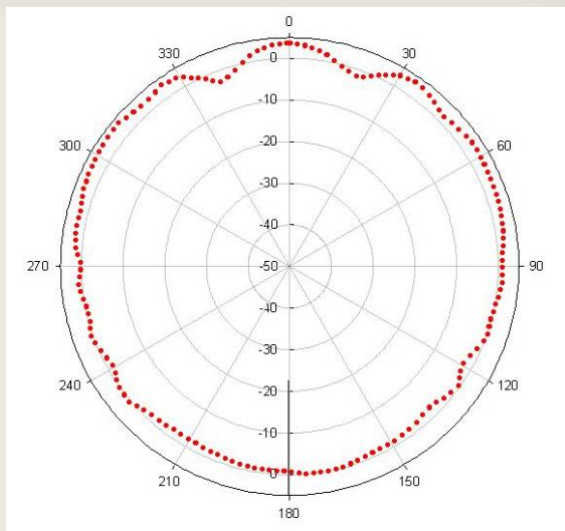
[Elevation2 plane @2.442GHz ]
