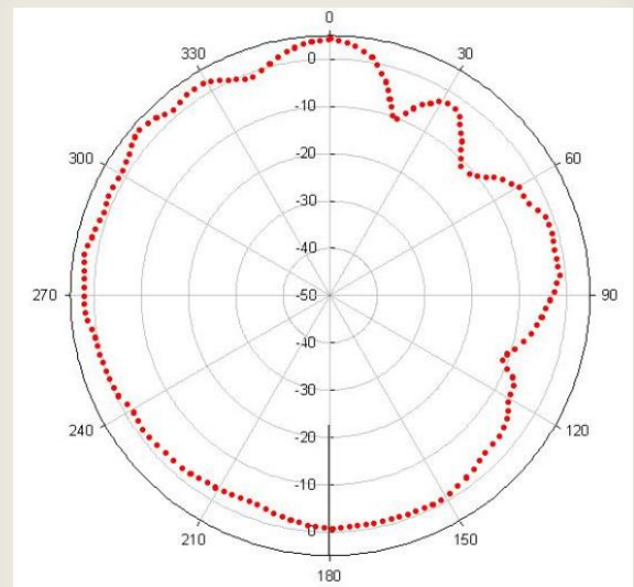
[Elevation1 plane @2.442GHz ]
