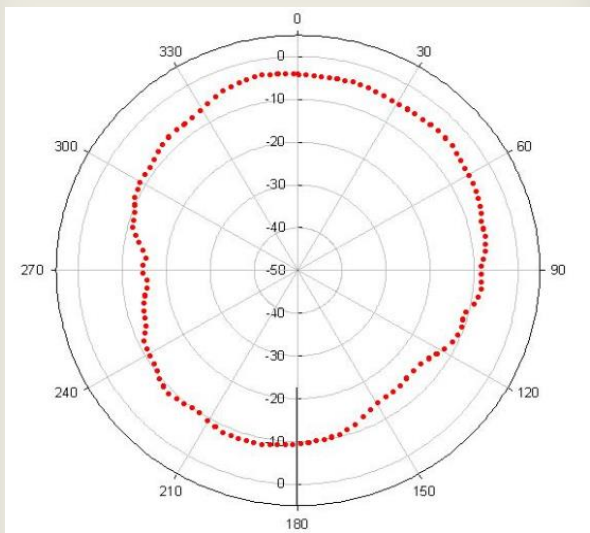
[Azimuth plane @5.5GHz ]
