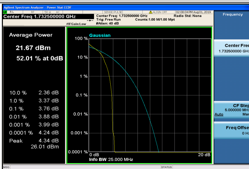
Band4-20MHz-QPSK-20175-1RB#0
