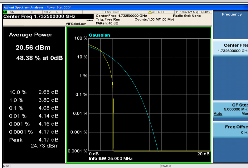
Band4-5MHz-16QAM-20175-1RB#0
