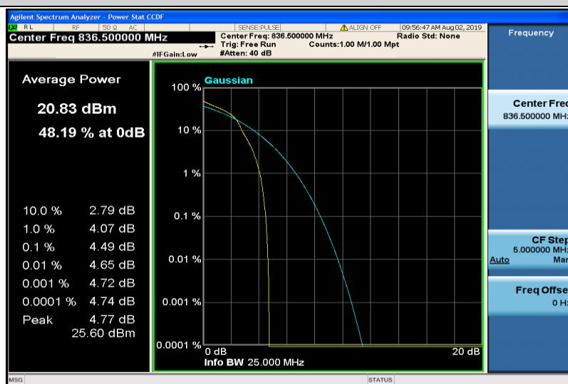
Band5-3MHz-16QAM-20525-1RB#0
