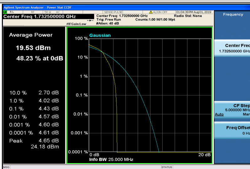
Band4-10MHz-16QAM-20175-1RB#0
