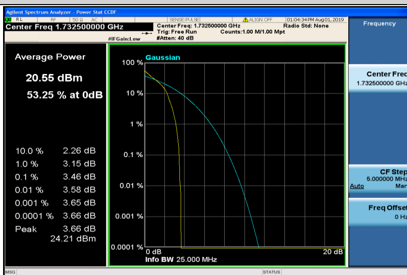
Band4-10MHz-QPSK-20175-1RB#0
