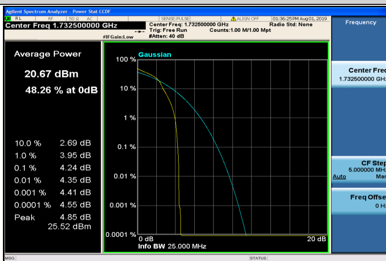
Band4-15MHz-16QAM-20175-1RB#0
