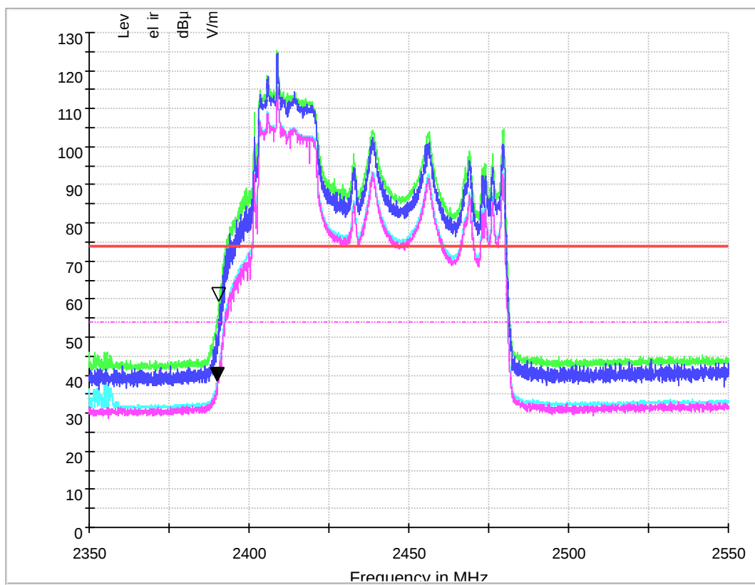
MEASUREMENT RESULT: PK Detector
